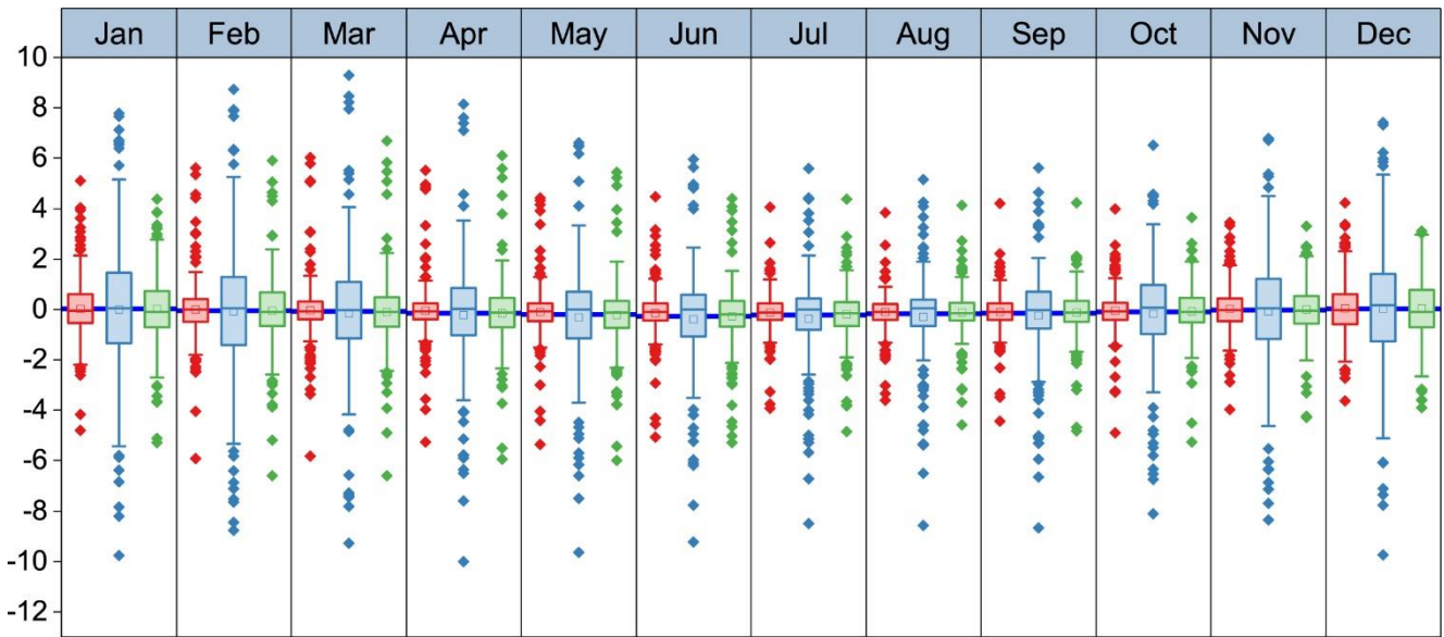
Figure 4: Residuals of the monthly Tmean predicted by the machine learning models with respect to in situ Tmean for the test meteorological stations. Note that the average of the residuals of Tmean from 1951–2020 for each test meteorological station is shown for each month. See Figure S6 and Figure S7 for the residual graph of Tmax and Tmin.
