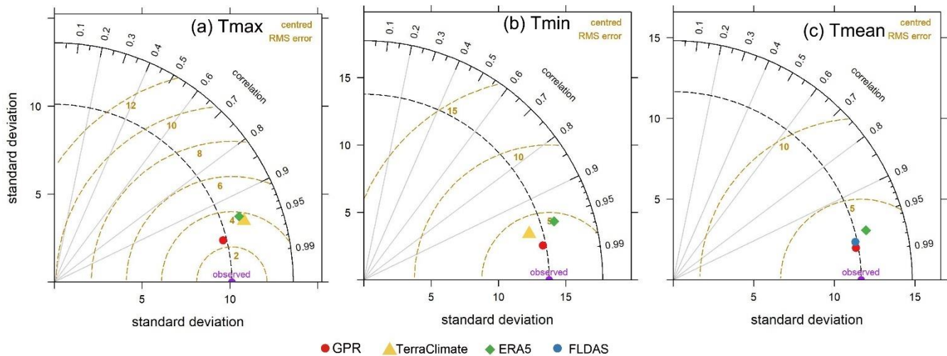
Figure 11: Taylor diagrams displaying a statistical comparison with observations between our products generated using the GPR model and the other products under the same spatial resolution. Given the overlapping time of the datasets, January 1979 to December 2019 was used for comparing Tmax and Tmin and January 1982 to December 2019 was used for comparing Tmean. Comparisons for each month are presented in the Supplementary Material (Figures S73–S75).
