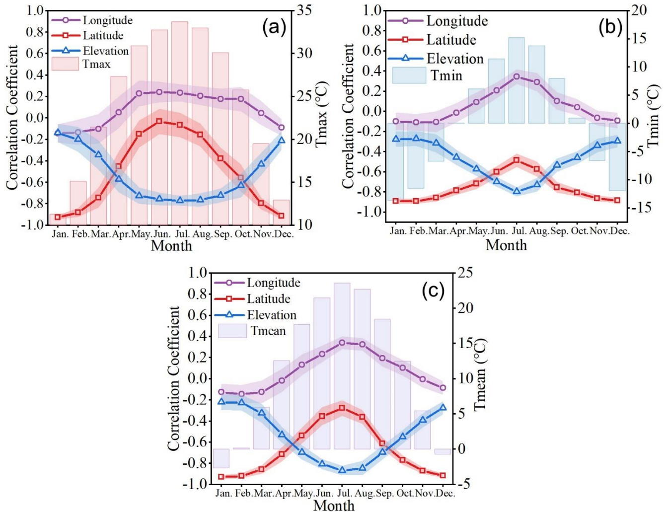
165 Figure 2: Correlation coefficients between (a) monthly maximum air temperature (Tmax), (b) minimum air temperature (Tmin), and (c) mean air temperature (Tmean) and longitude, latitude, and elevation for each month. Coloured shading indicates the standard deviation. Note that the correlation coefficients are the average values of the correlation coefficients for each month over 70 years (1951–2020).
