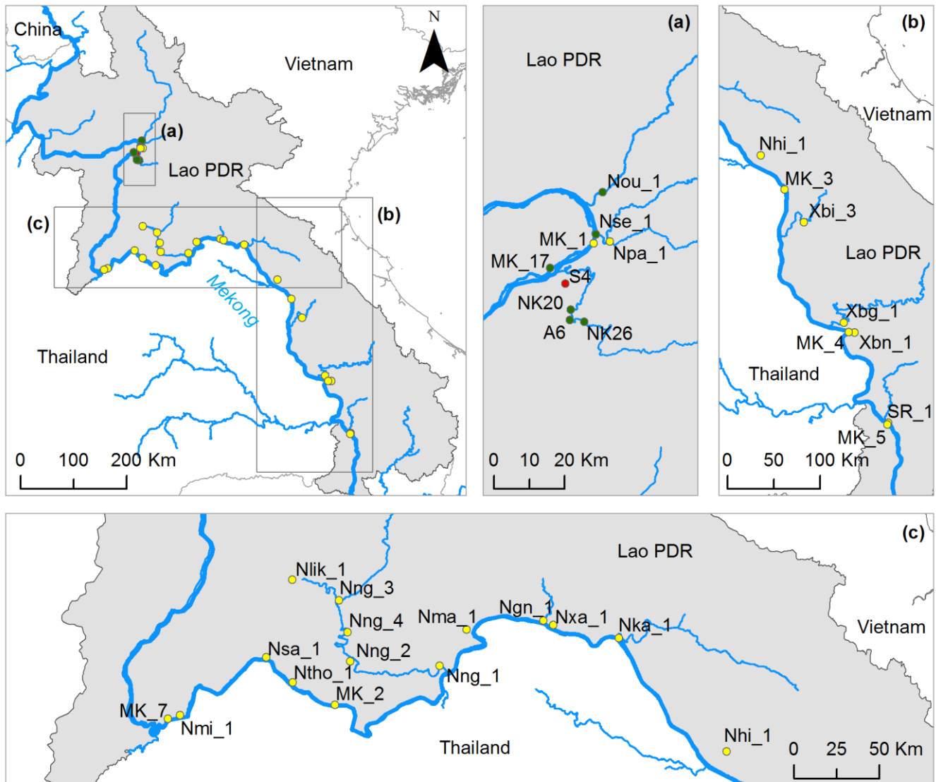
375 Figure 1: Location of the 31 sampling stations within the Mekong river basin in Lao PDR. Tributary names and catchment areas are given in Table 1. Red dot represents sampling station S4 and green dots represent sampling stations NK20, NK26, A6, Nou_1, Nse_1, and MK_17.
