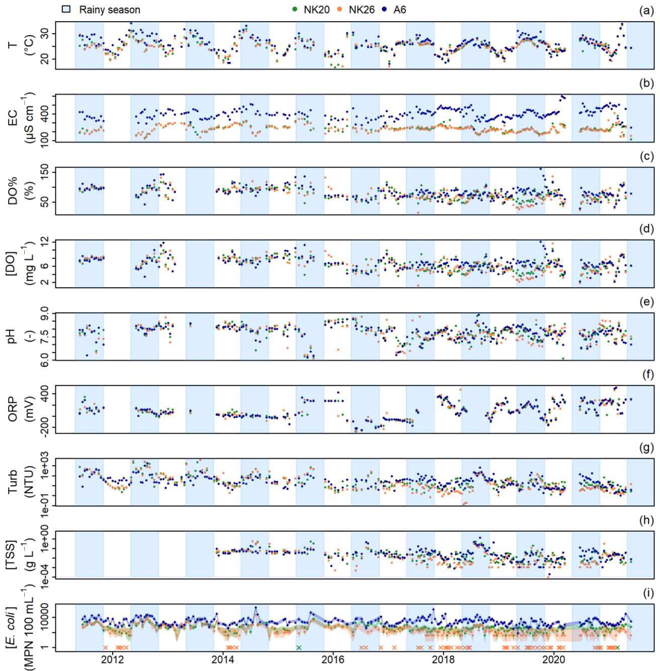
Figure 3: Stream water quality from 2011 to 2021 along the Nam Khan river (sampling stations NK20 and NK26) and its tributary Houay Khan (sampling station A6), northern Lao PDR. T: temperature ( ^{\circ}\text{C} ); EC: electrical conductance at 25^{\circ}\text{C} ( \mu\text{S cm}^{-1} ); DO%: oxygen saturation (%); [DO]: oxygen concentration ( \text{mg L}^{-1} ); pH: pH (-); ORP: oxidation-reduction potential (mV); Turb: turbidity (NTU); [TSS]: total suspended sediment concentration ( \text{g L}^{-1} ); [ E. coli ]: Escherichia coli concentration ( \text{MPN } 100 \text{ mL}^{-1} ) with lower and upper limits of the confidence interval given by Poisson distribution using the standardized microplate method. Turb, [TSS], and [ E. coli ] are shown with Y-axis as log scale. We added 0.0001 and 1 to all [TSS] and [ E. coli ] values, respectively, to present 0-
