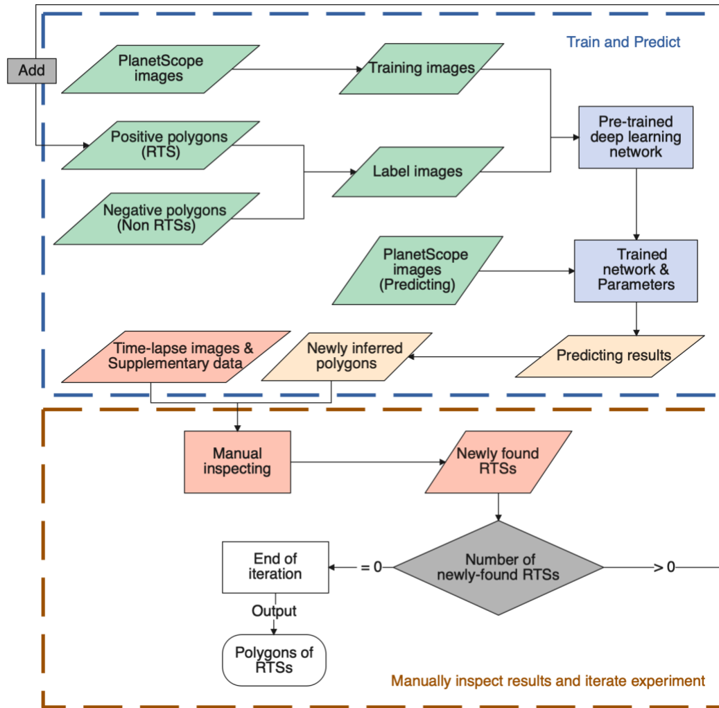
140 Figure 2. Workflow of the deep-learning-aided semi-automatic method.
