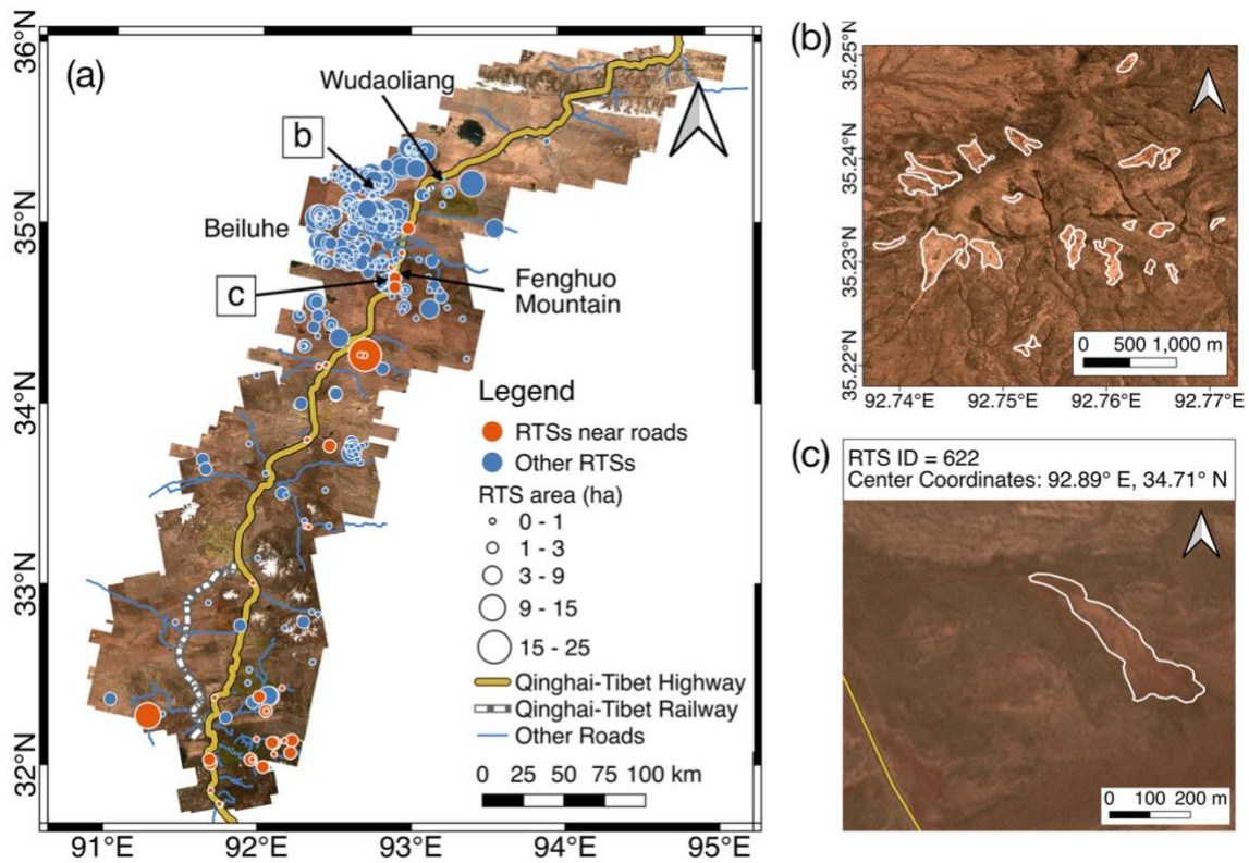
205 Figure 5. (a) The map of the 875 delineated RTSs. The circle sizes indicate the RTSs' area. Orange circles are RTSs close to roads, while blue circles show other RTSs. (b) Examples of the delineated RTSs in the Beiluhe region, with the white polygons representing the boundaries of RTSs. (c) An example of an RTS adjacent to the Qinghai-Tibet Highway (yellow line). Basemap images © Planet Labs Inc.
