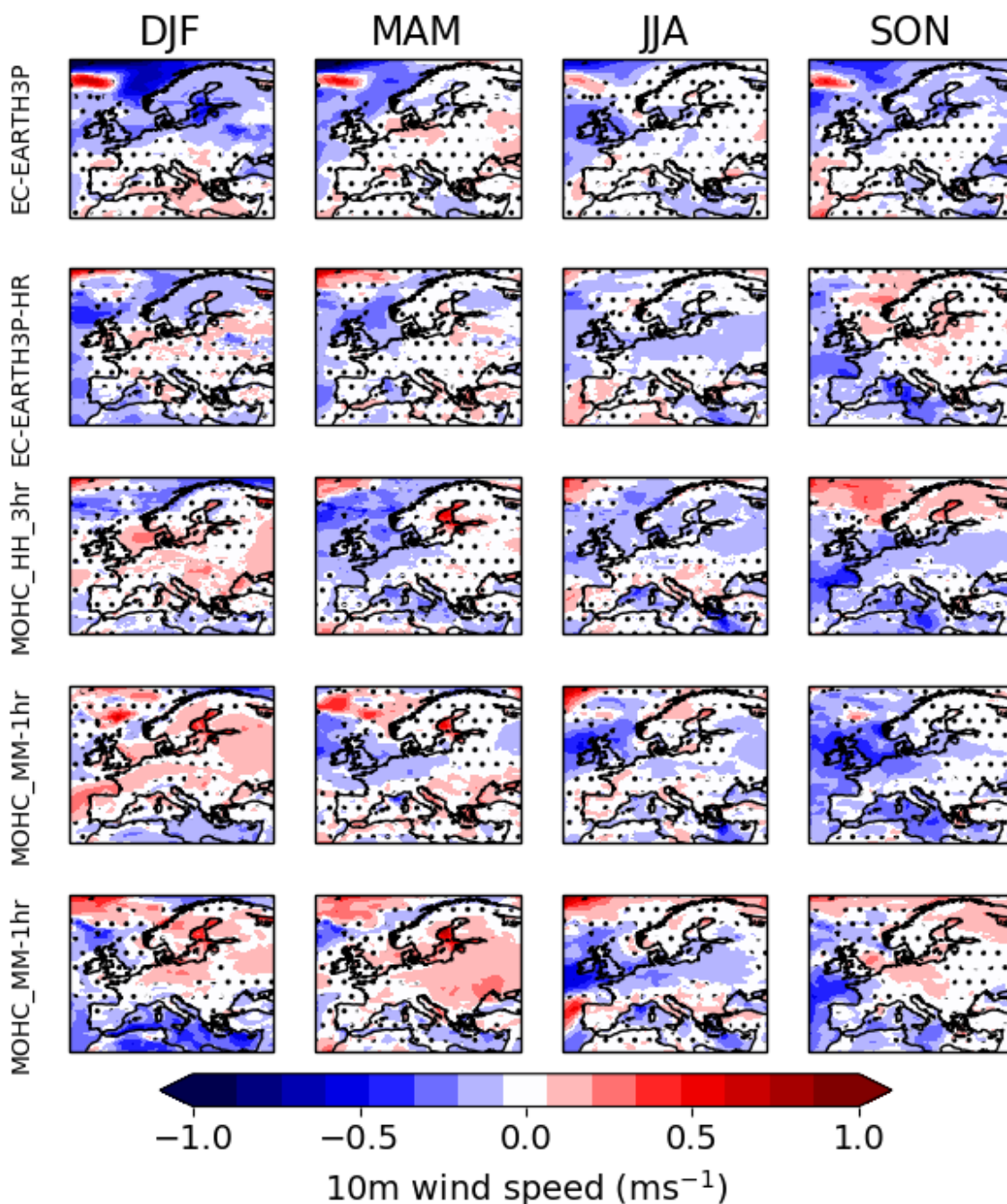
Figure A2. Seasonal-mean difference in 10m wind speed between 1980-2010 and 2020-2050 for the 5 different climate model simulations used in this study (see Table 1 for further details of the models). Stippling shows grid points where no statistically significant climate change signal was found when using a 2-sample t-test (Wilks, 2011).
