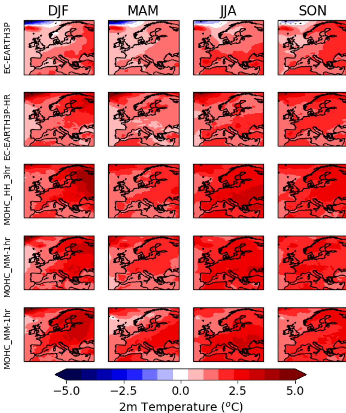
Figure A1. Seasonal-mean difference in 2m temperature between 1980-2010 and 2020-2050 for the 5 different climate model simulations used in this study (see Table 1 for further details of the models). Stippling shows grid points where no statistically significant climate change signal was found when using a 2-sample t-test (Wilks, 2011).
