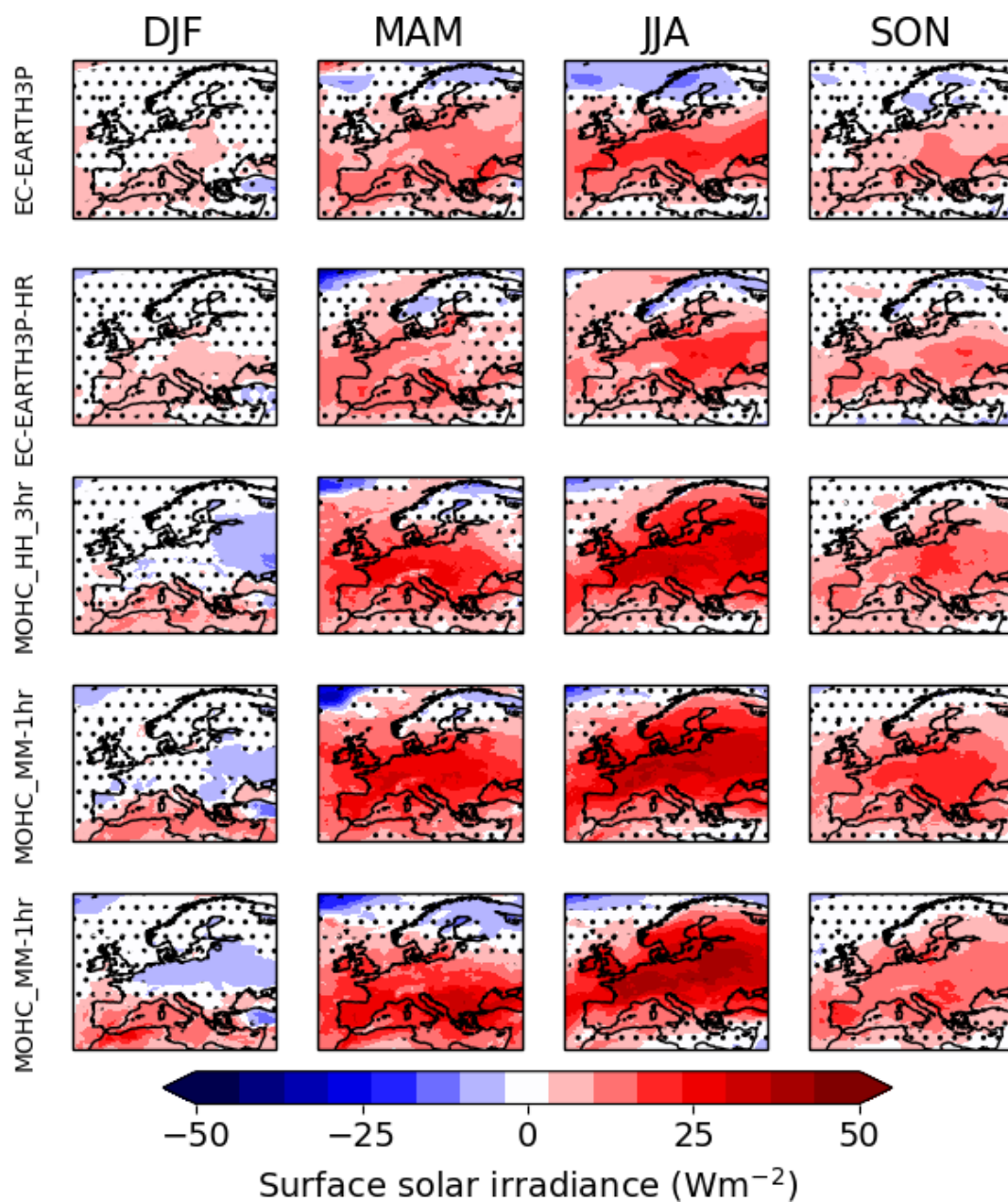
Figure 3. Seasonal-mean difference in surface solar irradiance between 1980-2010 and 2020-2050 for the 5 different climate model simulations used in this study (see Table 1 for further details of the models). Stippling shows grid points where no statistically significant climate change signal was found when using a 2-sample t-test (Wilks, 2011).
