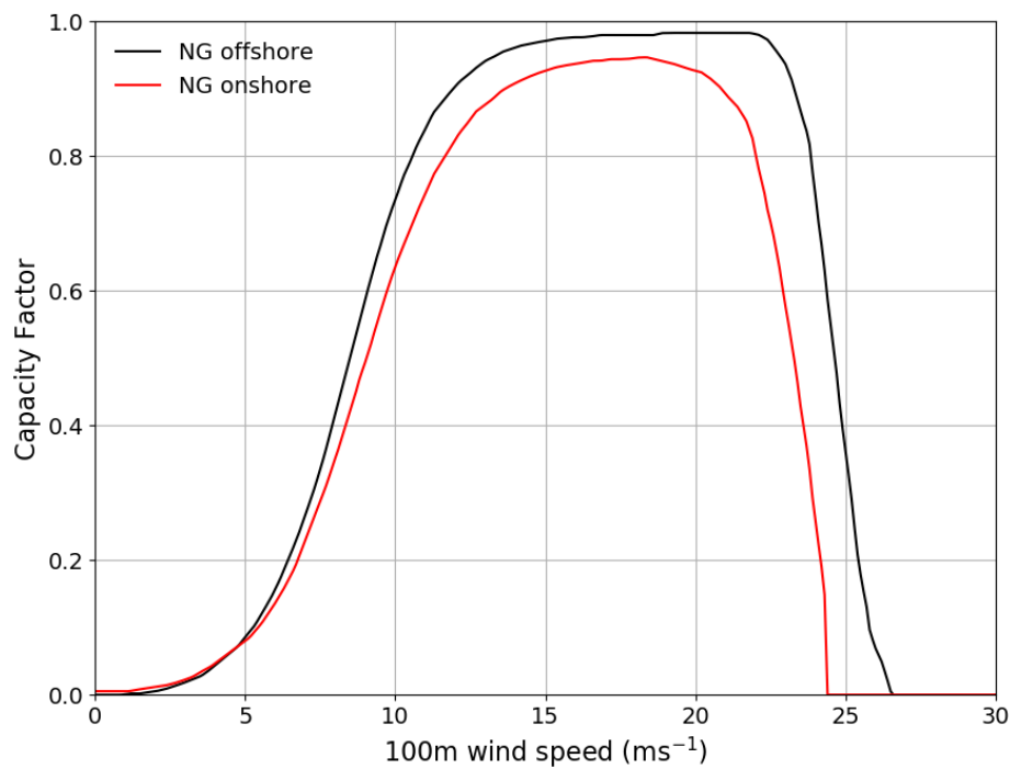
Figure 5. The onshore (red) and offshore (black) wind power curves used in this study, taken from National Grid
