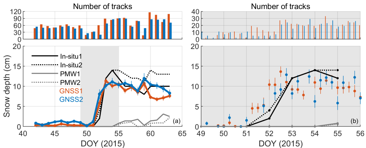
Figure 16. Performance of the GNSS snow depth on a snow event. (a) Daily data; (b) Two-hour data. Two 575 GPS/GLONASS compatible sites, i.e., bfqe (in red) and btll (in blue), are used to draw this figure. The error bar of each point in the figure is the standard error (STE) of the snow depths for all the available tracks of this point.
