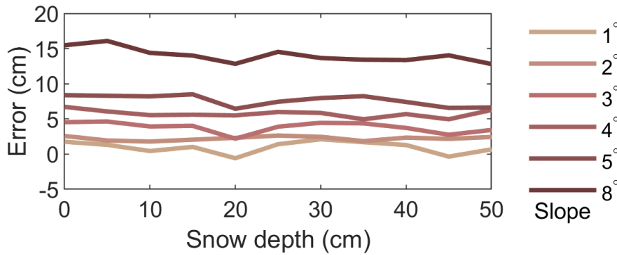
640 Figure 18. Simulations of the effects of terrain slopes on snow depth retrievals for a 2-m antenna height of GPS L1 (wavelength = 19 cm)
