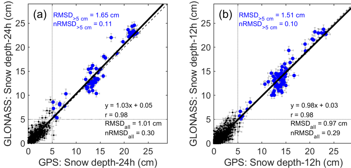
425 Figure 9. Correlations of 24 h/12 h snow depths from GPS and GLONASS observations. (a) 24 h; (b) 12 h. The error bar of each point is the standard error (STE) of the snow depths for all the available tracks of this point. Four available sites, i.e., hltl, hlhl, bfqe, and btll, during the GPS/GLONASS overlapped periods (i.e., the year 2014 and 2015) are used to plot this figure. For each point in the figure, the number of valid observations is more than five. To prevent other possible effects besides the GNSS constellation, the STE of snow depths is less than 1 cm (90% for the 430 24 h data and 76% for the 12 h data). Blue points are with the retrieved GPS and GLONASS snow depths greater than 5 cm. RMSD: Root Mean Square Difference; nRMSD: normalized RMSD.
