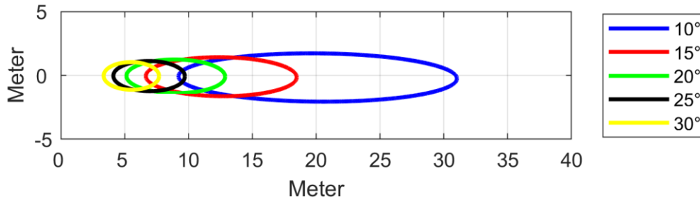
Figure 17. The footprint of the GNSS snow depth observation for a specific satellite track with different satellite 615 elevation angles.
