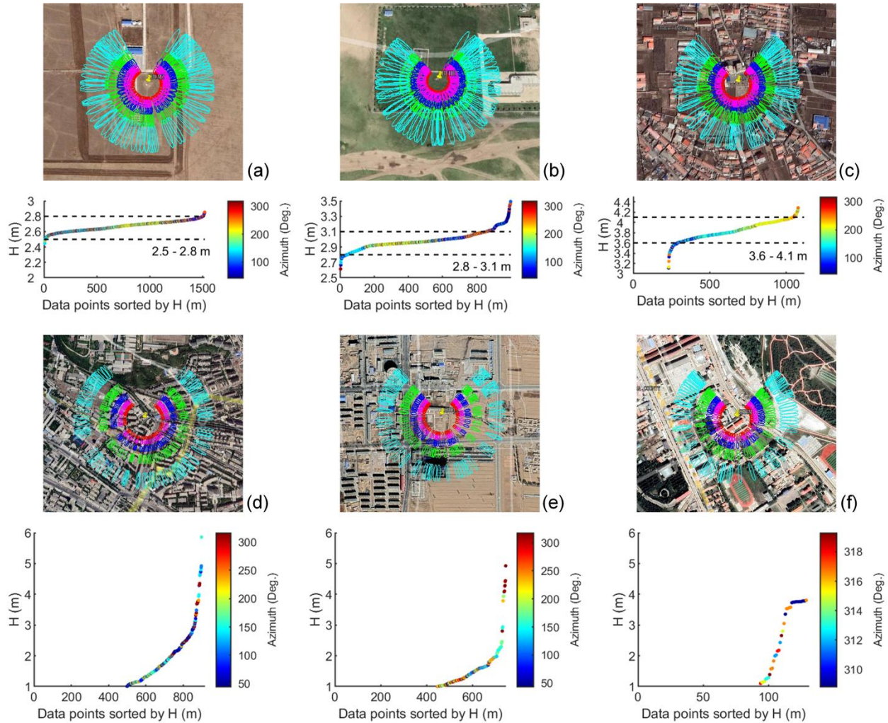
Figure 6. Examples show the high/medium-quality sites and the low-quality sites. High/medium-quality sites: (a) bumz, 2017; (b) bfhr, 2019; (c) bgfc, 2019; Low-quality sites: (d) uqw1, 2019; (e) qhdl, 2020; (f) qhbm, 2018. The top 325 image in each subfigure shows the footprint of the observation for elevation angles of 10^\circ , 15^\circ , 20^\circ , 25^\circ , and 30^\circ , respectively. The bottom image in each subfigure shows the distribution of the reflector heights for snow-free surfaces calculated from 10-days of observations using the SNR model. The background of this figure is from Google Earth ( https://earth.google.com/web/ ) © Google Earth 2021.
