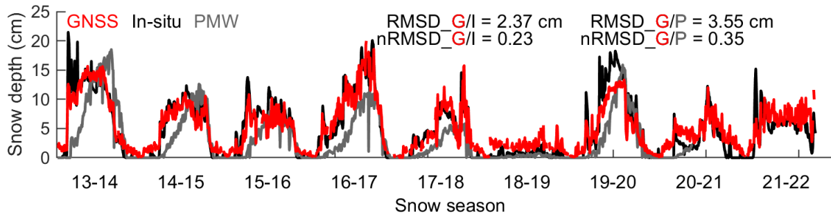
505 Figure 13. Comparisons of daily mean snow depth derived from GNSS, in-situ, and PMW for 17 GNSS sites with the most extended temporal coverage (i.e., from 2013 to 2022). RMSD: Root Mean Square Difference; nRMSD: normalized RMSD.
