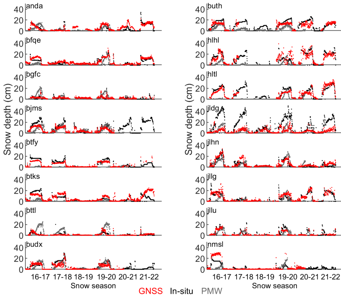
495 Figure 12. Comparisons of daily snow depth derived from GNSS, in-situ, and PMW. The data used in this figure is from 16 GNSS sites in 2016-2022, with the least missing daily snow depth values.
