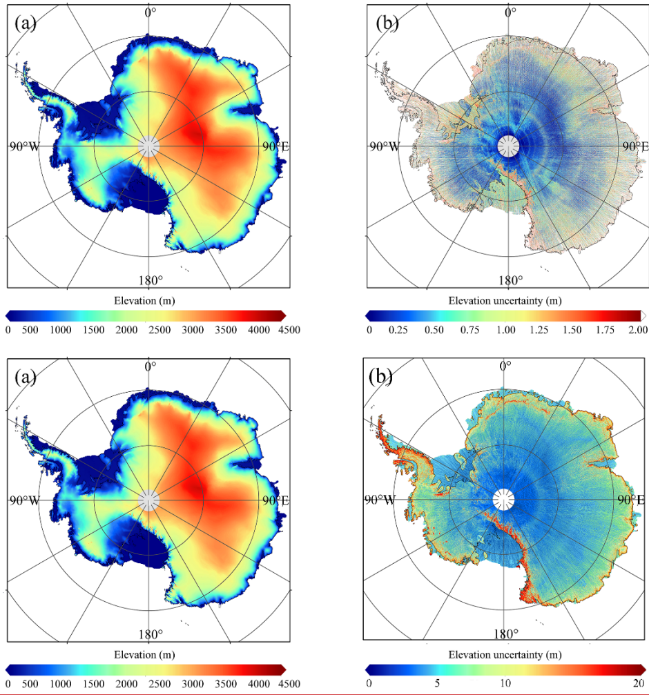
Figure 5. (a) A new DEM of Antarctica at a posting of 500 m derived from ICESat-2, which covers both the ice sheet and ice shelves with the southern limit of 88°S. (b) Map of the ICESat-2 DEM elevation uncertainty.
