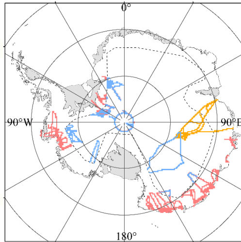
125 Figure 1. Maps of the OIB airborne data in October and November 2018 and October and November 2019 (red), from 2009 to 2019 in ice sheet interior (blue). Map of the GNSS transects from 2001 to 2015 in Antarctica (yellow). The dashed lines show the boundary of region where we assume to have low elevation change, it is the mode mask boundary of CryoSat-2 LRM data in Antarctica.
