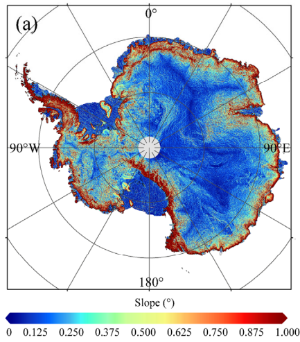
Figure 6. (a) Map of the surface slope of Antarctica derived from the ICESat-2 DEM. (b) Map of the ICESat-2 DEM surface slope uncertainty. The uncertainty is estimated based on the propagation of elevation uncertainty.
