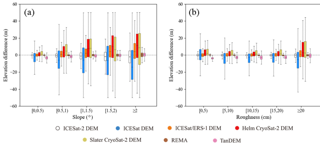
440 Figure 12. Median differences between seven DEMs and OIB airborne elevation measurements in areas of low elevation change from 2009 to 2019 with respect to surface slope and roughness. The upper and lower lines in each box indicate the 25th and 75th percentiles, the whiskers indicate the 5th and 95th percentiles, and the central horizontal line indicates the median difference.
