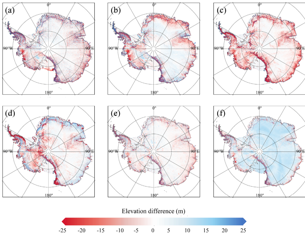
415 Figure 11. Elevation differences between the ICESat-2 DEM and six previously published DEMs, i.e., ICESat DEM (a), ICESat/ERS-1 DEM (b), Helm CryoSat-2 DEM (c), Slater CryoSat-2 DEM (d), REMA DEM (e) and TanDEM PolarDEM (f).
