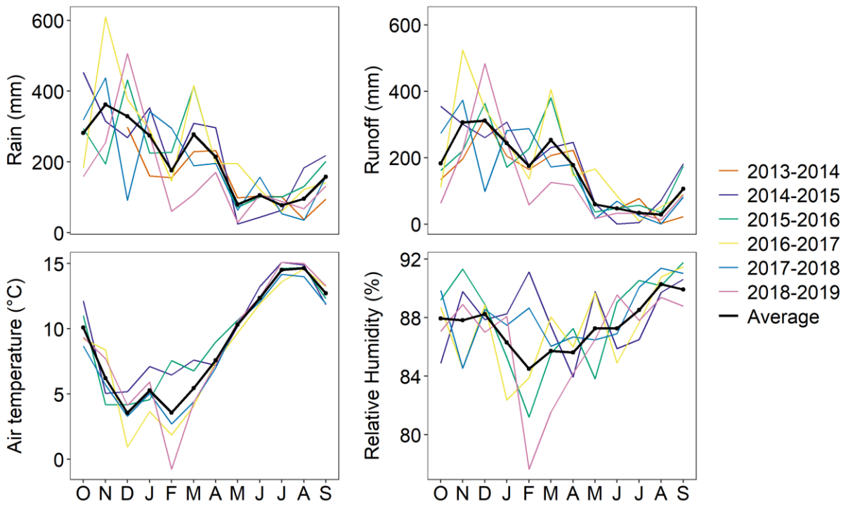
370 Figure 3: Seasonal rain, runoff, air temperature and relative humidity by water year. Monthly totals (rain, runoff) and monthly averages (air temperature, relative humidity) from station ‘SSN708’ are shown, the station with the longest record (installed September 2013, 12 m a.s.l.).
