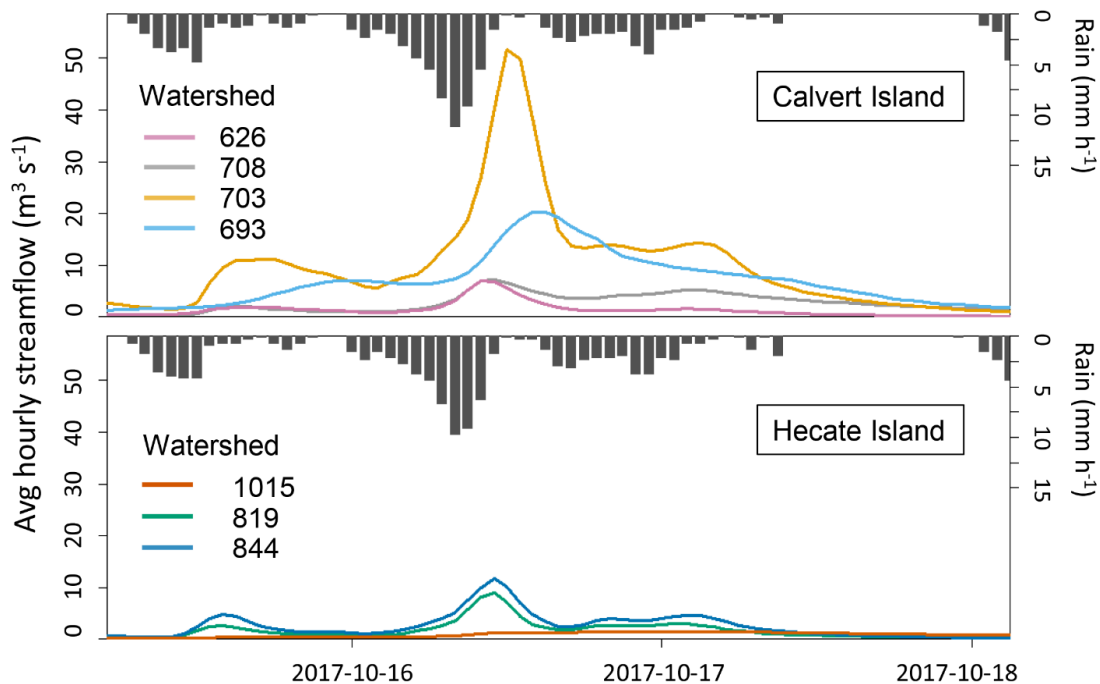
460 Figure 5: Hydro-hyetographs for the seven gauged watersheds during a large storm event (114 mm of rain in 3 days). Rain measured at ‘SSN708’ and ‘SSN819’.
