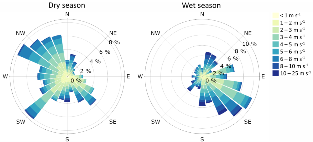
370 Figure 4: Average hourly wind speeds and wind directions during the dry (May-Sep) and the wet (Oct-Apr) meteorological seasons. Frequency of occurrence is indicated in % of time for the entire measurement record of ‘Hecate’ station (Oct 2015 – Oct 2019).
