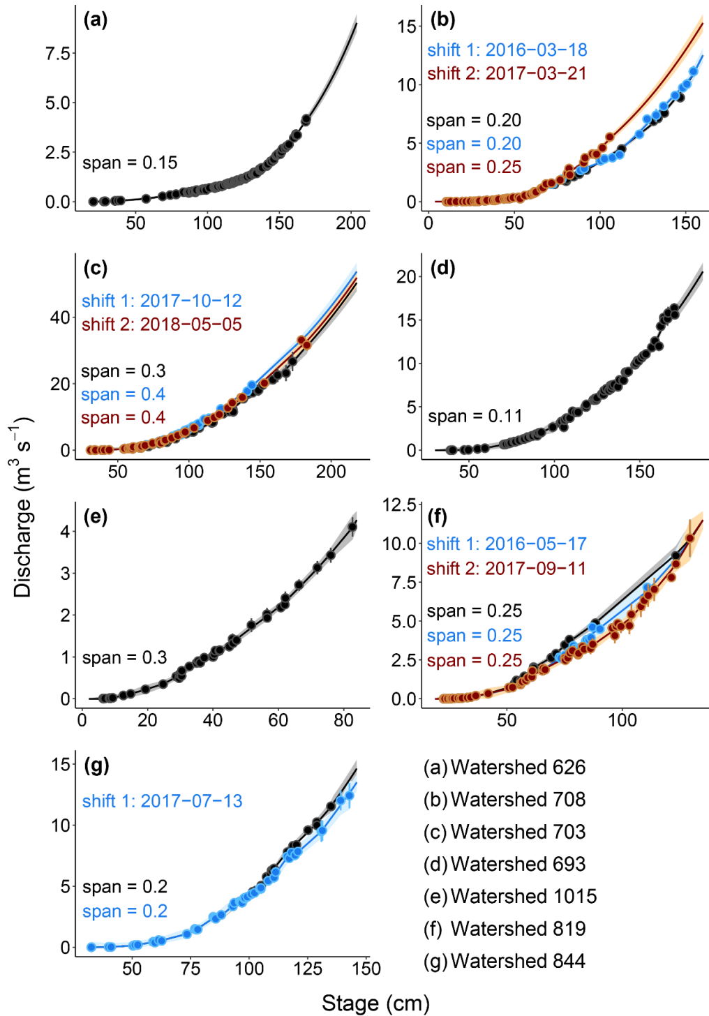
305 Figure 2: Stage-discharge rating curves with 95 % confidence bands for the seven gauged watersheds. Large storm events caused rating curves to shift at some of the watersheds; dates are indicated for each individual shift. Rating curves were plotted using LOESS regression and span widths ('span') were visually selected for each individual curve.
