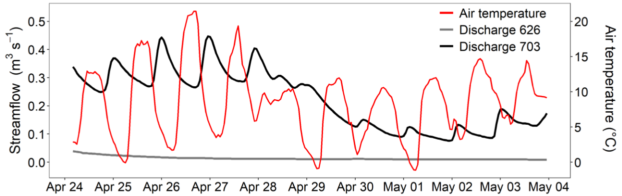
615 Figure A3: Discharge and air temperature at watershed 703 during 10 days without rainfall in the snowmelt season (measured at ‘SSN703’ and ‘WSN703’ respectively). Daily fluctuations in 703 streamflow indicate snowmelt contributions: peak flows occur ~12 h after daily maximum air temperatures. Discharge at watershed 626 (low elevation watershed with no snowpack), shown for reference: stable recession indicates no rainfall inputs during this period.
