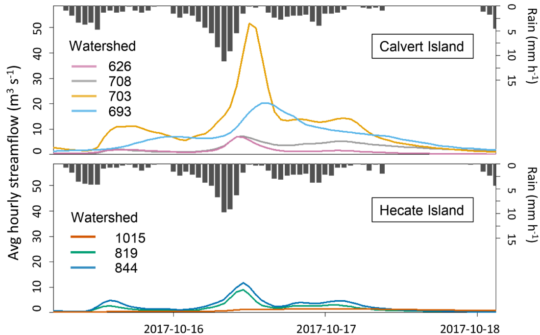
Figure 5: Hydro-hyetographs for the seven gauged watersheds during a large storm event (114 mm of rain in 3 days). Rain measured at ‘SSN708’ and ‘SSN819’.
