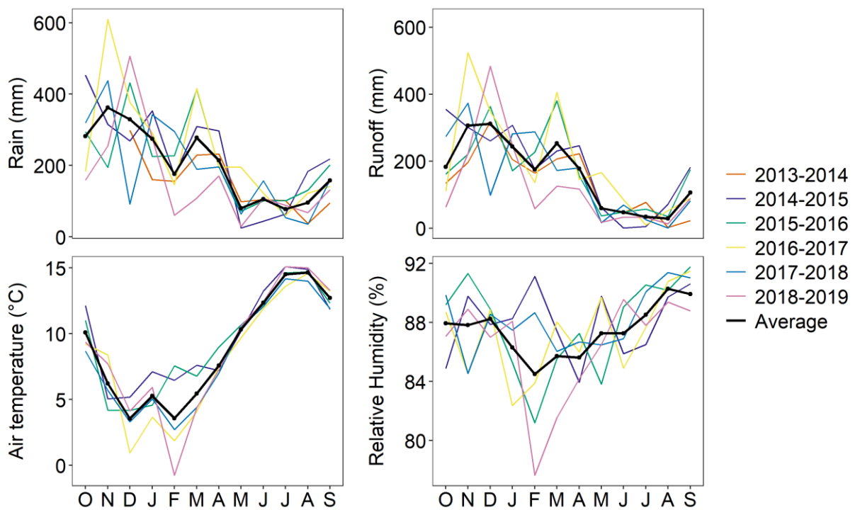
Figure 3: Seasonal rain, runoff, air temperature and relative humidity by water year. Monthly totals (rain, runoff) and monthly averages (air temperature, relative humidity) from station 'SSN708' are shown, the station with the longest record (installed September 2013, 12 m a.s.l.).
