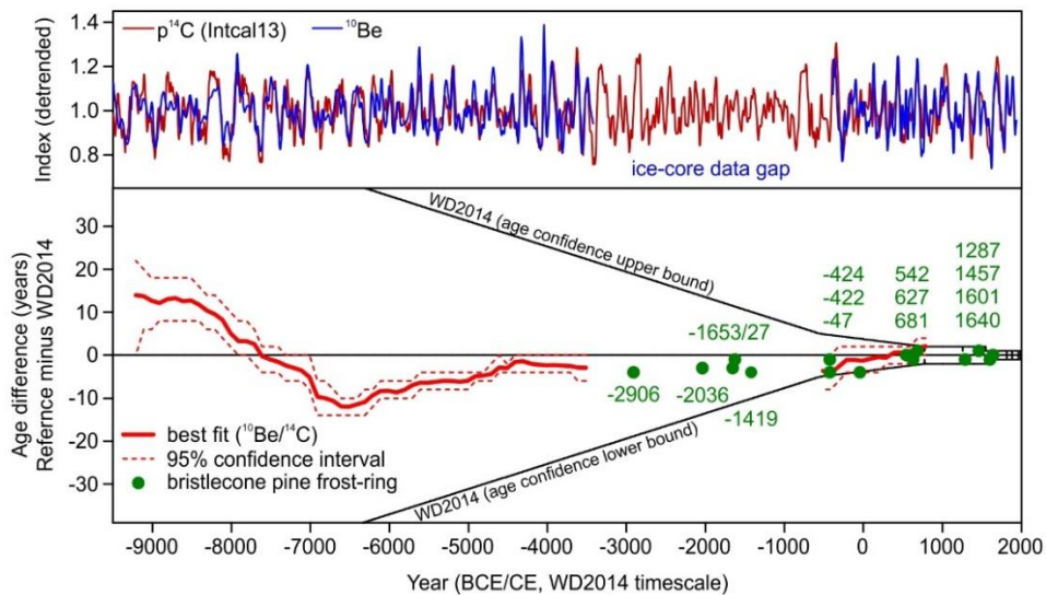
Figure 11: Estimated age uncertainty. Comparison of WD2014 to independent chronologies based on dendrochronology. Upper panel: filtered WD ^{10}\text{Be} (blue) and ^{14}\text{C} (red) tree-ring data on their respective timescales. Lower panel: most likely time shift (red line, 2 ka sliding window) for the highly significant correlations together with the 2\sigma uncertainty range (see Sigl et al., 2016, for details). Green circles mark the age difference between major reconstructed eruptions (VSSI >10 Tg) and cooling anomalies (i.e. co-occurrence of frost-ring and ring-width minima within \pm 1 year) in a 5 ka bristlecone pine chronology from the SW of the USA. A complete list of the selected event years are in the Supplementary Table S1 and Supplement Table S2 extracted from the compilation by Salzer and Hughes (2007).
