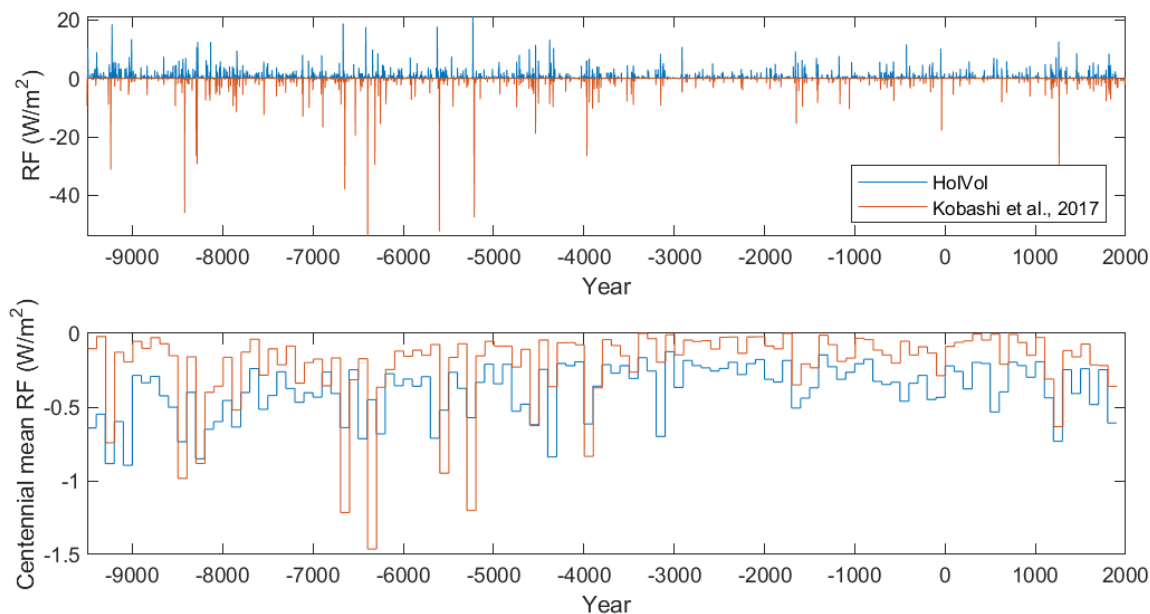
600 Figure 10: Upper panel: Global mean radiative forcing (RF) from the EVA(HolVol) reconstruction (inverted axis) and from a reconstruction based on the GISP2 ice-core (Kobashi et al., 2017). Lower panel: centennial mean RF for the two reconstructions.
