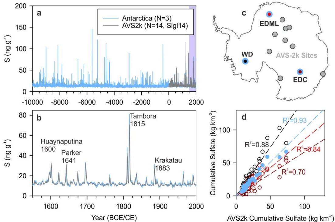
250 Figure 4: Representativeness, a: Mean annual sulfur concentrations from the ‘Antarctica’ stack ( ANT12k , N=3) over the Holocene compared to the ‘AVS2k’ stack from on average 14 ice cores from Antarctica over the Common Era (Sigl et al., 2014). The time period from 1550-2000 CE (purple shading) is displayed in b: with known large volcanic eruptions from the tropics highlighted; c: map of the ice core sites from Antarctica used in this and a previous study; d: scatterplot between cumulative volcanic sulfate mass deposition (‘flux’) for individual ice cores (WD, black; EDML, red, EDC dark red), the ‘Antarctica’ stack composite record (greenlight blue) and the ‘AVS2k’ stack. Included in the analysis are the 30 largest sulfate deposition events in ‘AVS2k’. 255
