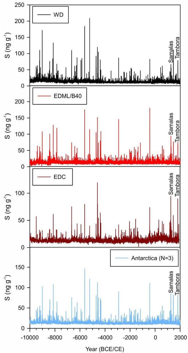
Figure 3: Holocene sulfur records from Antarctica; sulfur concentration record from WD, EDML, EDC ice cores and a stack ('Antarctica' or ANT12k) of all three records for the Holocene (10000 BCE – 2000 CE). Measured as sulfate, EDML and EDC records are synchronized on the WD2014 chronology (Sigl et al., 2016), annualized and scaled to the WD record. The upper part from EDML is based on the 200 m long B40 ice-core drilled at the same site in 2012 (Sigl et al., 2015). Signals from two large historic eruptions of Tambora (1815) and Samalas (1257) are marked.
