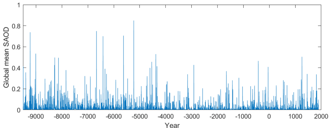
580 Figure 9: Global mean annual mean stratospheric aerosol optical depth (SAOD) from the EVA(HolVol) reconstruction. Years are shown using the ISO 8601 standard, which includes a year zero.
