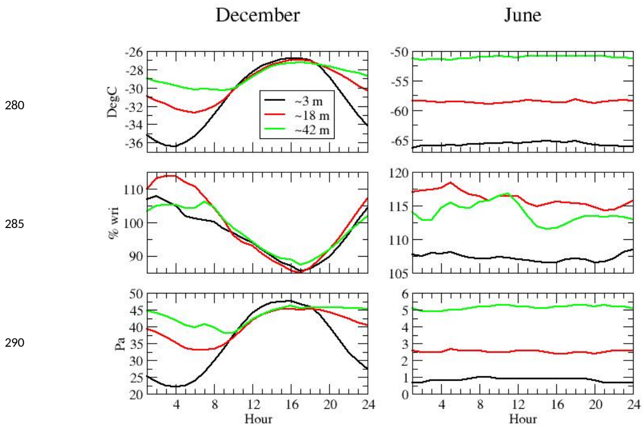
295 Figure 8: Mean 24-hour cycle of temperature (upper plots), RH i (middle plots) and PPW (lower plots) in December (at left) and June (at right) averaged over 2018-2020.
