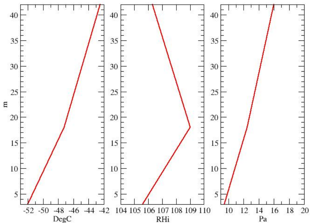
Figure 9: Annual mean vertical profile of temperature (left), RH (middle) and PPW (right) for observations made in 2018-2020.
