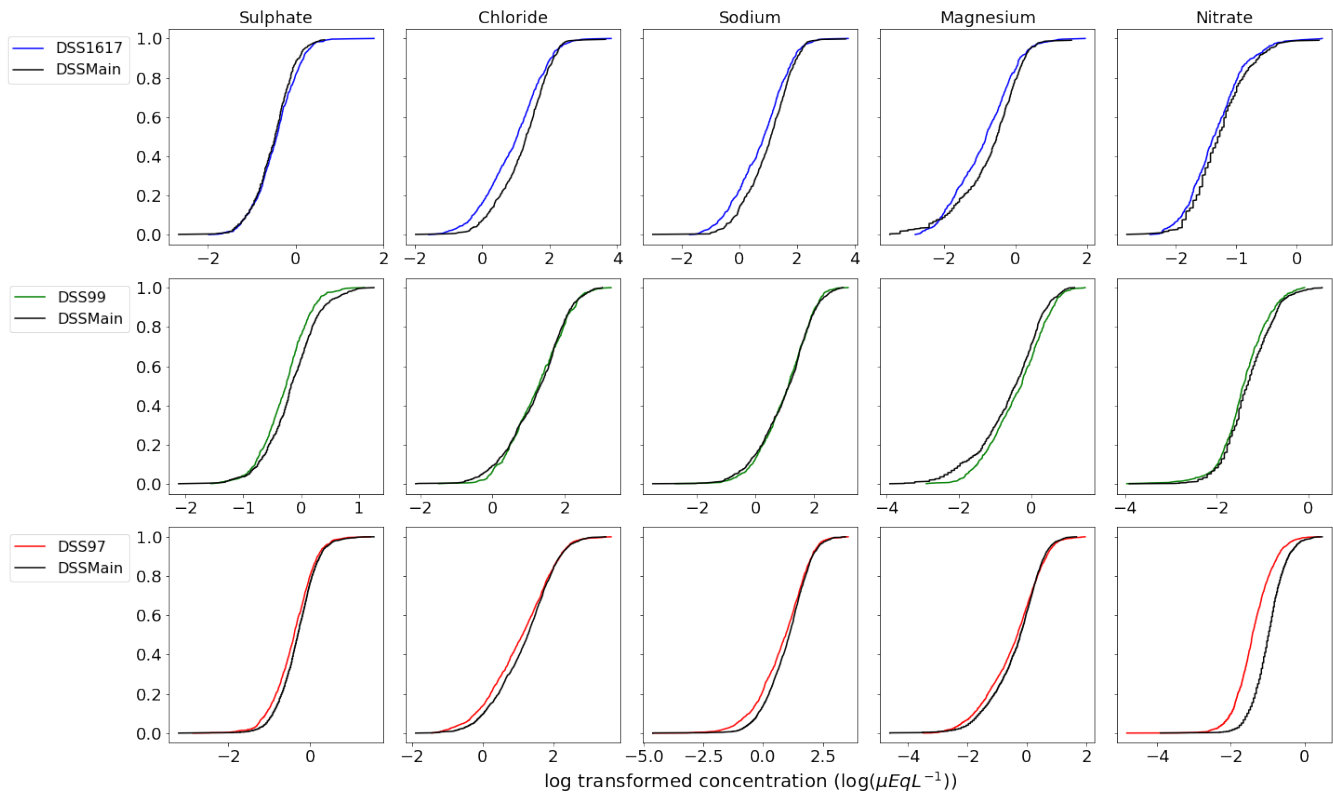
Figure A2. Empirical cumulative distribution functions of the log transformed concentration data for each trace chemistry species. Epochs from DSS1617, DSS99 and DSS97 are each compared against epochs from the DSSMain core with similar, but not identical, snow accumulation rates. Epochs are determined by the changepoint analysis on the CUSUM snow accumulation.
