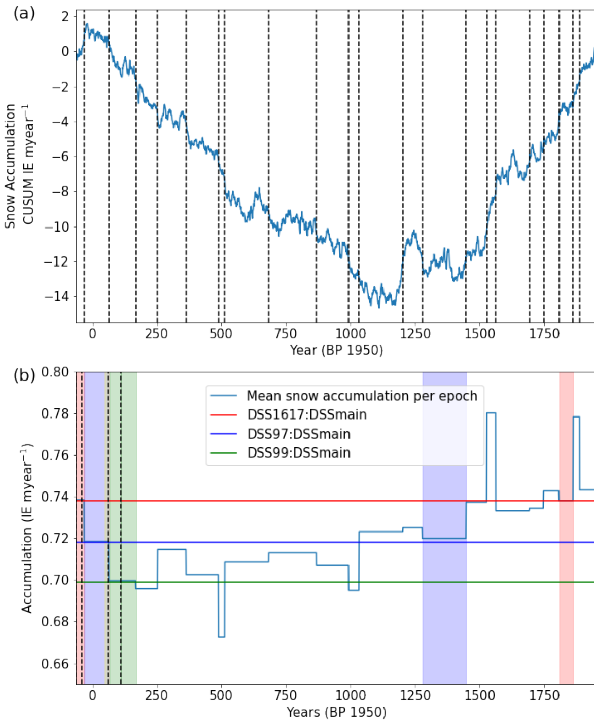
Figure A1. (a) Cumulative sum of the annual snow accumulation rate with detected change points indicated by vertical dashed lines. (b) Average snow accumulation epochs used for chemistry data statistical analysis.
