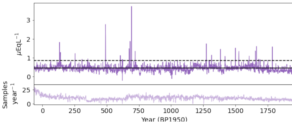
Figure 14. Time series for annually averaged non-sea salt sulphate. Solid black line indicates the 2000 year mean value. Dashed black line indicates 2\sigma value.
