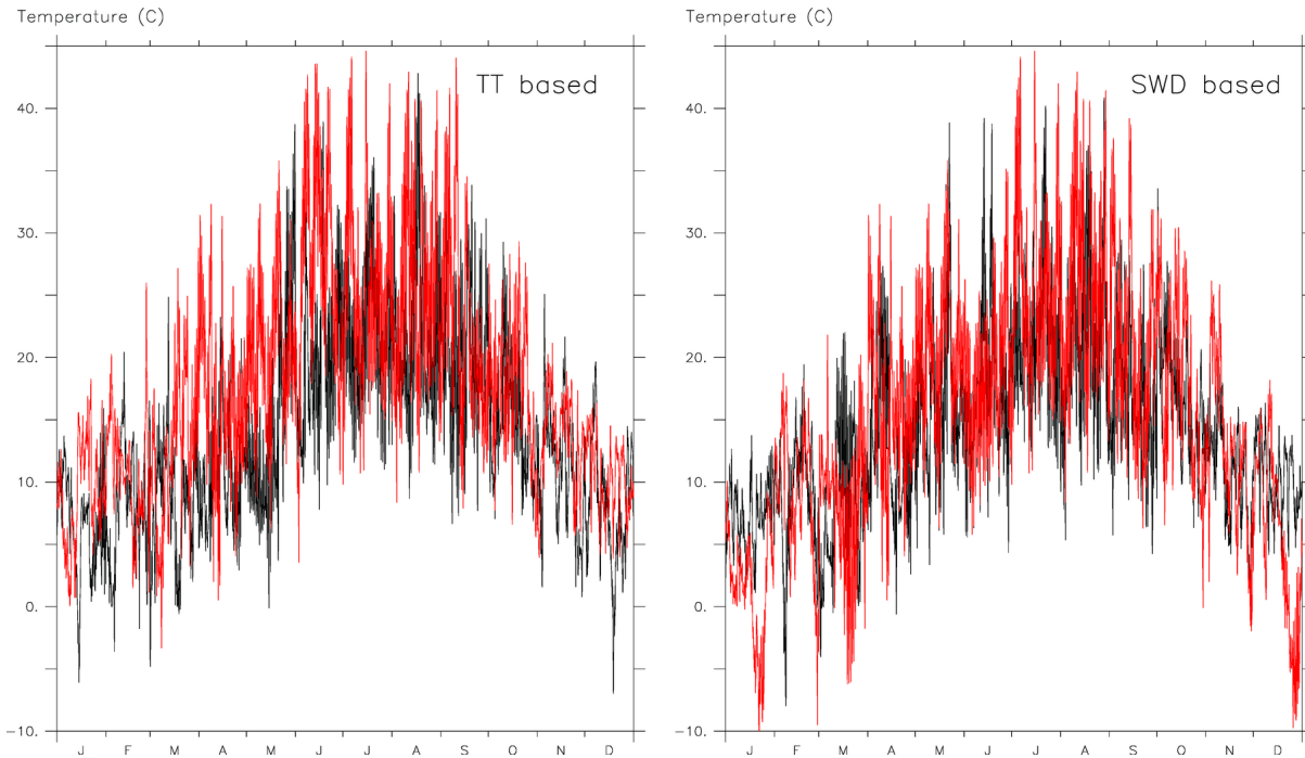
485 Figure A1: Typical (black) and extreme (red) temperature for Liege city simulated by MAR forced by BCC-CSM2-MR with the scenario SSP5-8.5 for the period 2085-2100. The typical/extreme months are based on temperature (left) and incoming solar radiation (right). These data are extracted from these files:
