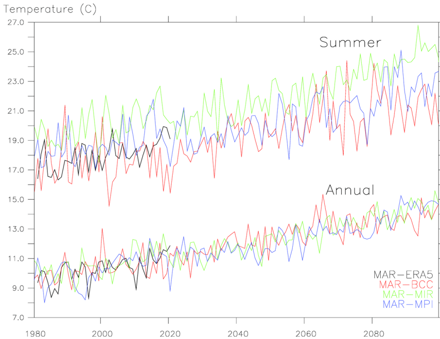
Figure 3: Annual mean temperature (in C, lower lines) and annual summer temperature (in C, upper lines) of MAR forced by ERA5 reanalysis (in black lines between 1980 and 2020), MAR-BCC (i.e., MAR forced by BCC-CSM2-MR; in red lines), MAR-MPI (i.e., MAR forced by MPI-ESM1.2 ; in blue lines), and MAR-MIR (i.e., MAR forced by MIROC6 ; in green lines) between 1980 and 2100 according to the scenario SSP5-8.5. The average is computed here over the whole integration domain excluding the ocean.
