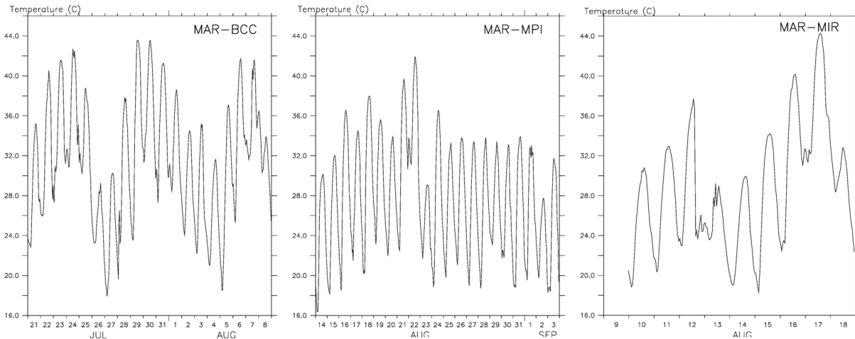
490 Figure A2: Temperature during warmest heatwave events for Liege city simulated by MAR-BCC (i.e., MAR forced by BCC-CSM2-MR), MAR-MPI (i.e., MAR forced by MPI-ESM1.2), and MAR-MIR (i.e., MAR forced by MIROC6) with the scenario SSP5-8.5 for the period 2085-2100. These data are extracted from these files:
