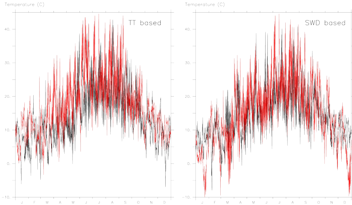
495 Figure A-1: Typical (black) and extreme (red) temperature for Liege city simulated by MAR forced by BCC-CSM2-MR with the scenario sspSSP5-8.5 for the period 2085-2100. The typical/extreme months are based on temperature (left) and incident solar radiation (right). These data are extracted from these files :
