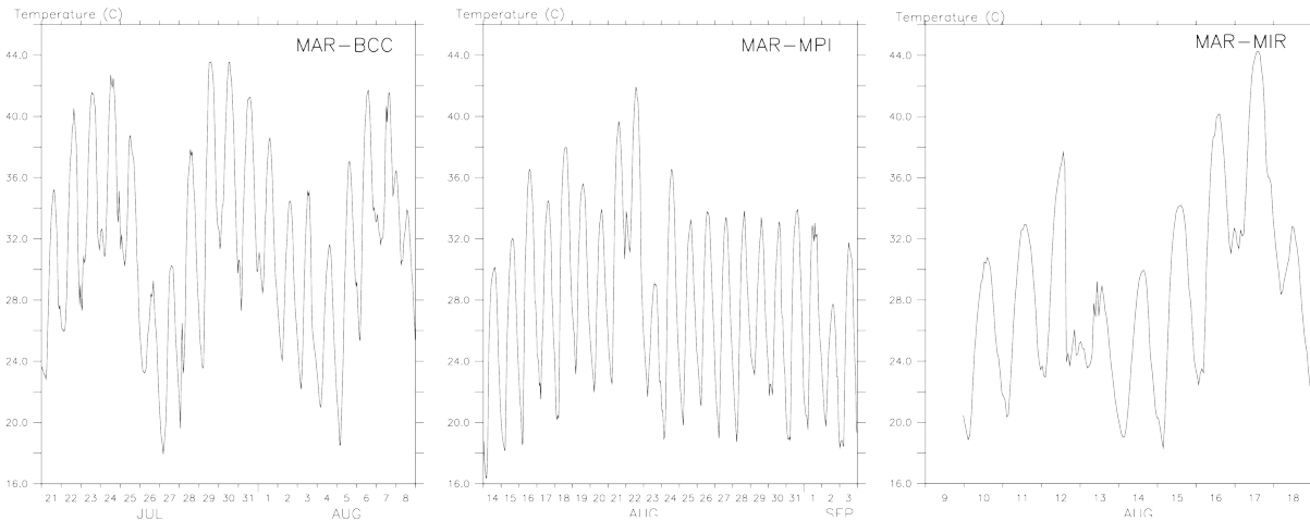
505 Figure A-2: Temperature during warmest heatwave events for Liege city simulated by MAR-BCC (i.e., MAR forced by BCC-CSM2-MR), MAR-MPI (i.e., MAR forced by MPI-ESM.1.2), and MAR-MIR (i.e., MAR forced by MIROC6) with the scenario sspSSP5-8.5 for the period 2085-2100. These data are extracted from these files :
