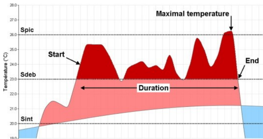
490 Figure 4 (figure and legend coming from Ouzeau et al., 2016): Characterization of a heatwave from a daily mean temperature indicator over France (example of a time series from June 30 to August 5, 1983): Duration (start and end), maximal temperature, and global intensity (red area of the plot). Temperatures above (below) climatological line (1981–2010 reference period) are represented by the pink (blue) area. (For interpretation of the references to color in this figure legend, the reader is referred to the web version of this article.)
