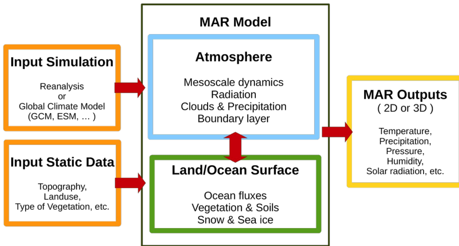
Figure 1: Workflow of the MAR model. The MAR model (black box) needs to be forced by a reanalysis model or global model (upper orange box) and by static data (lower orange box) and the result of the MAR simulation gives meteorological variables in two or three dimensions (yellow box).
