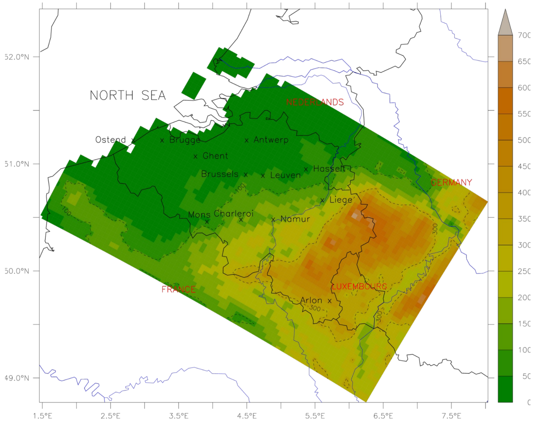
480 Figure 2: Model topography (color background, in meters), localization of cities (black) used in this dataset for Belgium, and localization of neighboring countries (in red).
