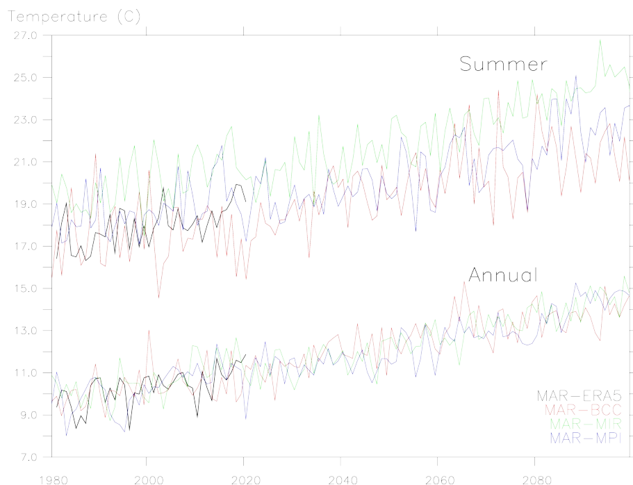
485 Figure 3: Annual mean temperature (in C, lower lines) and annual summer temperature (in C, upper lines) of MAR forced by ERA5 reanalysis (in black bold lines), MAR forced by BCC-CSM2-MR (in red lines), MAR forced by MPI-ESM1.2 (in blue lines), and MAR forced by MIROC6 (in green lines) between 1980 and 2100 according to the scenario SSP5-8.5. The average is computed here over the whole integration domain excluding the ocean.
