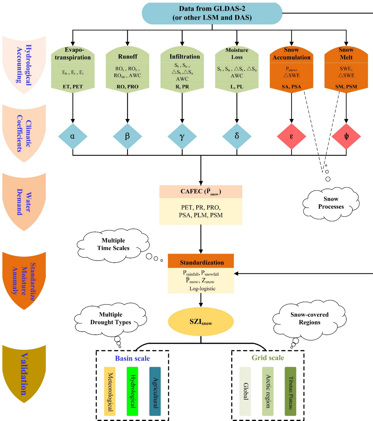
190 Figure 3. The procedure flowchart describing the production and validation of SZI_{snow} . Variables derive the SZI_{snow} from the GLDAS-2 (or other LSM and DAS). The production of SZI_{snow} includes four steps. The SZI_{snow} is validated at basin scale for three types of drought and at grid scale across different regions worldwide, respectively. The cloud-shape annotation shows the advantages of the SZI_{snow} .
