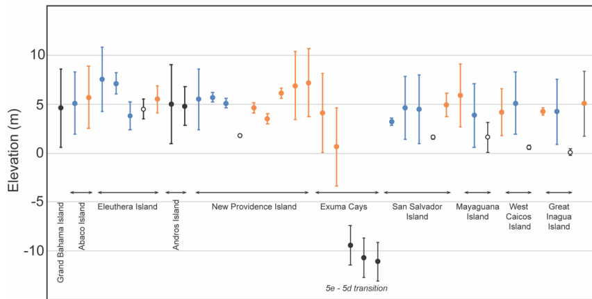
740 Figure 2. Relative sea level position during MIS 5e across the Bahamas and Turks and Caicos. Data are grouped by island and ordered roughly north to south from left to right across the diagram. Symbols are as follows (black circles = MIS 5e; blue circles = early MIS 5e; orange circles = late MIS 5e; open circles = erosional or subaerial exposure surface). Uncertainties represented by error bars include the combined uncertainty of the elevation measurement and indicative range of the sea level indicator by adding the uncertainties in quadrature.
