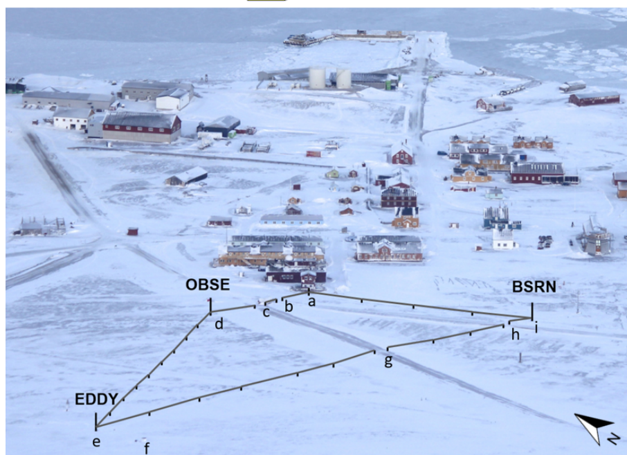
Figure 2. Schematic setup and picture of setup from the Zeppelin mountain from south. The fiber-optic array has a length of 700 m. The letters a-i refer to the same elements.
