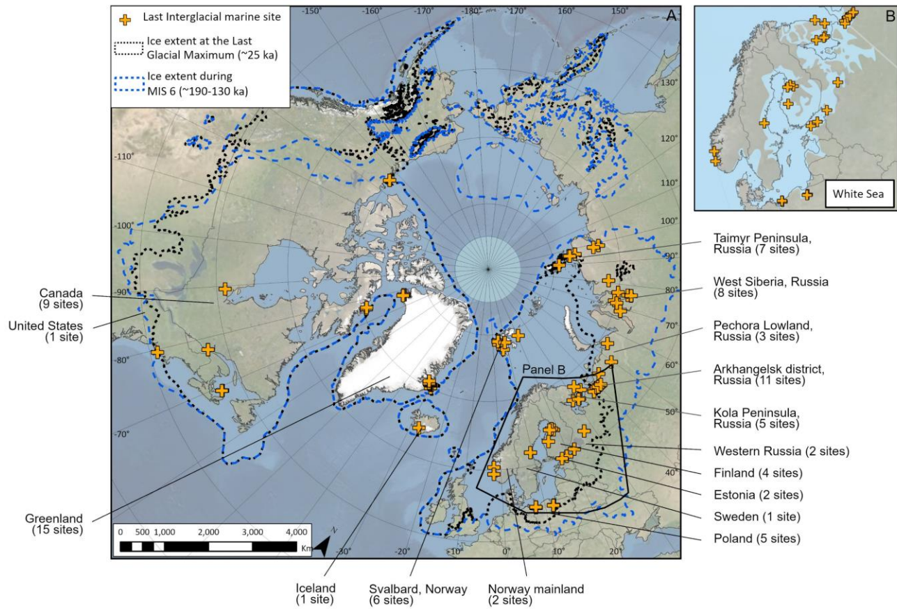
Figure. 1. Location of Last interglacial (LIG) marine sites in the formerly glaciated Northern Hemisphere, along with the extent of MIS 6 and Last Glacial Maximum ice sheets (Batchelor et al., 2019). Inset map shows extent of the LIG White Sea that inundated the isostatically depressed landscape of western Russia and northwestern Europe.
