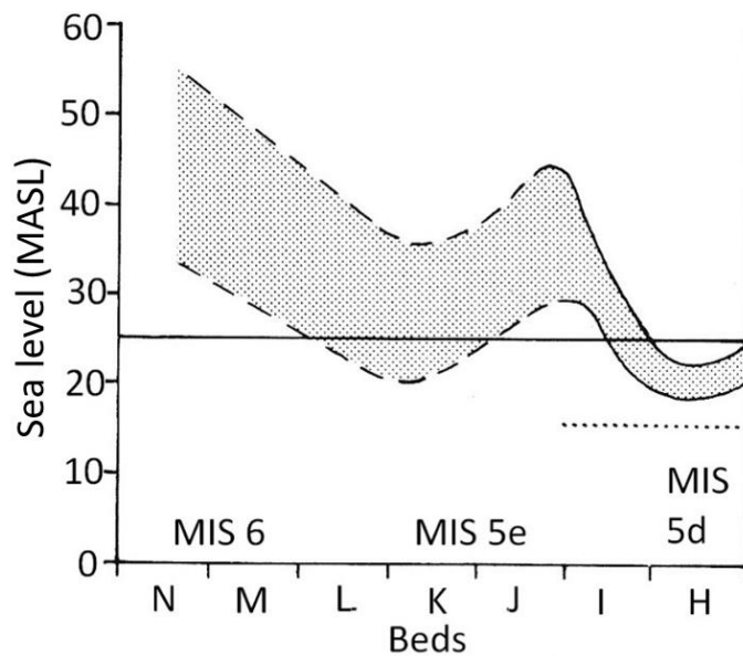
1895 Figure 7. Relative sea-level curve for Fjøsanger during the LIG, shown as a dotted uncertainty band. The dashed part of the curve is considered most uncertain. The line at 25 MASL shows the threshold in the Bergen Valley; when sea level was higher than this threshold the fjord turned into a sound that was open in both ends. The dotted line at 15 MASL shows the top of the LIG marine sediments and thus the minimum altitude of the RSL during the entire LIG. Modified from Mangerud et al., (1981).
