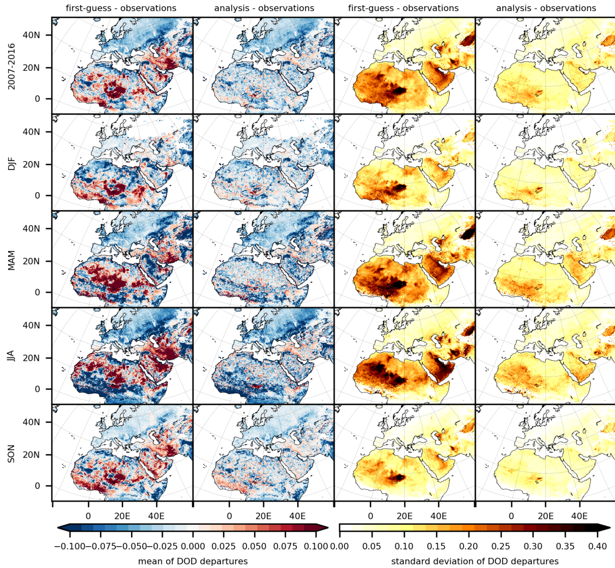
Figure 8. Maps of mean 3-hourly DOD_{coarse} for first-guess departures (first column), analysis departures (second column), standard deviation of first-guess departures (third column) and standard deviation of analysis departures (fourth column) calculated for the whole period (2007-2016; top row) and for different seasons (DJF, MAM, JJA, SON; rows 2 to 5). Model fields are ensemble mean and are collocated with the observations.
