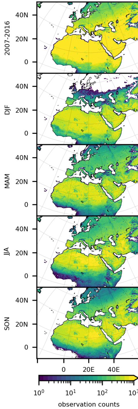
Figure 2. Maps of counts of assimilated observations for the whole period (2007-2016; top row) and for the different seasons (DJF, MAM, JJA, SON; rows 2 to 5) of the 10-year period.
