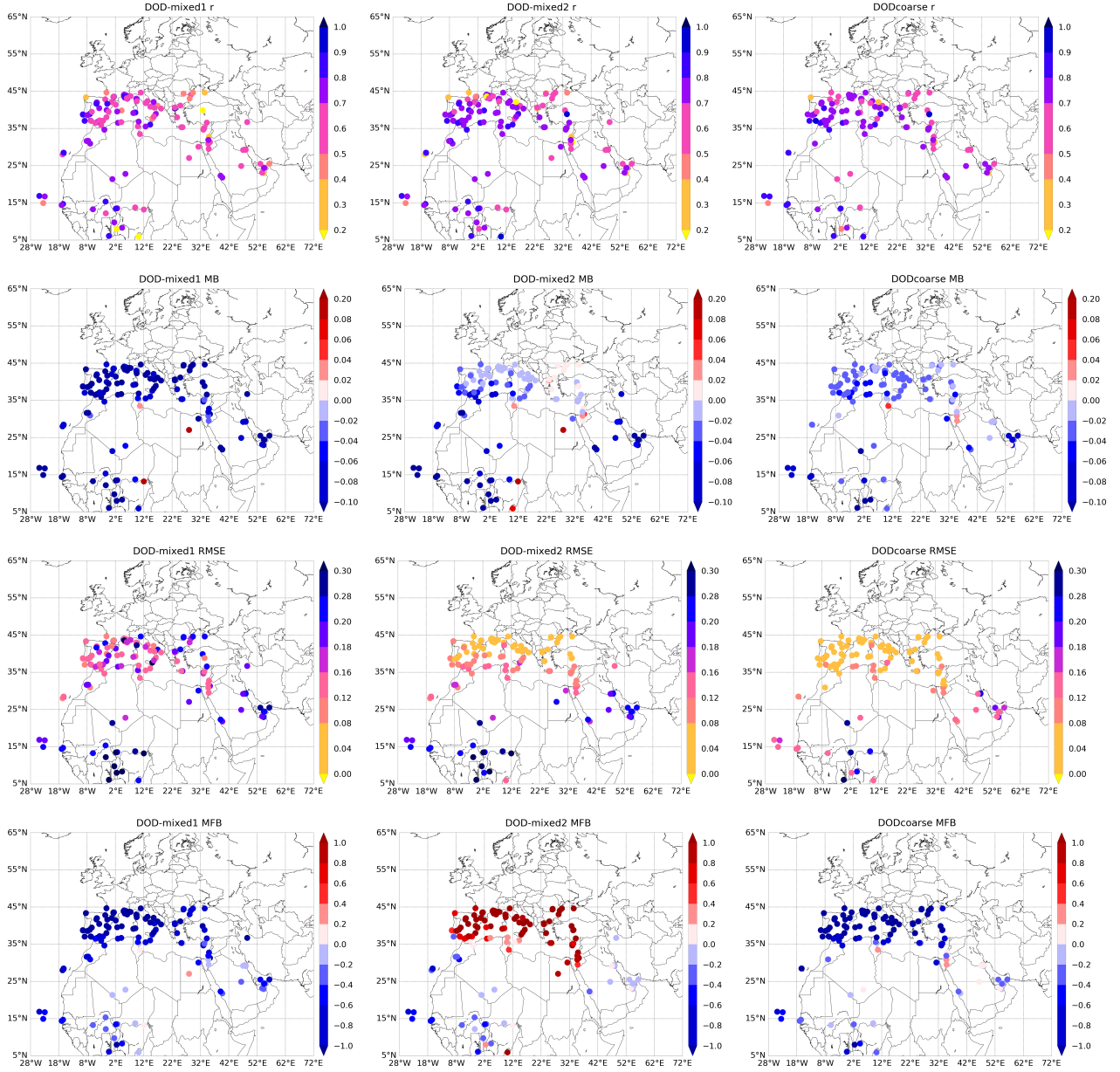
Figure 12. Maps of verification statistics (r, MB, RMSE, MFB, from top to bottom) of the analysis DOD (first and second columns) and DOD coarse (third column) versus AERONET dust-filtered AOD (Table 6): DOD-mixed1 (left), DOD-mixed2 (middle) and DOD coarse (right) calculated for the whole period (2007-2016). The results are obtained using 3-hourly collocated reanalysis and observation values (see also Table 7).
