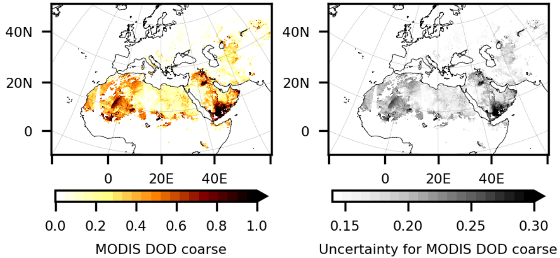
Figure 1. Example of assimilated observations for July 9, 2012: DOD_{coarse} retrieved from the Aqua MODIS DB Level 2 products (Collection 6; left) and the associated observation uncertainty used in the assimilation algorithm (right).
