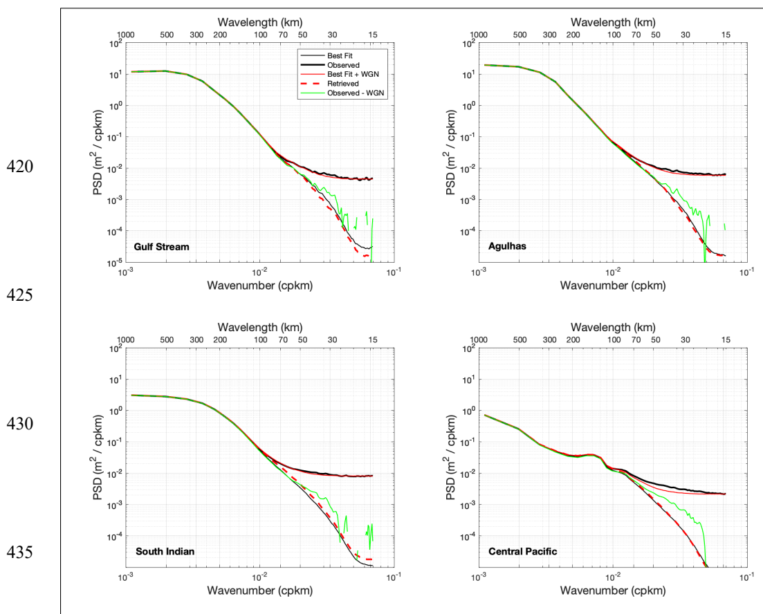
Figure 5: Mean Power Spectral Density (PSD) of Saral SLA along-track measurements: Observed (thick black), Best Fit (thin black), Best Fit plus White Gaussian Noise (red), Retrieved (dashed red), Observed minus WGN (green). WGN is estimated as the average in the range 15-25 km of the mean observed PSD (bold black curve). The PSD is the average of PSDs computed over all data segments covering the years 2016-2018, and the Gulf Stream region (72° W-60° W; 44° N-32° N).
