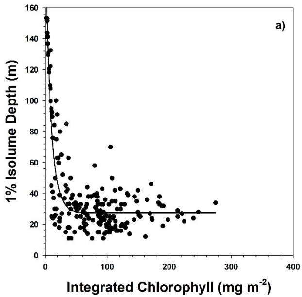
Figure 6: Relationship between integrated chlorophyll concentrations (integrated through the 1% isolume depth) and the 1% isolume depth at a) stations dominated by Phaeocystis antarctica and b) stations dominated by diatoms. The relationships were best described by an exponential decay equation and were highly significant ( R^2 = 0.77 and R^2 = 0.17 ; p < 0.0001 for both). Both axes were made equal to allow a direct comparison.
