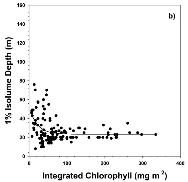
Figure 6: Relationship between integrated chlorophyll concentrations (integrated through the 1% isolume depth) and the 1% isolume depth at a) stations dominated by Phaeocystis antarctica and b) stations dominated by diatoms. The relationships were best described by an exponential decay equation and were highly significant ( R^2 = 0.77 and R^2 = 0.17 ; p < 0.0001 for both). Both axes were made equal to allow a direct comparison.
