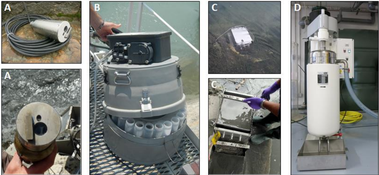
185 Fig. 4 - Devices used for SSC measurement and SPM sampling. A) Hach Lange Solitax SC turbidity probes equipped with a wiper, B) Automatic sampler (ISCO, Teledyne ISCO, Lincoln, USA) used for the calibration of turbidity stations, C) Particle Trap, and D) Continuous Flow Centrifuge at Jons station.
