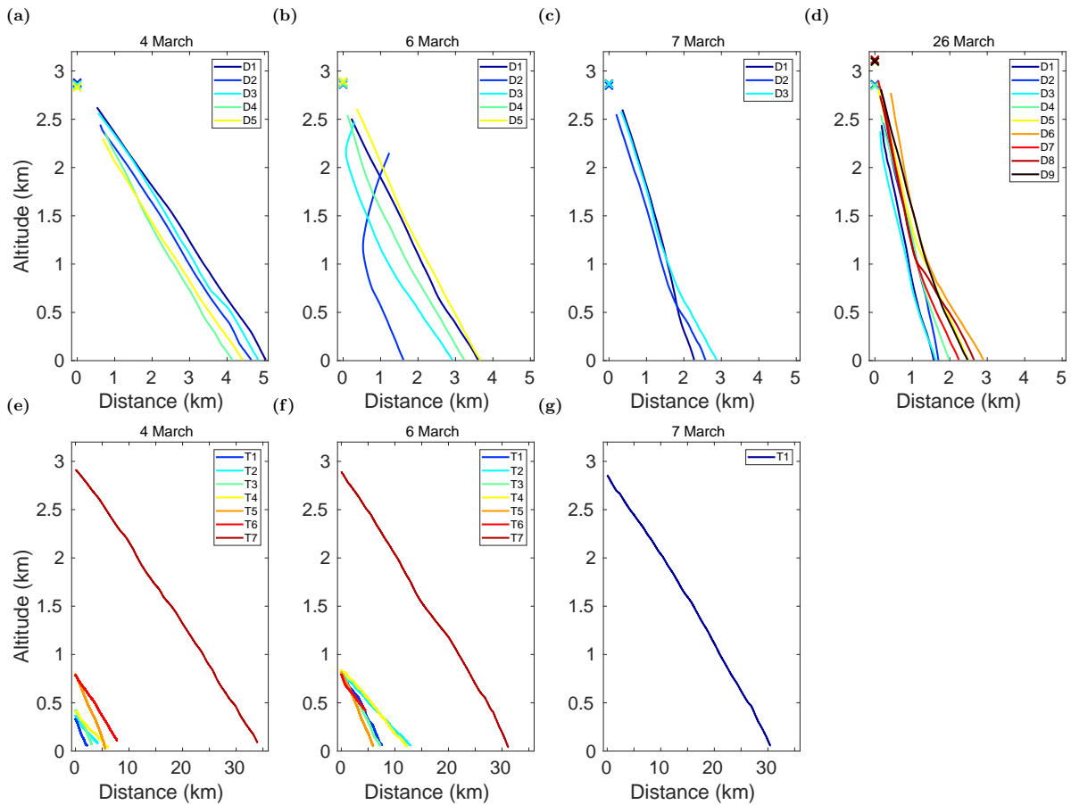
Figure 5. Horizontal drift distances of the drosondes (a)–(d) and distances flown by the aircraft during ascents and descents (e)–(g). Distances are calculated with respect to the uppermost measurement point. For the drosondes, this information is missing for the uppermost layer (see text), and coloured crosses refer to the drosondes’ release altitudes derived via GPS.
