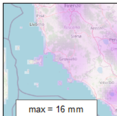
max of 6-hourly maps
