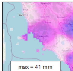
sum of 6-hourly maps
