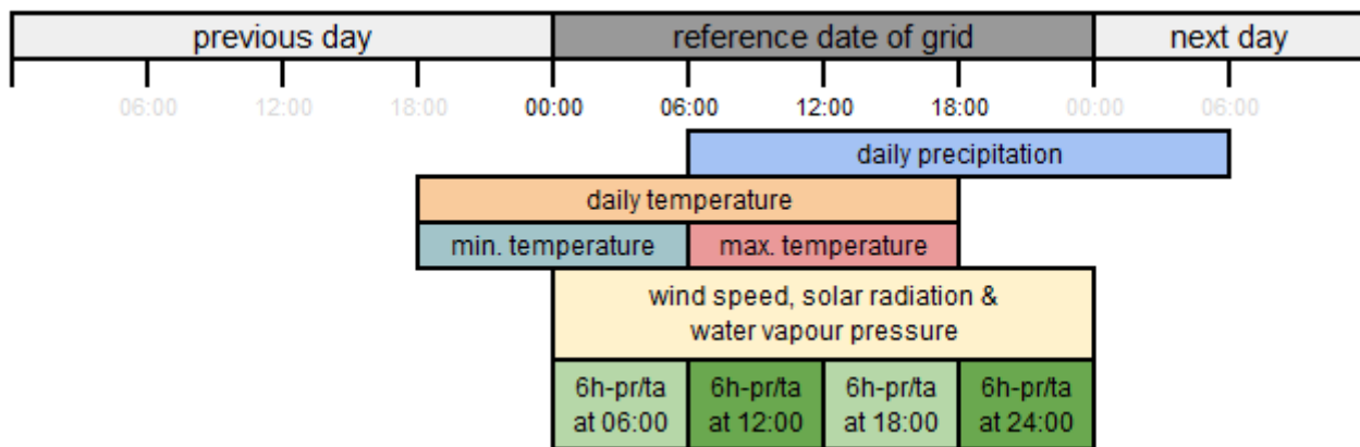
735 Figure 5: Aggregation i.e. reference period of the EMO-5 grids per variable.
