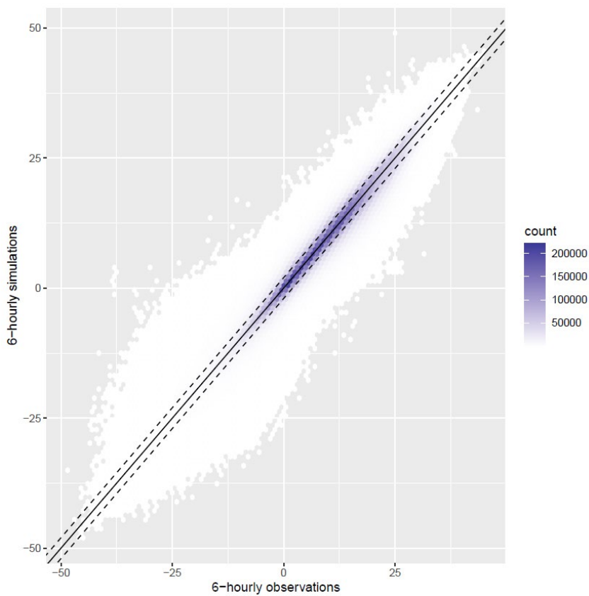
Figure 7: Comparison of observed and simulated 6-hourly temperatures.
