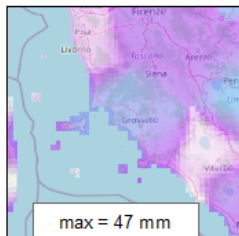
max of daily maps
