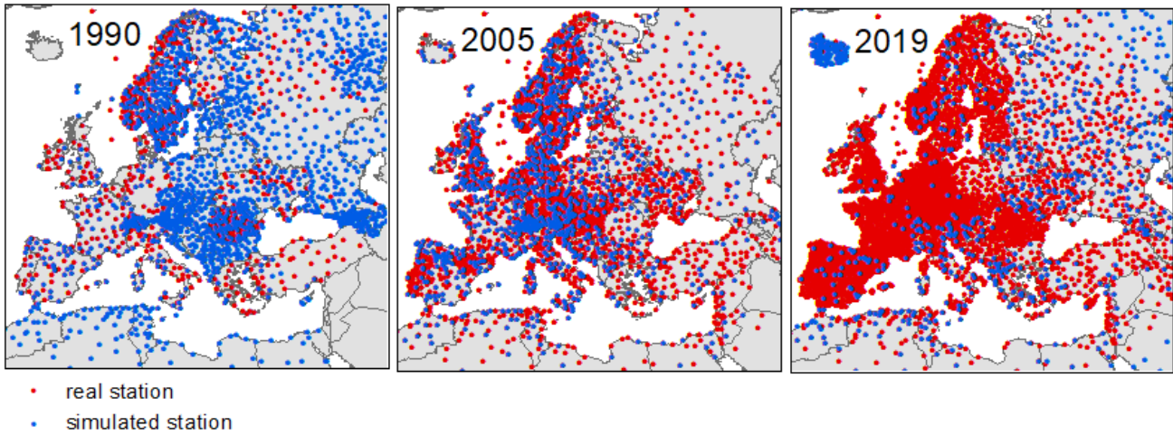
715 Figure 6: Coverage of existing and simulated stations used for the 6-hourly temperature fields for 1990, 2005 and 2019.
