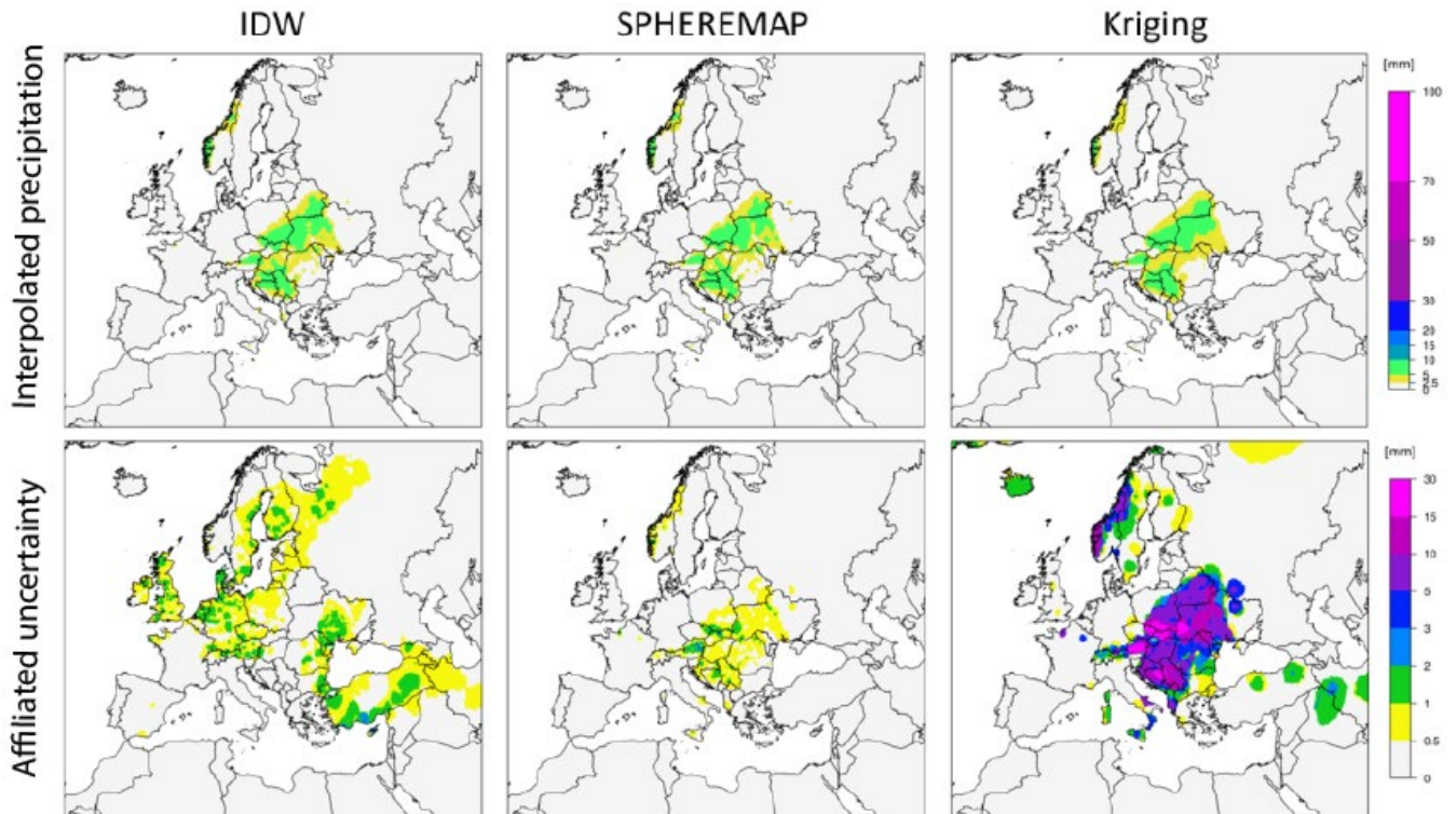
710 Figure 4: Gridded daily precipitation data (top row) and the corresponding uncertainty fields (bottom row) for the 15.05.2014 as an example for IDW (left), SPHEREMAP (middle) and Kriging (right).
