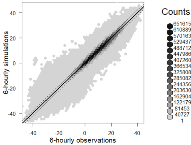
Figure 7: Comparison of observed and simulated 6-hourly temperatures.
