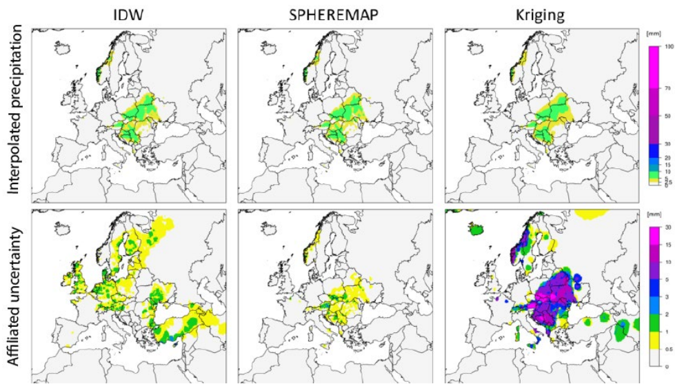
745 Figure 4: Gridded daily precipitation data (top row) and the corresponding uncertainty fields (bottom row) for the 15.05.2014 as an example for IDW (left), SPHEREMAP (middle) and Kriging (right).
