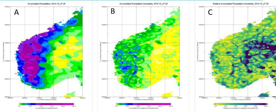
Figure 8: Example of interpolated precipitation totals and associated uncertainty for extreme event No. 3 in Section 5.3. (A) Accumulates precipitation totals from 2014/10/27 to 2014/10/29 (three days), (B) accumulated uncertainty of the interpolated precipitation totals and (C) the percentage of the accumulated uncertainty in relation to the accumulated precipitation totals.
