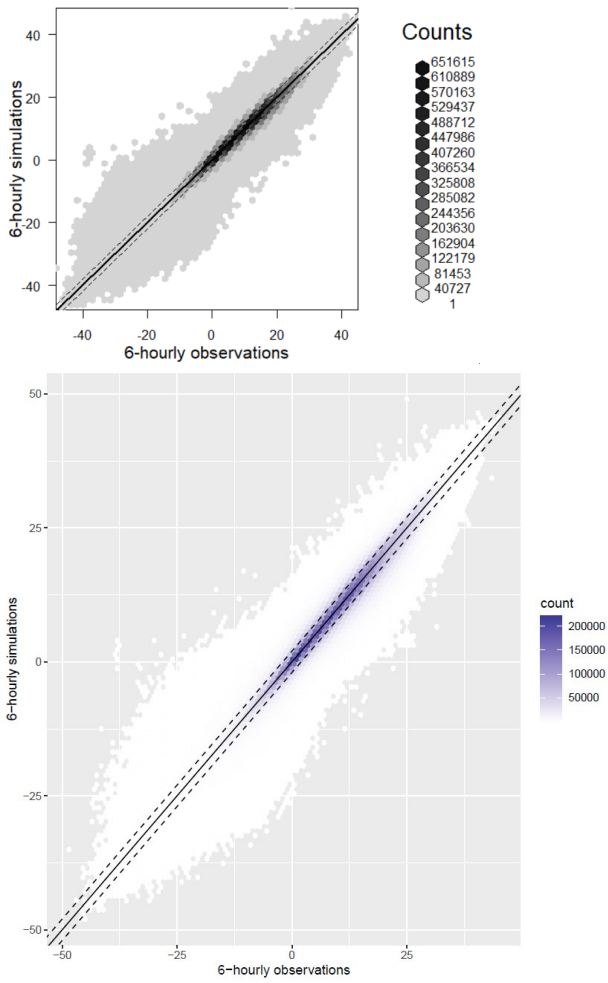
Figure 7: Comparison of observed and simulated 6-hourly temperatures.
