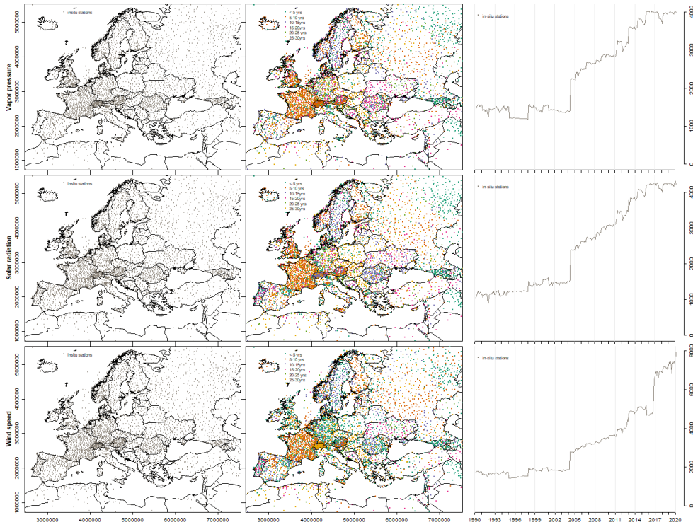
740 Figure 2: Input data for daily EMO-5 vapour pressure, solar radiation and wind speed grids in terms of station locations, record lengths and number of stations used.
