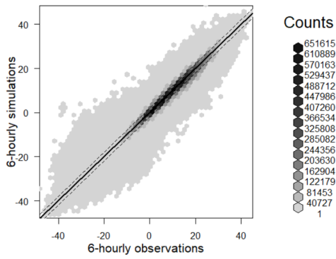
Figure 7: Comparison of observed and simulated 6-hourly temperatures.
