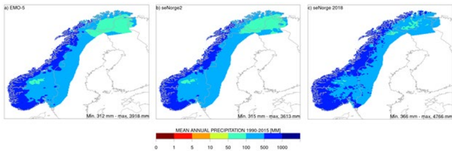
Figure 89: Mean annual precipitation [mm] for the (a) EMO-5, (b) seNorge2, and (c) seNorge 2018 data sets for the joint period 1990-2015. seNorge data are bi-linearly interpolated to the coarser EMO-5 resolution. EMO-5 was cropped to the same spatial extent as the seNorge data sets.
