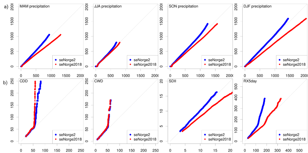
Figure 4011: Quantile plot of a) seasonal precipitation, where each point represents the sum of a grid value over 3 months and b) extreme value indices (ETCCDI) values, but these correspond to the maximum of the entire time series. Each plot shows seNorge2
