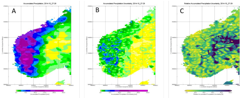
Figure 78: Example of interpolated precipitation totals and associated uncertainty for extreme event No. 3 in Section 5.3. (A) Accumulates precipitation totals from 2014/10/27 to 2014/10/29 (three days), (B) accumulated uncertainty of the interpolated precipitation totals and (C) the percentage of the accumulated uncertainty in relation to the accumulated precipitation totals.
