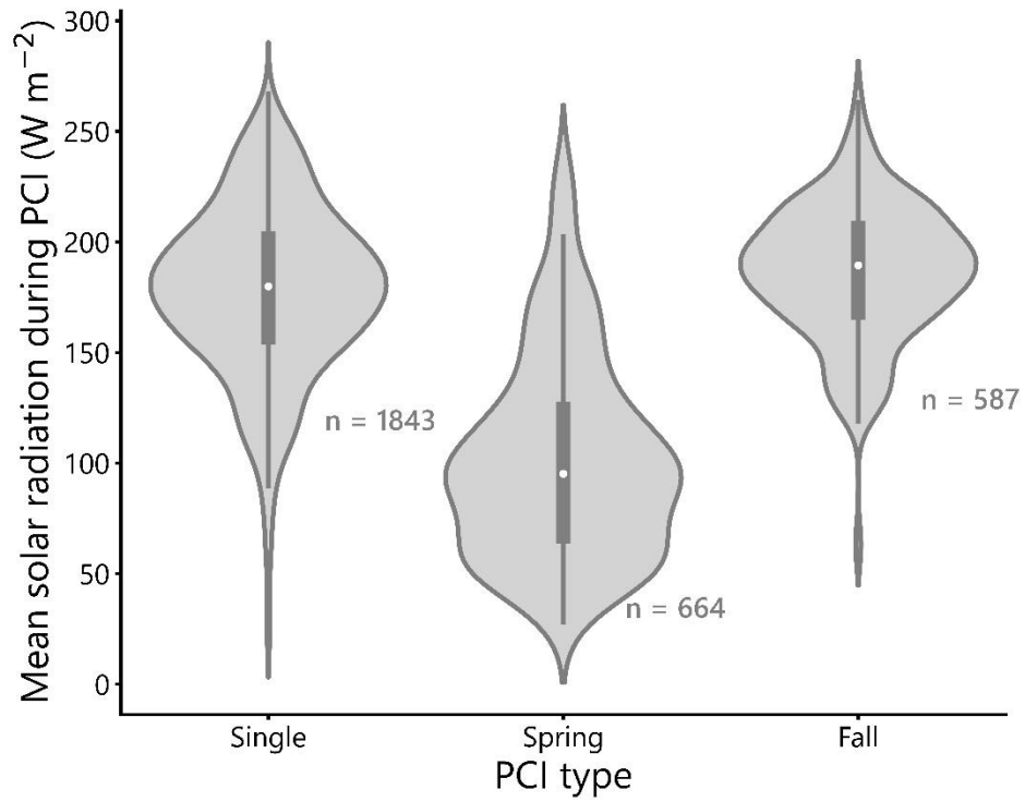
665 Figure 9: Mean PCI surface solar radiation (SSR) grouped by PCI type (single, spring, or fall). White circles show the mean value for each violin. The mean SSR during spring PCIs is lower than that of single and fall PCIs, which have similar distributions.
