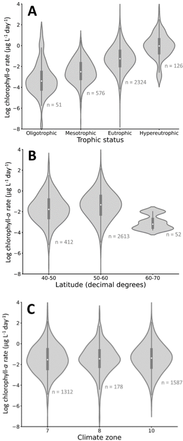
650 Figure 7. Rate of Chlorophyll-a increase (RCI) trends in the dataset, grouped by (a) trophic status, (b) latitude, and (c) climate zone. Lakes of a higher trophic status have a higher mean RCI while lakes at higher latitudes have lower RCI (with considerable overlap between all categories). Grouping by climate zone shows minimal effect on RCI. The number of lakes represented by each violin is shown in grey text on the panels. Climate zones are as follows: 7 = cold and mesic; 8 = cool, temperate, and dry; 10 = warm, temperate, and mesic. White circles indicate the mean value for each violin.
