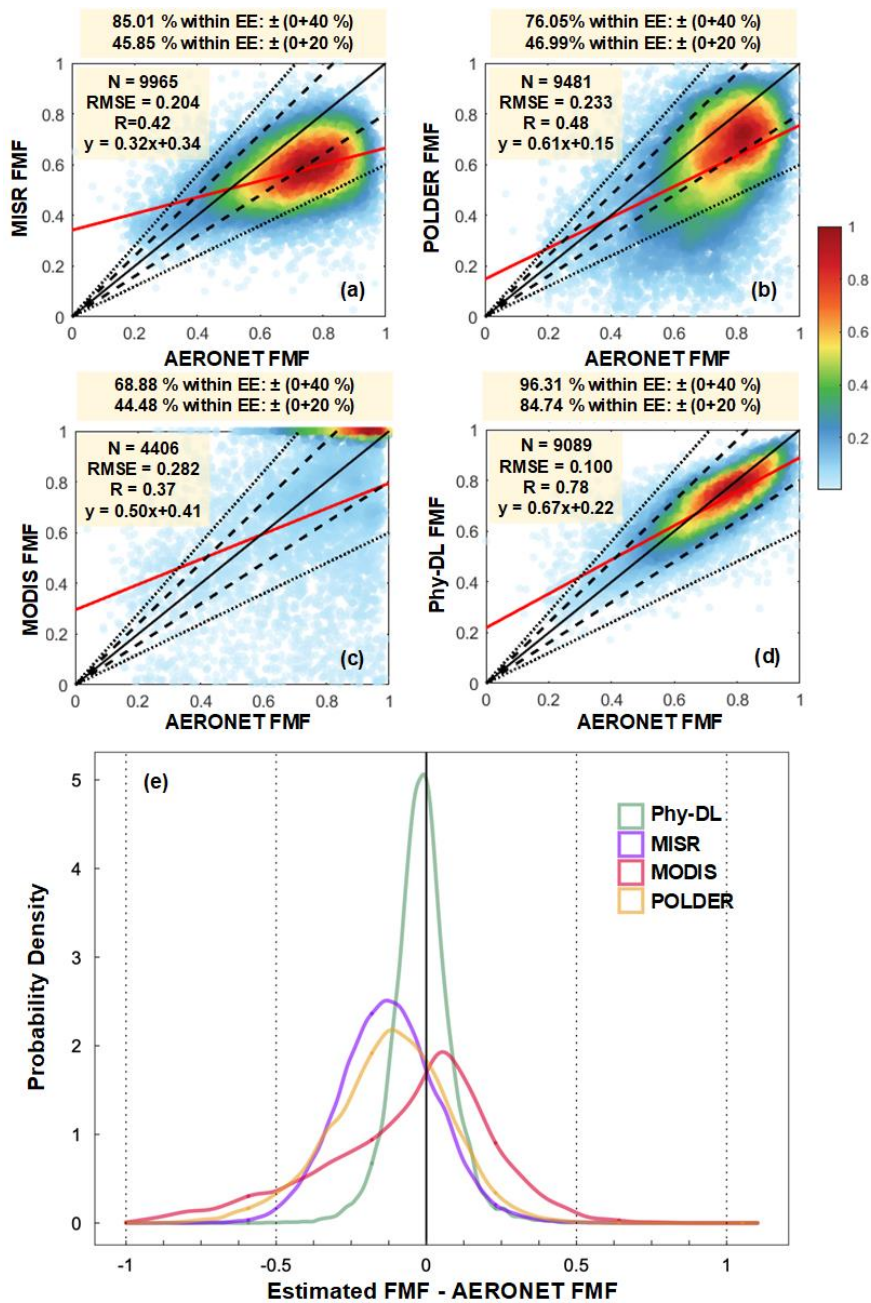
Figure 10: Evaluation of (a) MISR (550 nm), (b) POLDER (490 nm), (c) MODIS (550 nm), and (d) Phy-DL FMFs (500 nm) against AERONET FMF (500 nm) from 2008 to 2013. Black and red solid lines are 1:1 reference lines and best-fit lines from linear regression, respectively. Black dashed and dotted lines represent the EE envelopes of \pm 20\% and \pm 40\% , respectively. The number of samples (N), RMSE, correlation coefficient (R), and linear regression relation are given in each panel. (e) Probability density functions of the FMF bias (estimated FMF minus AERONET FMF) for MISR (blue), POLDER (orange), MODIS (red), and Phy-DL (green) FMFs.
