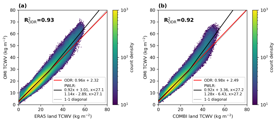
Figure B6. Same as Fig. B4, but for data over land. The red solid line represents the ODR results and the solid black line the PWLR results.
