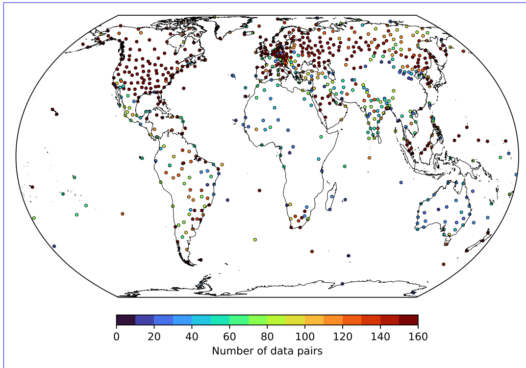
Figure 13. Same as Fig. 7, but now with ESA WV CCI CDR-2 data Global distribution of radiosonde stations used for the TCWV intercomparison to the MPIC OMI data over ocean (top row) and for set. Colours indicate the amount of data over land (bottom row) pairs for the intercomparison.
