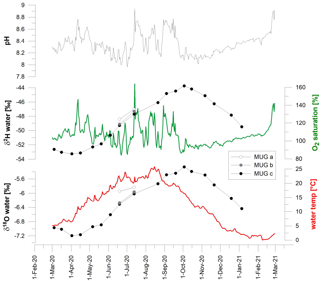
375 Figure 4: Timeseries of \delta^2\text{H} and \delta^{18}\text{O} values from the samples taken in 2-4 weekly intervals (March 2020 – January 2021) at the outflow of Müggelsee (MUG c: Friedrichshagen harbour) and from additional samples taken on the northern shore (MUG a and b) on 19 th June and 13 th July. Water chemical data from the IGB measuring station (IGB, 2022).
