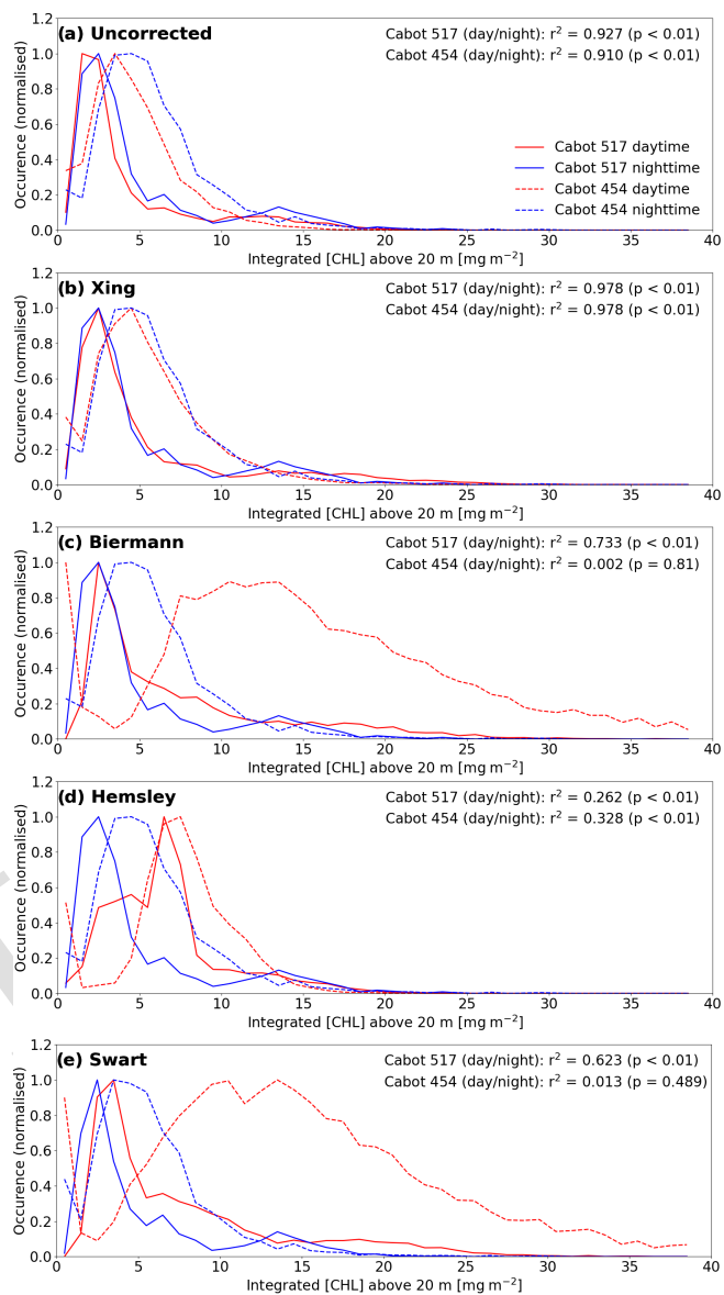
Figure 5. The effects of the implementation of different quenching mechanisms on the distribution of the integrated [Chl- a ] in the top 20 m for Cabot deployments 454 (dashed lines) and 517 (solid lines). Panel (a) shows the distribution of daytime (red) and nighttime (blue) [Chl- a ] in the uncorrected case. Panels (b), (c), (d), and (e) show the effects of implementing the mixed-layer-depth-based correction of Xing et al. (2012), euphotic-depth-based correction of Biermann et al. (2015), and the backscatter-based corrections of Hemsley et al. (2015) and Swart et al. (2015).
