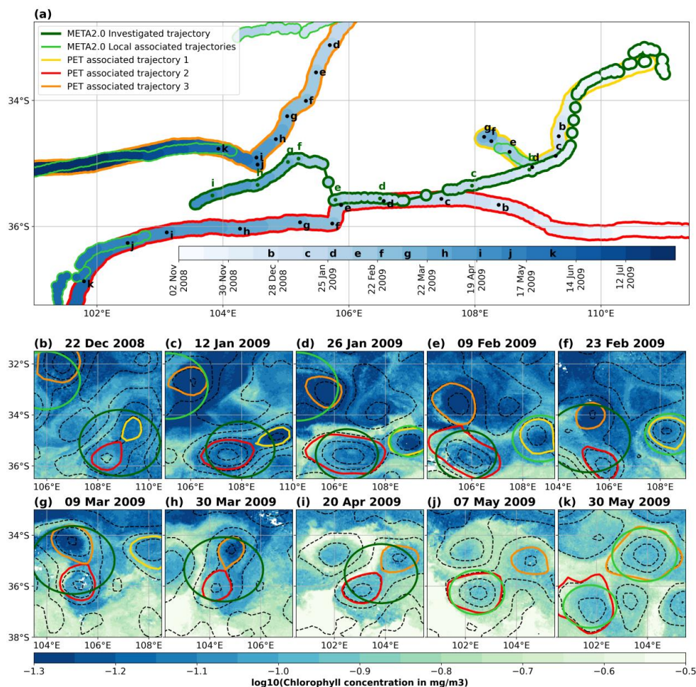
630 Figure 9 : Selected eddies detected by both OSU (META2.0) and PET algorithms. The input field (filtered SLA) is identical for both detections, as the tracking (restricted area method). Eddies were selected as representative examples highlighting the differences between the two detection algorithms. Panel (a) shows six META2.0 trajectories (the dark green investigated trajectory, and five smaller ones in light green) and three PET trajectories 635 (yellow, red and orange) for eddies detected over the same temporal period, from November 2008 to January 2009 (color scale). Dashed black lines in panels (b-k) show arbitrary 10 cm levels of filtered SLA. Background colors in panels (b-k) show chlorophyll-a concentrations in logarithmic scale (data courtesy of CLS). Note the reverse color scale, showing high concentrations in light color. Letters on panel (a) correspond to the snapshot time of panels (b-k) as well as panel (a) trajectories outline colors correspond to contours in panels (b-k).
