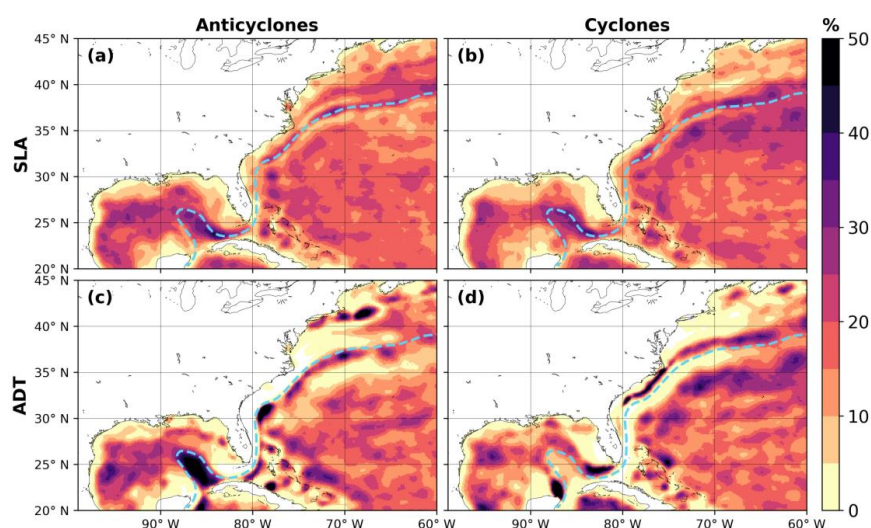
Figure 6: Percentage of time spend by each pixel of 0.1^\circ \times 0.1^\circ within anticyclones detected in (a) SLA and (c) ADT maps and within cyclones detected in (b) SLA and (d) ADT maps. The dashed blue line follows the velocity maximum of the current.
