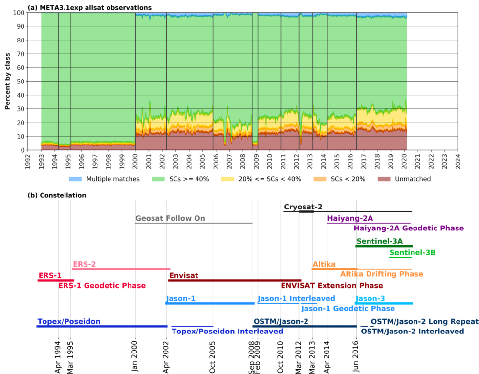
360 Figure 4 : (a) Temporal evolution of the similarity coefficient distribution obtained for the META3.1exp all-satellites, compared with the META3.1exp two-satellites. The percentage of unmatched observations (dark red shading) represents eddies detected in the all-satellite product but absent in the two-satellite atlas. The low and intermediate similarity coefficients (SCs < 40%, yellow and orange shadings) highlight eddies with shifted locations. Eddies similarly detected in the all-satellites and two-satellites products represent most of the eddies (SCs \geq 40%, green shading). (b) Temporal evolution of the satellite constellation used for the two-satellites (thick lines, reference missions) and the all-satellite (thin lines) products. The highlighted changes in the missions correspond to some abrupt variations in the SCs.
