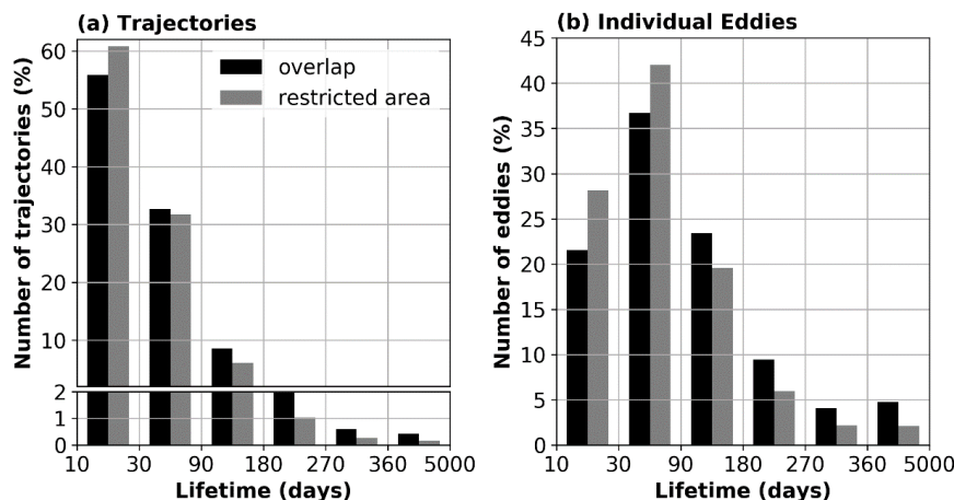
275 Figure 2 : Distribution of the number of (a) trajectories and (b) individual eddies by lifetime for the restricted area (grey) and the overlap (black) tracking methods built from the same detection dataset. Percentages are relative to the number of trajectories lasting at least 10 days and the individual eddies for each tracking : 1.67 million trajectories built with the restricted area tracking from 62 million individual eddies and 1.46 million trajectories built with the overlap tracking from 65 million individual eddies. Note the discontinuity in the yaxis of (a).
