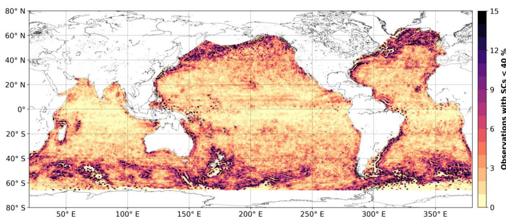
425 Figure 5 : Number of eddy centers associated with ADT-detected eddies that are unmatched or matched with low similarities indexes (SCs < 40 %) with SLA-detected eddies.
