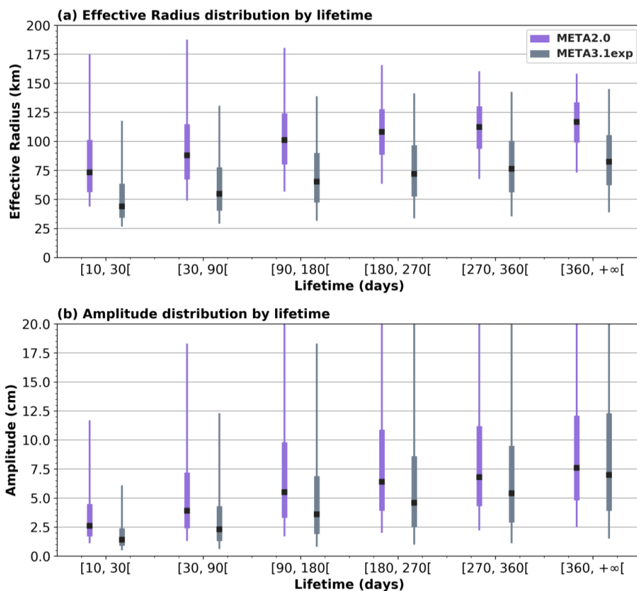
685 Figure 10: Distribution of (a) Effective Radius and (b) Amplitude for different lifetimes for the META2.0 eddies (purple) and META3.1exp eddies (grey). The black squares mark the median, the thick lines span from the 25 th to the 75 th percentiles, and the thin lines from the 5 th to the 95 th percentiles of the data.
