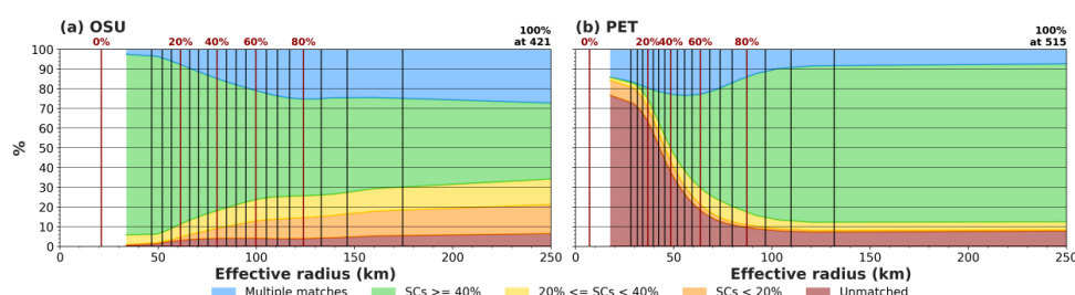
545 Figure 8 : Similarity coefficient repartition as a function of the effective radius for the eddies detected with (a) OSU and (b) PET over the 1000 km filtered SLA. The vertical lines separate the eddies in 20 equally distributed classes of ~1.7 million eddies for OSU and ~2.8 million eddies for PET.
