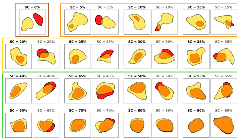
325 Figure 3 : Illustration of the Similarity Coefficients (SCs) from 0 % to 100 %. A SC of 0 % is when the eddies of one atlas have no match in the other atlas (brown rectangle), SCs strictly below 20 % are associated with quite different eddies (orange rectangle), SCs between 20 – 40 % are considered as intermediate (yellow rectangle), and SCs over 40 % are associated with very similar eddies (green rectangle). Except for unmatched eddies (SC = 0 %), for each SC is presented on the left the case of one eddy included in the other, and on the right the case of shifted eddies.
