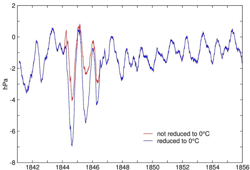
Figure 6: 91-day running means of daily mean-sea-level pressure differences between Trieste and Milan (hPa). Trieste pressure reduced to 0 °C is shown in blue, and the 10 March 1844–23 May 1846 as appears in the Repertori is shown in red.
