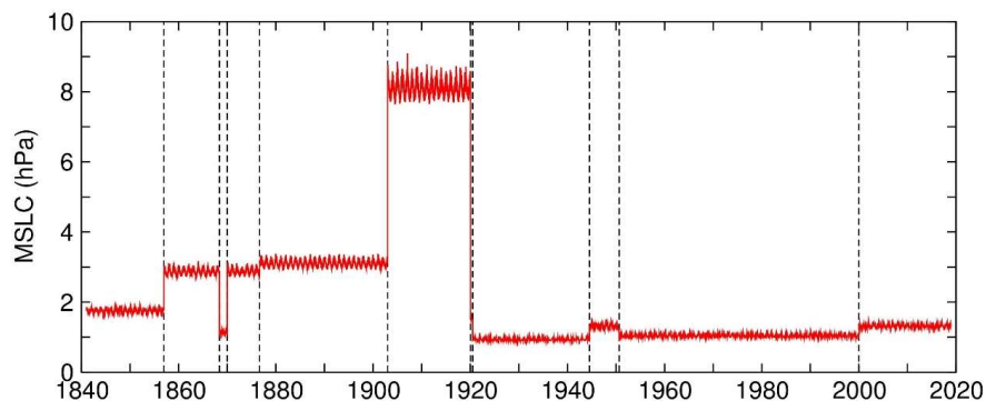
5 Figure A1: Daily corrections to reduce pressure to MSL ( MSLC ) in hPa. The dashed vertical lines correspond to the barometer height changes summarized in Table 3.
