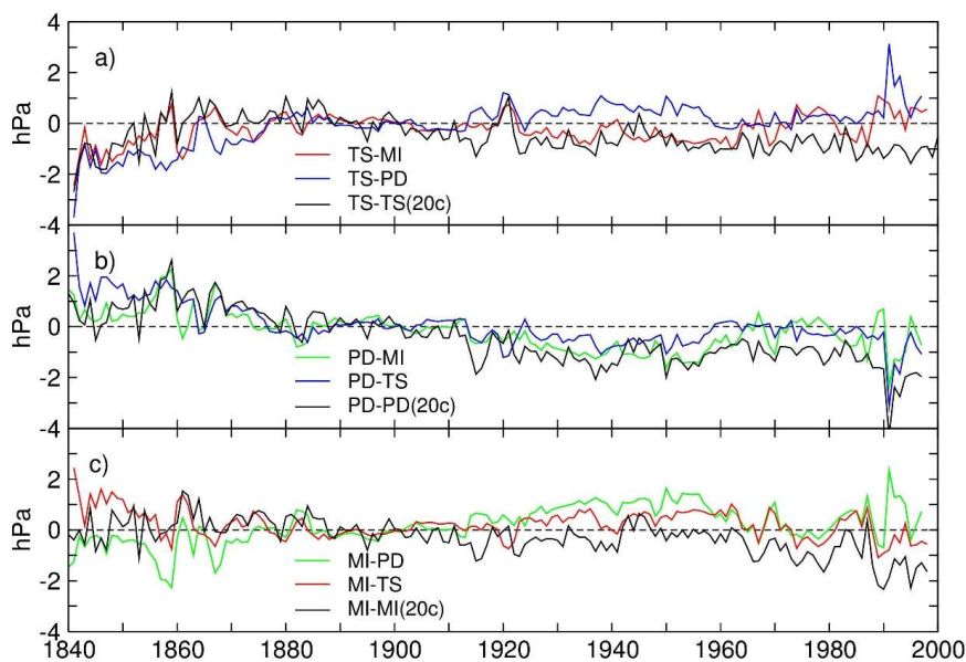
Figure 7: Comparisons of annual mean pressures (hPa): a) differences involving Trieste; b) differences involving Padua; c) differences involving Milan. Black curves represent the comparisons between each station and the corresponding time series from the 20 th Century Reanalysis; the comparison between Trieste and Milan is shown in red, that between Trieste and Padua in blue and that between Padua and Milan in green.
