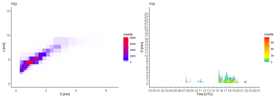
Figure 4. Example of disdrometer data for 22 June 2011 at site 3 (disdrometer P22). (left) Scatterplot of the number of drops according to the velocity (terminal fall speed) and size (equi-volumetric drop diameter) classes. (right) Temporal evolution of the DSD.
