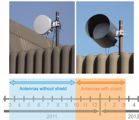
Figure 2. (top) Outdoor unit of the Dual-Pol MiniLink-MINI-LINK and the antenna radome without (left) and with custom shield (right). (bottom) Timeline of the operational period of the shielding of antenna radomes.
