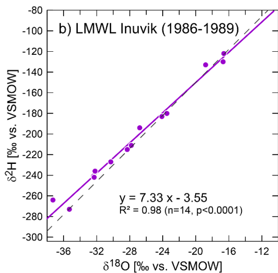
Figure 3. Co-isotope plots of \delta^{18}\text{O} and \delta^2\text{H} of precipitation for Inuvik (NT, Canada). (a) New (n=34, 2015-2018) local meteoric water line. (b) Old (n=14, 1986-1989) local meteoric water line. Dashed line represents the global meteoric water line.
