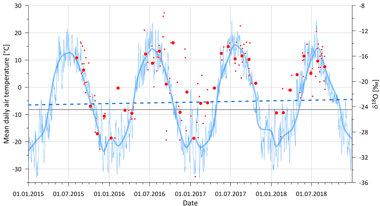
135 Figure 2. Air temperatures from Inuvik (NT, Canada) together with \delta^{18}\text{O} values in precipitation during the sampling period from August 2015 to August 2018. Thin blue line shows mean daily air temperatures and the thick blue line shows monthly averages. Small red dots show all \delta^{18}\text{O} data points. Large red dots show \delta^{18}\text{O} monthly averages. Grey line illustrates long-term average of air temperatures (1981-2010). Blue dashed line illustrates air temperature trend from 2015 to 2018.
