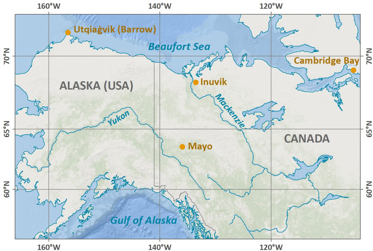
Figure 1. Map with WMO stations in the western Arctic, where GNIP data and LMWLs exist (i.e., Inuvik, Utqiagvik [Barrow], Mayo and Cambridge Bay). Map by Sebastian Labor (Alfred Wegener Institute, AWI, Potsdam, Germany).
