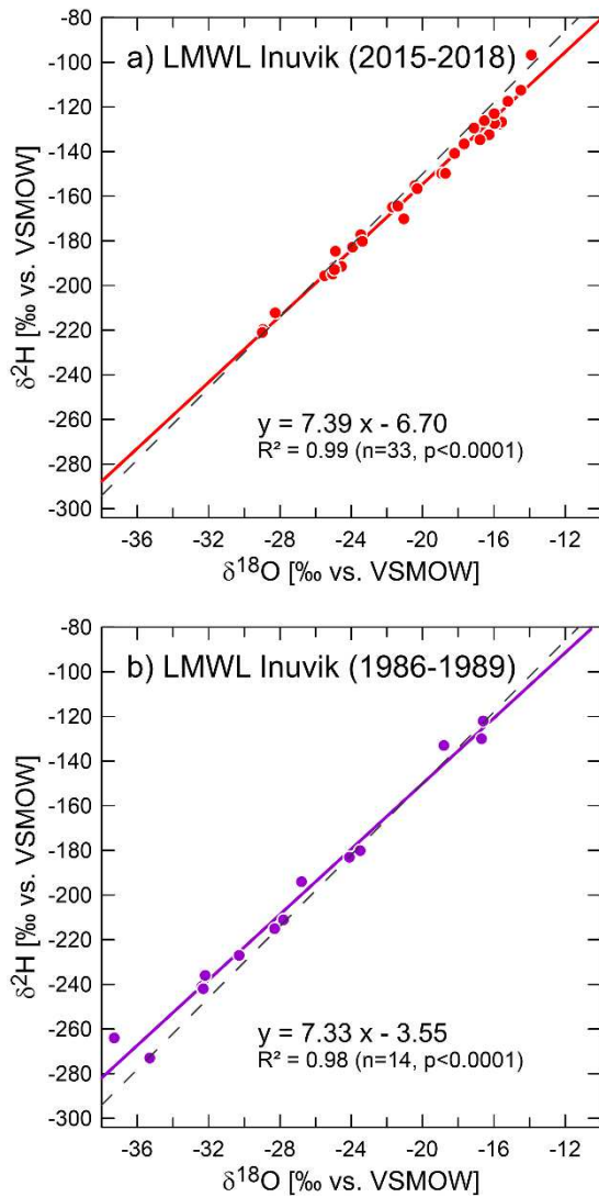
165 Figure 3. Co-isotope plots of \delta^{18}\text{O} and \delta^2\text{H} of precipitation for Inuvik (NT, Canada). (a) New ( n=34 , 2015-2018) local meteoric water line. (b) Old ( n=14 , 1986-1989) local meteoric water line. Dashed line represents the global meteoric water line.
