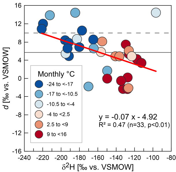
Figure 4. Relationship between hydrogen isotope ratios ( \delta^2\text{H} ) and Deuterium excess d (monthly means). The solid horizontal line indicates mean d from Inuvik (this study), whereas the dashed line indicates global average d . Bubble colour indicates air temperature ranges (monthly mean) at the time of sampling. Red line represents the linear trend.
