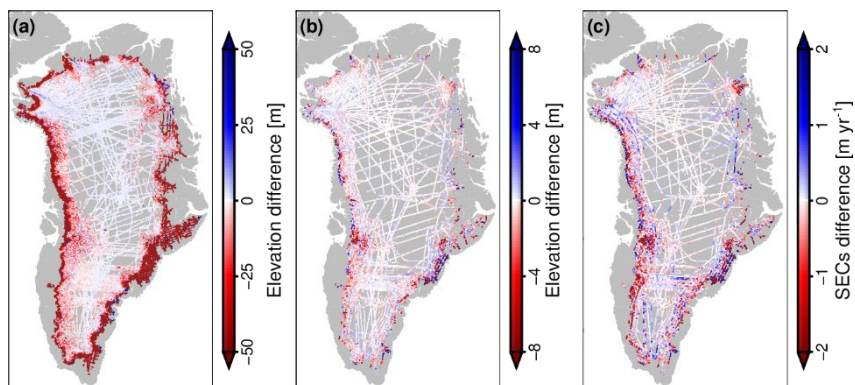
Figure 9: Validation with ATM laser altimeter observations: (a) differences between SE derived from ATM L2 and our merged time series, (b) SE differences, and (c) SEC differences between ATM L4 observations and our merged time series at the same epochs.
