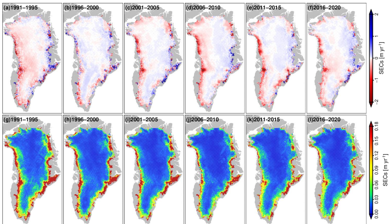
545 Figure 5: Maps of long-term SECs and their uncertainties from the combined elevation time series over the periods of (a) and (g), 1991–1995, (b) and (h) 1996–2000, (c) and (i) 2001–2005, (d) and (j) 2006–2010, (e) and (k) 2011–2015, and (f) and (l) 2016–2020.
