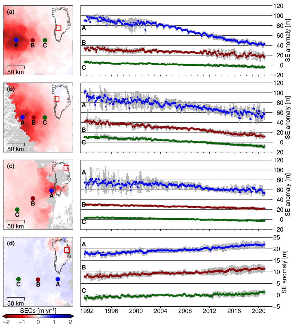
550 Figure 6: SE anomaly time series near (a) Jakobshavn Isbræ, (b) Upernavik Isstrøm, (c) Zachariae Isstrøm and Nioghalvfjærdsfjorden glacier, and (d) King Christian X Land. The locations of the selected points (A, B, and C) are marked in the left-hand maps of elevation change over 1991–2020. The time series and the 1\sigma uncertainty ranges for each point are given in the right-hand plots with the time series of points A and B shifted along the SE anomaly axis for better visibility.
