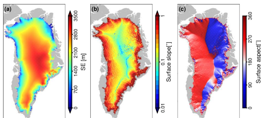
525 Figure 1: (a) SE of the GrIS DEM at reference time 2010.0, and (b) surface slope and (c) aspect derived from the DEM.
