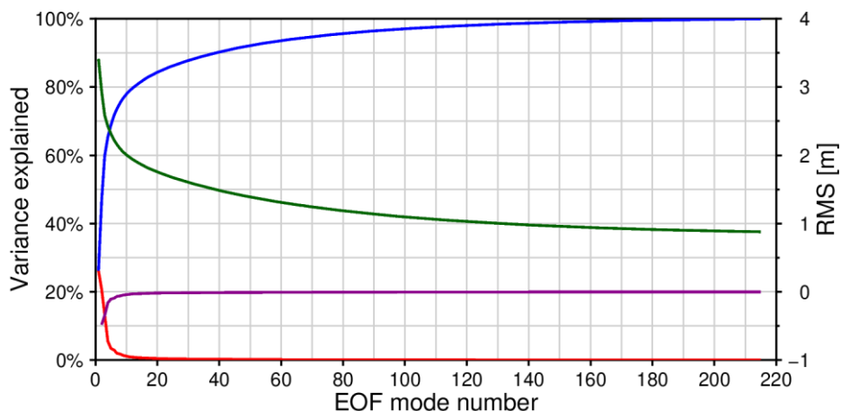
530 Figure 2: Percentage of variance explained (red line) and cumulative variance explained (blue line) by each EOF mode; RMS error (green line) and its derivative (purple line) of the difference between the reconstructed time series of monthly elevation change and that of observation in different EOFs.
