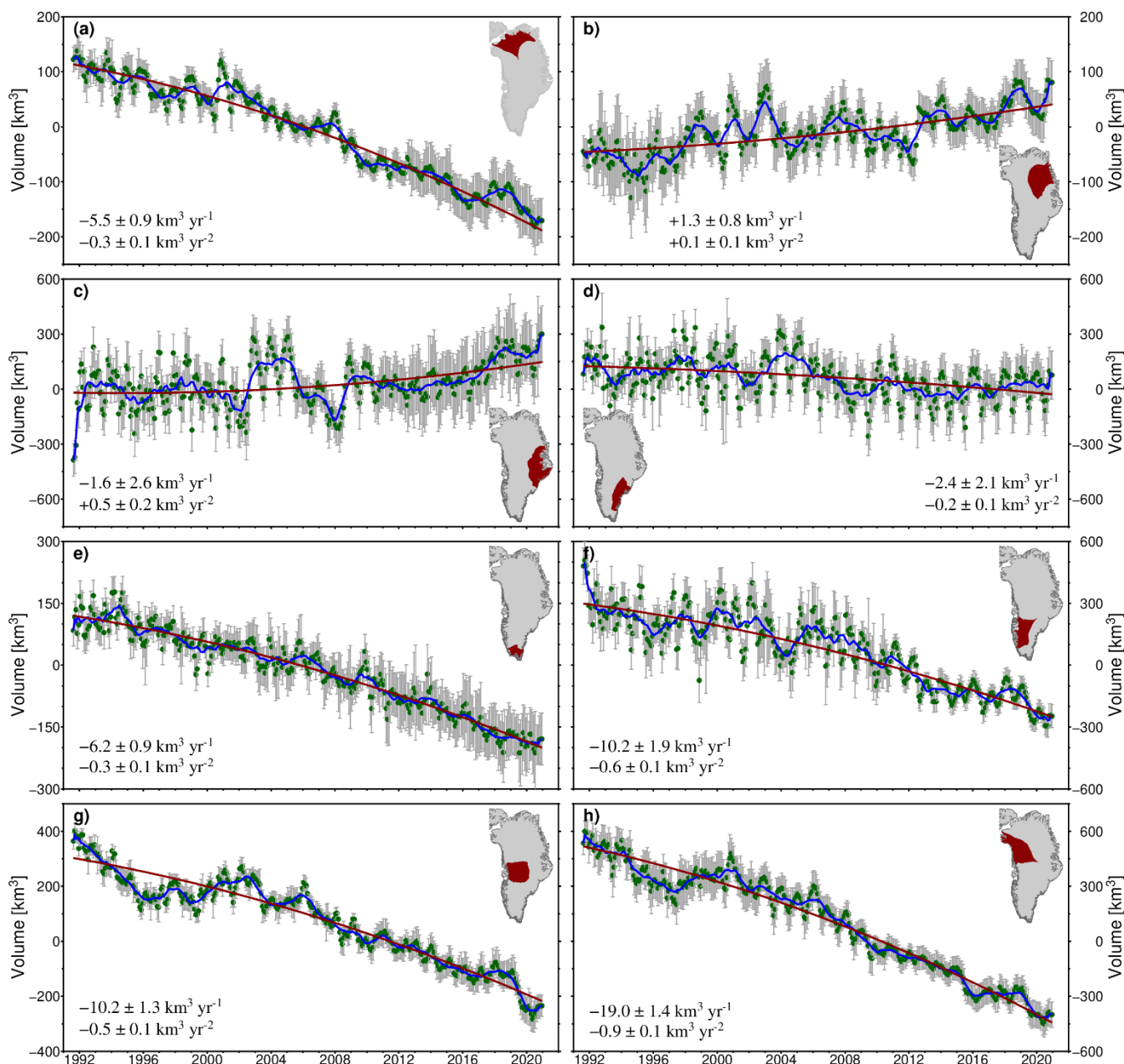
565 Figure 8: Volume change of sub-regions south of 81.5^\circ\text{N} from our merged altimetric time series (green dots) and their corresponding results after removing seasonal oscillations using a 13 month moving average (blue solid curves). The solid red lines are the best-fit quadratic curves for the linear and quadratic trend estimates of volume change. The grey error bars show the 1\sigma uncertainty range of the altimetry data. The red shaded area in the inset of each panel indicates the coverage of the sub-region with reference to the Greenland drainage system boundaries in Zwally et al. (2012).
