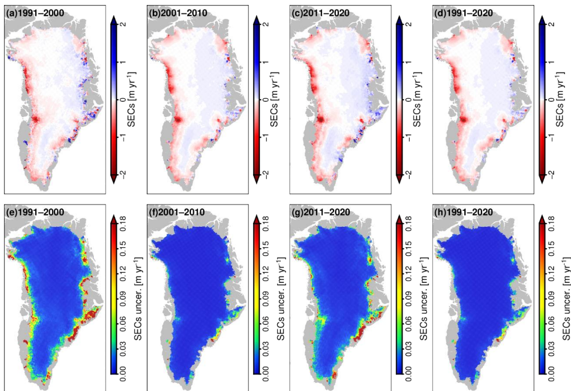
540 Figure 4: Maps of long-term SECs and their uncertainties from the combined elevation time series over the periods of (a) and (e) 1991–2000, (b) and (f) 2001–2010, (c) and (g) 2011–2020, and (d) and (h) 1991–2020.
