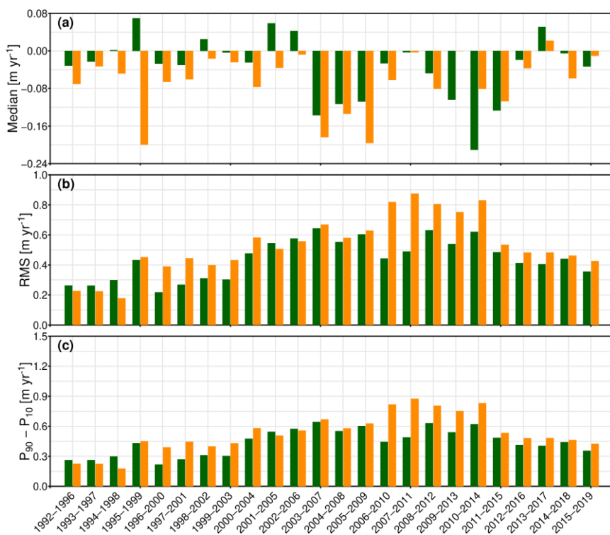
Figure 10: Validation with GrIS CCI SECs: (a) median, (b) RMS error, and (c) P_{90}-P_{10} of the SEC differences between CCI (orange) and those derived from our merged time series (green) at 5 year intervals during 1992–2019.
