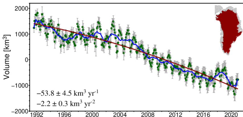
Figure 7: Volume change of the entire GrIS south of 81.5°N from our merged altimetric time series (green dots) and its corresponding result after removing seasonal oscillations using a 13 month moving average (blue solid curve). The solid red line is the best-fit quadratic curve for the linear and quadratic trend estimates of volume change. The grey error bars show the 1 \sigma uncertainty range of the altimetry data. The red shaded area in the inset indicates the coverage of the GrIS with reference to the Greenland drainage system boundaries in Zwally et al. (2012).
