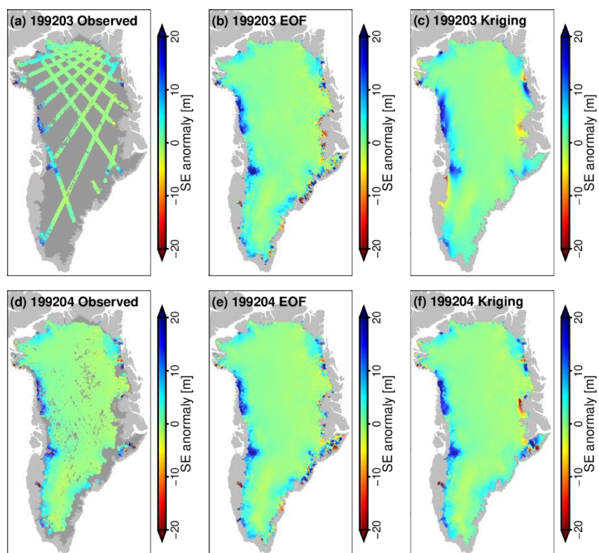
535 Figure 3: Interpolation performance of EOF reconstruction and ordinary kriging: (a), (b), and (c) are the results for March 1992 observation, EOF reconstruction, and ordinary kriging interpolation, respectively, and (d), (e), and (f) are the same for April 1992.
