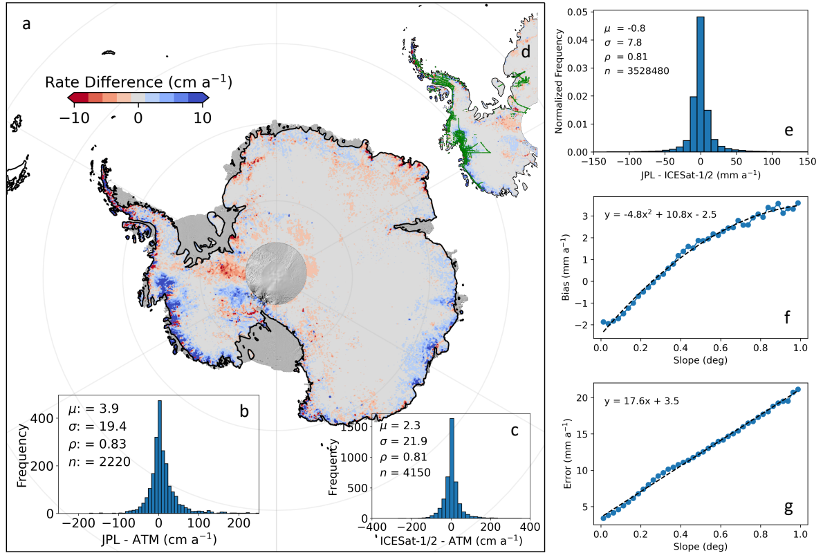
Figure 7. Elevation change validation and comparison using rates derived from ICESat - ICESat-2 and airborne ATM data over the time period of 2003-2019 and 2001-2019, respectively. (a) shows the spatial distribution of the elevation change differences from this study (JPL) differenced with rates derived from Smith et al. (2020). (b) shows the comparison of rates derived from JPL with ATM at locations indicated in (d) with green flight lines. (c) shows the comparison between ICESat - ICESat-2 derived rates with ATM. (e) depicts the ice sheet wide histogram of elevation change differences. (b,c,e) include the distribution mean ( \mu ), standard deviation ( \sigma ), correlation ( \rho ), and number of observations ( n ). (f-g) the bias (mean) and error (standard deviation) as a function of surface slope for the JPL – ICESAT-1/2 validation.
