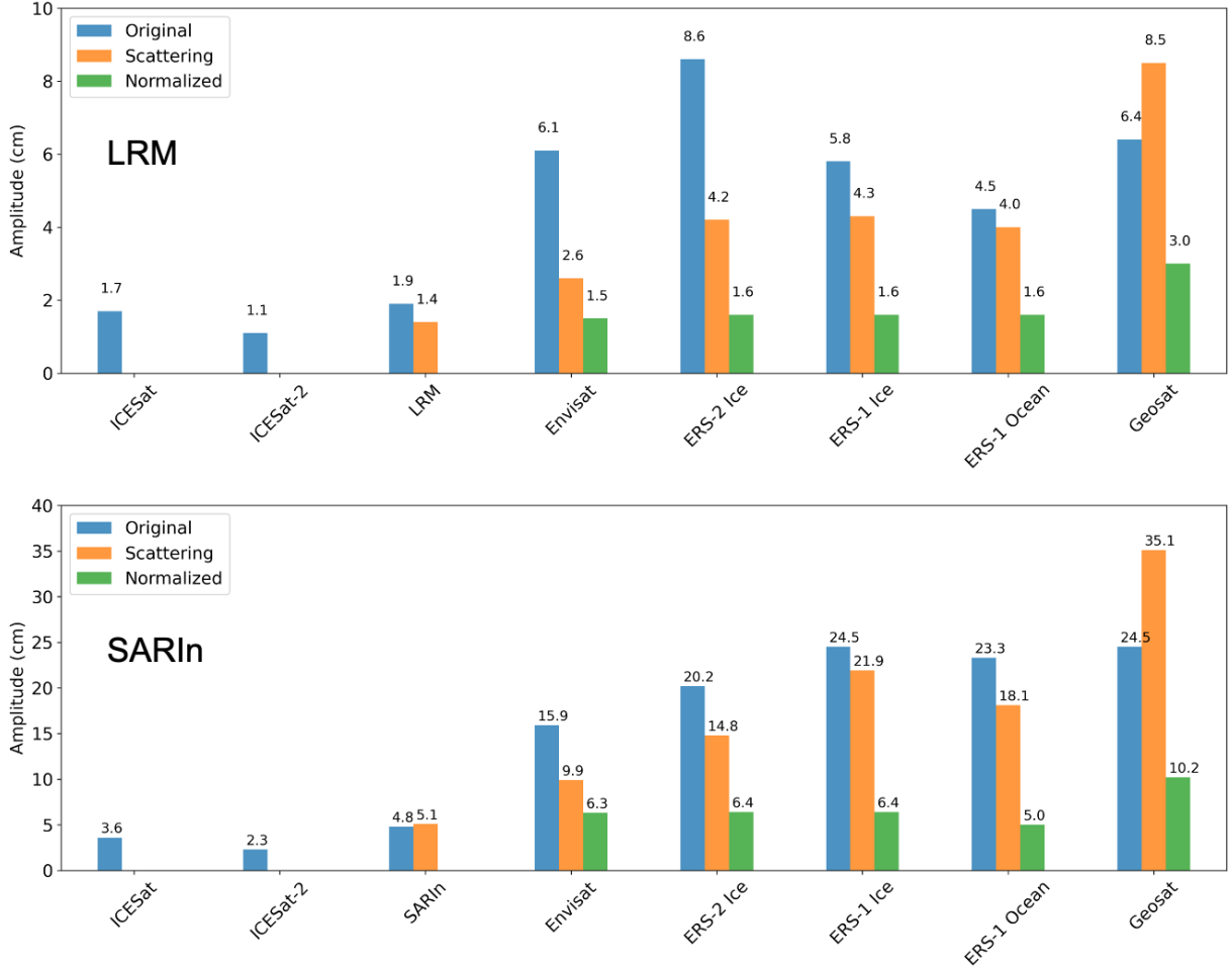
Figure 5. Top: Median seasonal amplitude of the different missions and modes for the CryoSat-2 LRM (top) and SARin (bottom) mode masks (South of 81.5° S for LRM). The blue bars show the original seasonal amplitude with no corrections applied, the orange bars show the amplitude once the mission dependent scattering correction has been applied, and the green bars show the normalized amplitude after adjustment using CryoSat-2 as reference.
