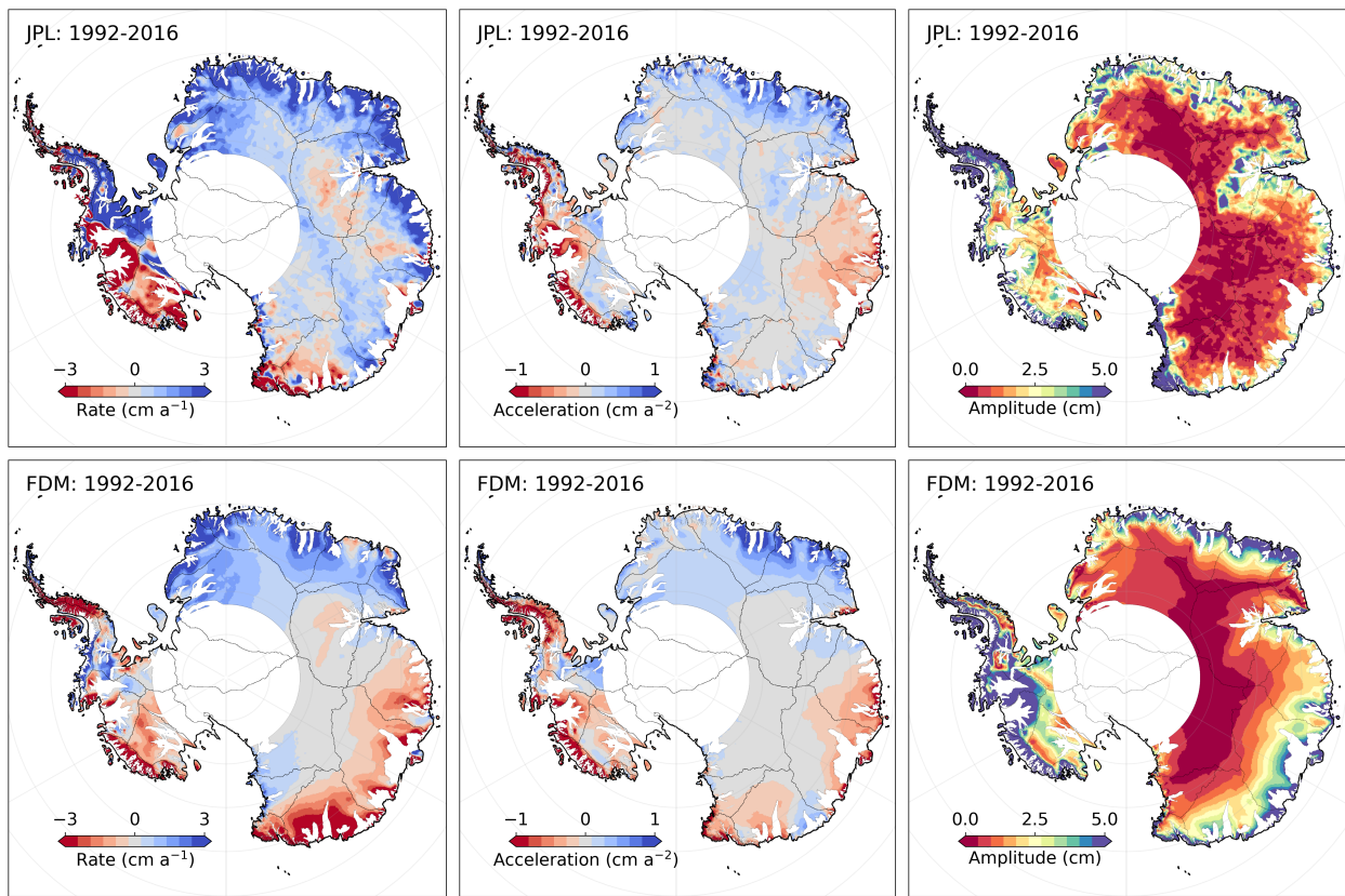
Figure 9: Spatial fields of rates (left column), acceleration (middle column) and seasonal amplitudes (right column) from our product (JPL: top row) and modelled values from the IMAU firm densification model (FDM: bottom row). Areas of fast flow ( >30 \text{ m a}^{-1} ) have been masked out to minimize height changes caused by changes in ice flow. The altimetry data has been smoothed with a 50 km median filter to highlight large scale spatial patterns.
