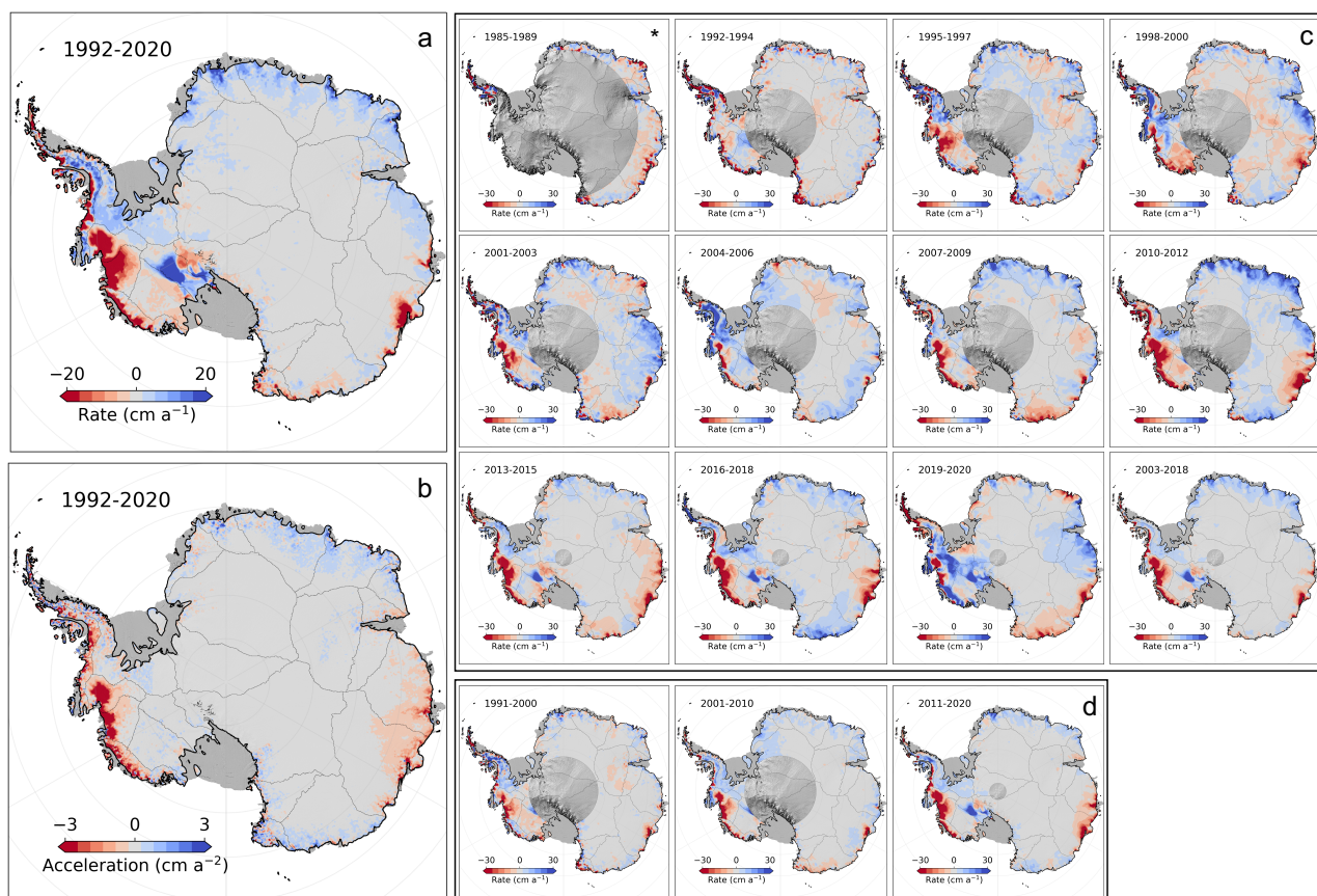
Figure 10. Rates of Antarctic Ice Sheet elevation change. Elevation change rate (a) and acceleration (b) for the 1992-2020 period and average rates for (c) 3-year, (d) ICESat – ICESat-2 and (d) 10-year intervals. (*) indicates a five-year interval for Geosat.
