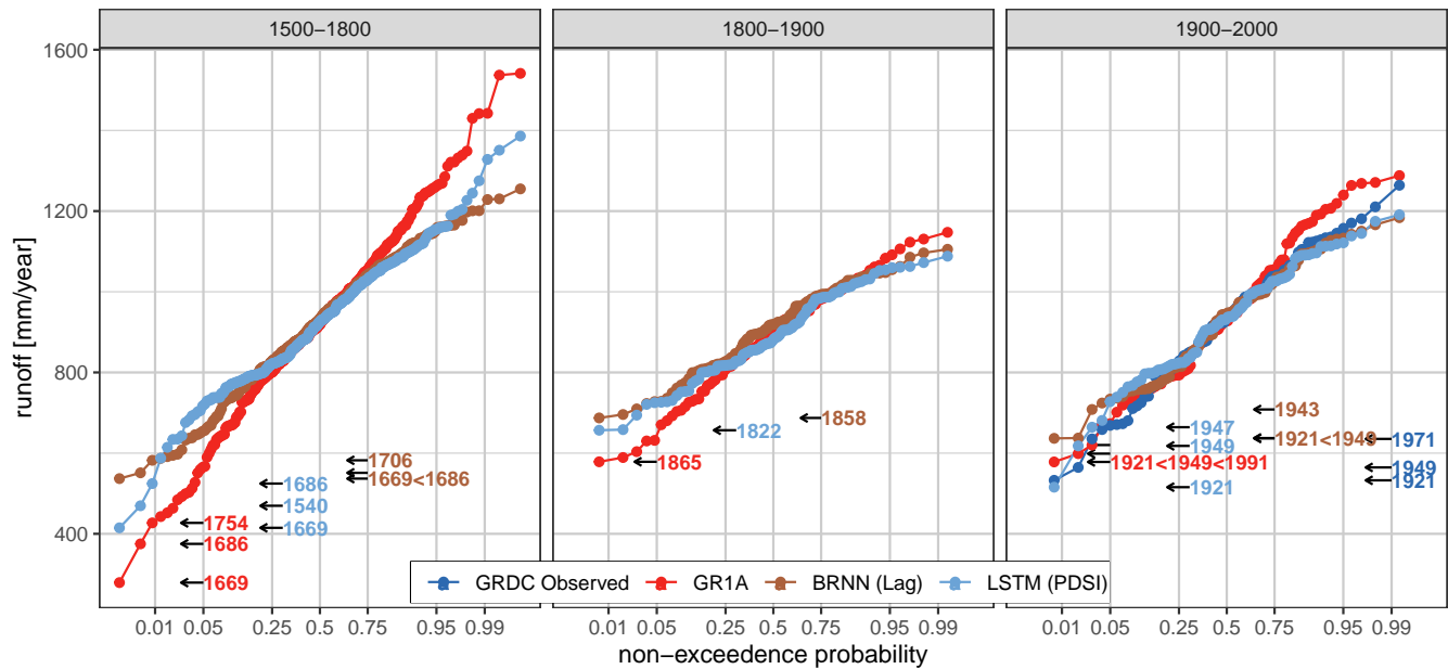
Figure 7. Distribution functions for BRNN(Lag), LSTM(PDSI), i.e. the best two models, GR1A and observed data (OBS) for the periods 1500–1800, 1800–1900 and 1900–2000 over Basel Rheinhalte-Rhine catchment. The values on the horizontal axis are transformed using the “probit” function. The colored labels indicate the most extreme drought years according to each model.
