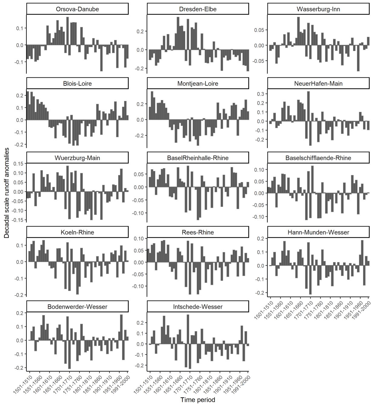
Figure A2. Decadal fluctuation of runoff anomalies in selected catchments over the past 500 years.
