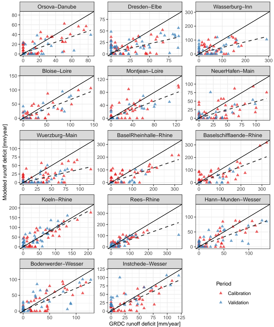
Figure 9. The observed and simulated runoff deficit based on the 33rd percentile threshold for 14 selected catchments during the calibration and validation period. The solid line represents the 1:1 relation, the dashed line corresponds to fitted regression between observed and simulated runoff.
