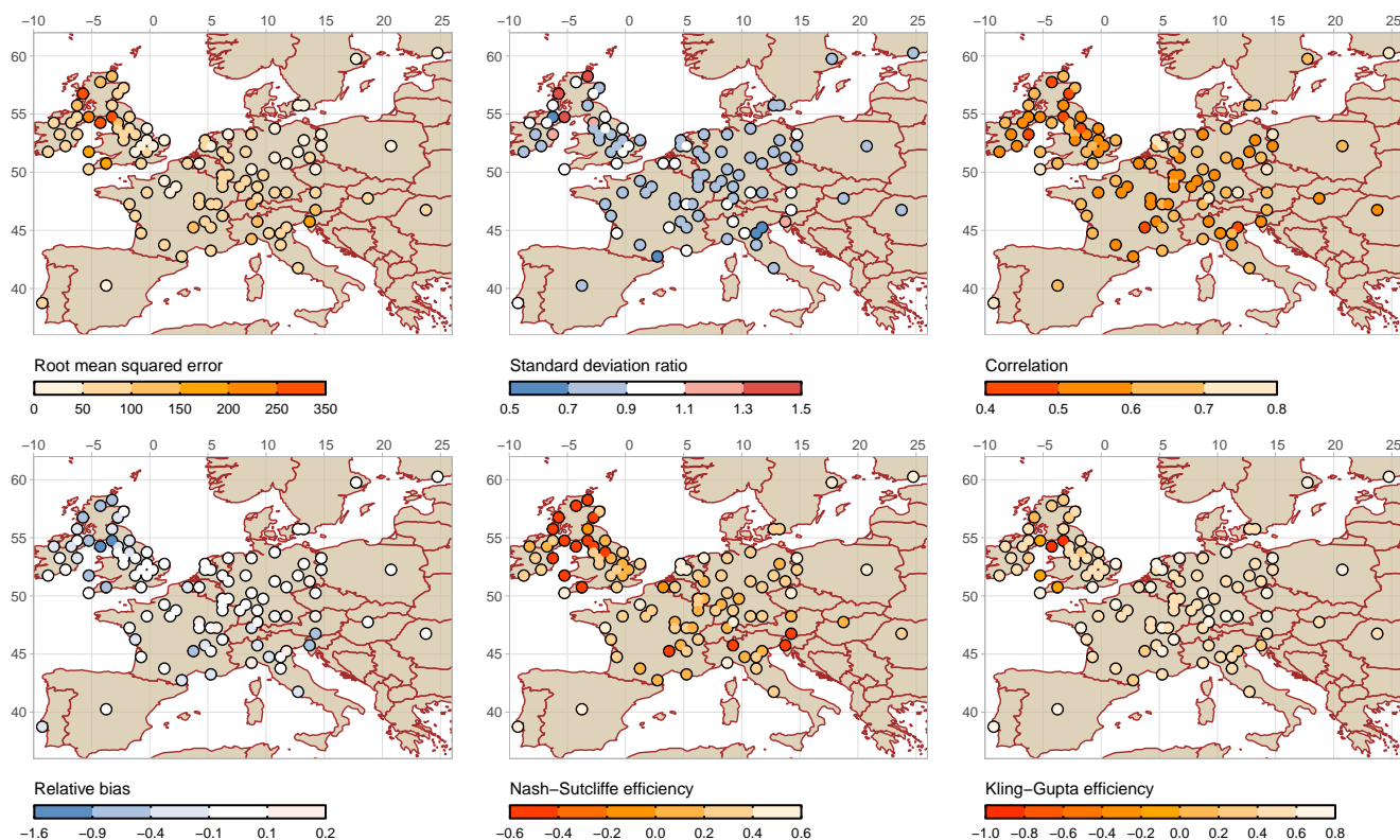
Figure 3. Validation of reconstructed precipitation (Pauling et al., 2006) against GHCN observations. The left and right most figures represent the approximate minimum and maximum for the corresponding indicator.
