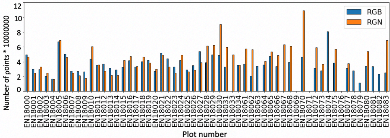
385 Figure 11: Comparison of the number of points in Red Green Near infrared (RGN; orange bars) and the combination of the two Red Green Blue (RGB) ‘groundonly’ and ‘treesonly’ point clouds (RGB; blue bars).
