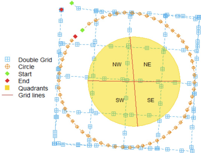
665 Figure A4: SiDroForest unmanned aerial vehicle (UAV) data acquisition and flight pattern consisting of a double grid (blue) and a circular mission (orange). The two 15 m long grid lines (red) divide the plot area into four quadrants of similar size (yellow). From Brieger et al. (2019).
