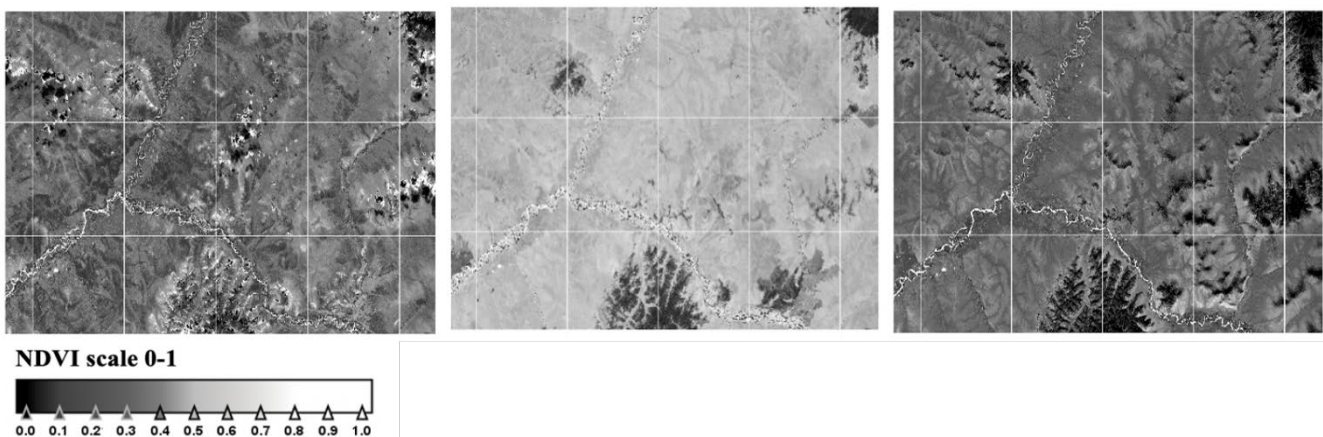
Figure 10: Sentinel-2 NDVI in greyscale of the three periods for the Bilibino subregion in Chukotka. Left: early summer, centre: peak summer, and right: late summer.
