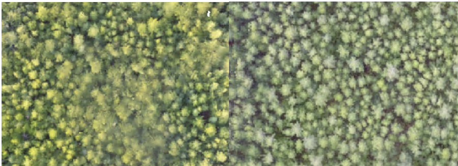
580 Figure 22: Dense forest Red Green Blue (RGB) orthomosaics for plots EN18077 and EN18063 .
