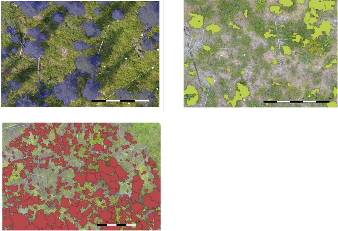
Figure 14: Top left: Crown polygons for plot EN18014 with Q1 quality score. Top right: Crown polygons for plot EN18014 with Q2 quality score. Bottom: Crown polygons for plot EN18014 with Q3 quality score. The scale bar represents 10 meters.
