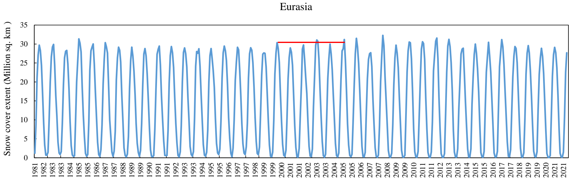
Figure 2. Monthly snow cover extent over the Eurasia
