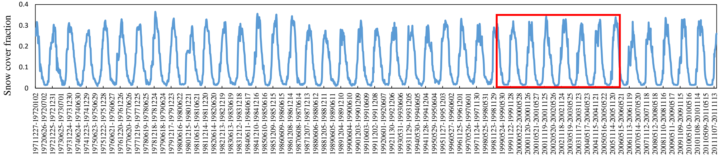
Snow cover fraction in Europe (longitude:-30-55 degree, latitude:30.0-75.0 degree)
