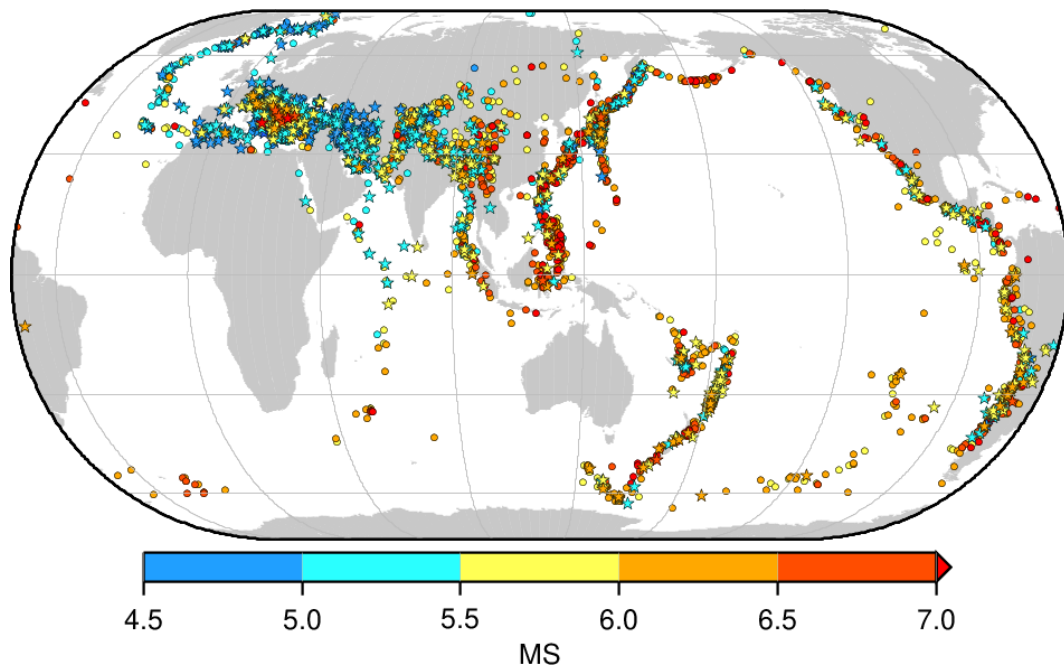
Figure 9. Map of the pre-1964 earthquakes where the expansion of the delta-period ranges compared to the current ISC practice allowed us to better constrain M_S . Stars are for the 1,000 earthquakes that otherwise would not have network M_S . All symbols colour-coded by M_S . Map drawn using the Generic Mapping Tools (GMT) (Wessel et al., 2013) software.
