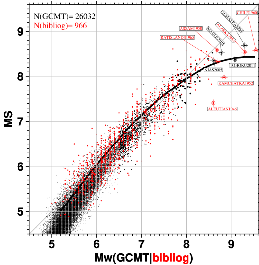
Figure 12. Comparison of MS with M_w from GCMT (black dots) and from the literature (red, Lee and Engdahl, 2015, and further updates listed at www.isc.ac.uk/iscgem/mw_bibliography.php , last access: August 2021). The black solid curve is a digitized version of the mid-point M_w - MS curve shown in Figure 4b of Kanamori (1983). The largest 10 earthquakes in terms of M_w (bulls eye symbols) are also identified by the event code in the ISC Event Bibliography ( www.isc.ac.uk/event_bibliography/index.php , last access: August 2021).
