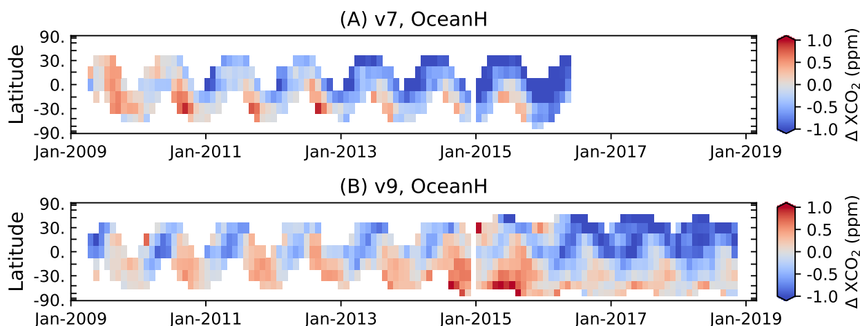
Figure 11. Time series of \Delta\text{XCO}_2^{\text{MMM}} (ACOS GOSAT v9 - MMM) versus latitude at 30 day by 15^\circ resolution for Ocean-Glint observations for v7.3 (A) and v9 (B). Grid cells containing less than 10 collocations are colored white.
