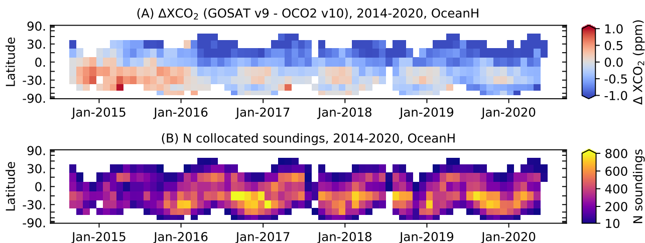
Figure 15. Difference in XCO 2 between ACOS GOSAT v9 and OCO-2 v10 ( \Delta XCO_2^{OCO-2} ) as a function of time and latitude at 30 day by 15° latitude resolution for Ocean-Glint observations (panel A). Panel (B) shows the sounding density of the collocated soundings. Grid cells containing less than 10 collocations are colored white.
