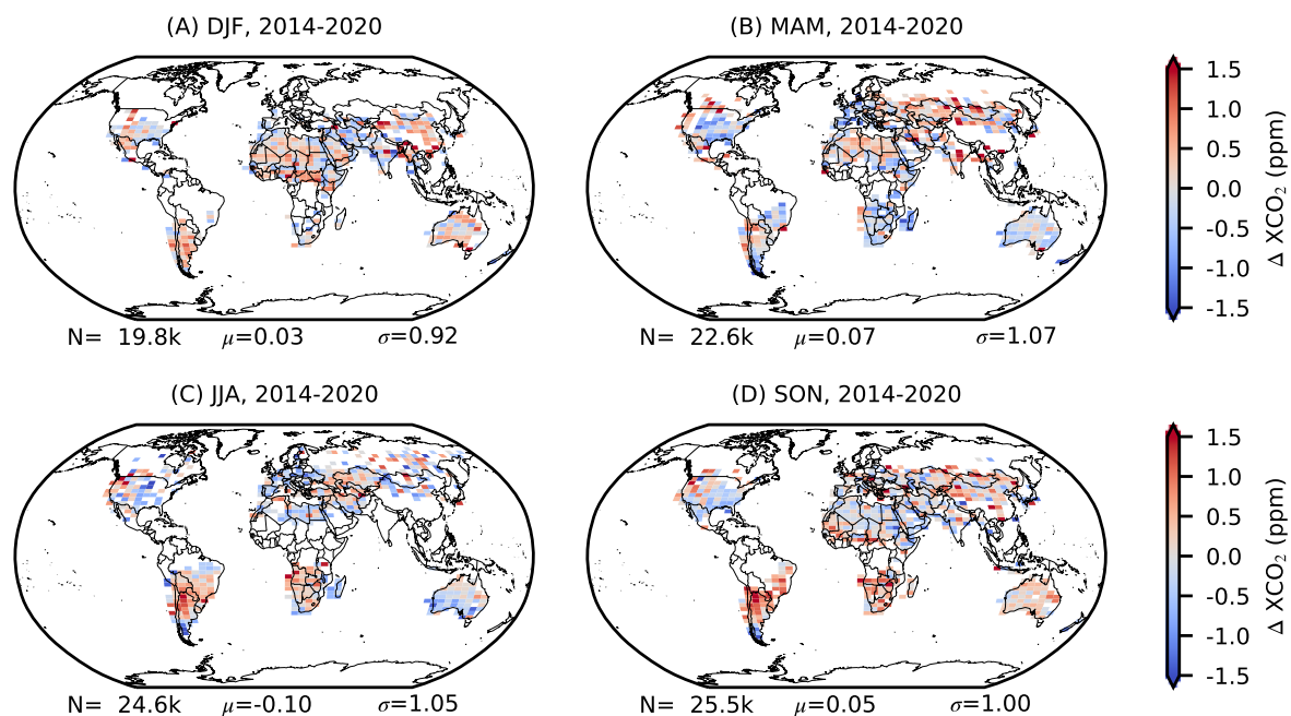
Figure 13. Spatial distribution of the bias corrected \Delta XCO_2^{OCO-2} (GOSAT v9 minus OCO-2 v10) for the good QF land soundings for DJF (A), MAM (B), JJA (C), and SON (D) for the overlapping period August 2014 through June 2020. The spatio-temporal requirements for matched soundings are a maximum separation of 300 km, and observation time within \pm 2 hours. Maps are gridded at 2.5^\circ latitude by 5^\circ longitude resolution, and only grid boxes with at least 10 matched soundings are shown.
