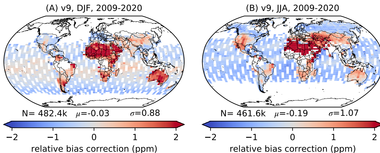
Figure 2. Maps of ACOS GOSAT v9 relative bias correction for DJF (A) and JJA (B) for good QF soundings in the eleven year data record at 2.5^\circ by 5^\circ latitude/longitude, after removal of the global, median bias of -1.8 ppm. Grid cells with less than 5 GOSAT soundings are not colored. The total number of soundings (N), and the mean bias ( \mu ) and standard deviation of the bias ( \sigma ) in each grid cell are given.
