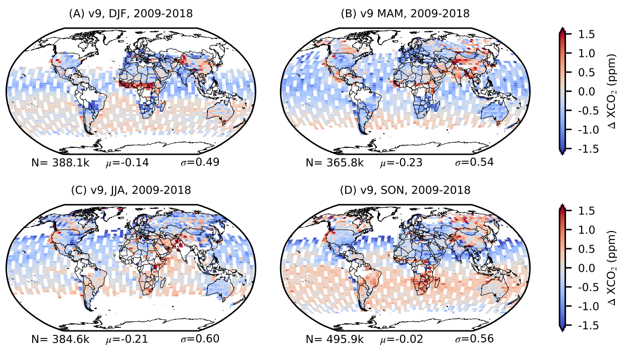
Figure 10. Seasonal maps of the mean \Delta XCO_2^{MMM} (GOSAT - MMM) spanning 2009 through 2018 for DJF (A), MAM (B), JJA (C), and SON (D) at 2.5° latitude by 5° longitude resolution. Grid boxes containing less than 10 collocations are colored white.
