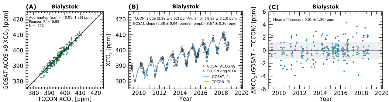
Figure A3. Same as Figure A1, but for Bialystok, Poland.
