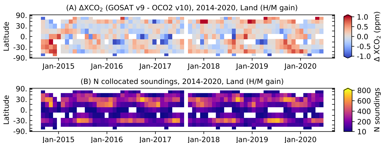
Figure 16. Same as Figure 15, but for land observations (combined H-gain and M-gain).
