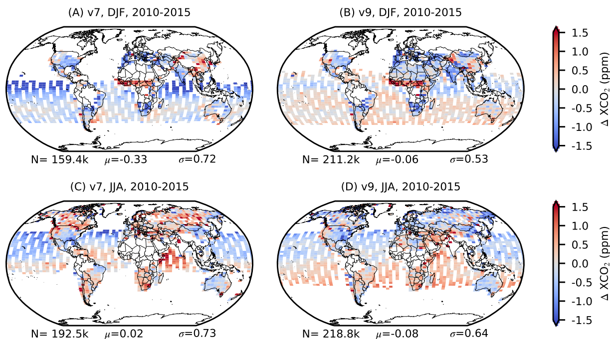
Figure 12. Maps of the mean \Delta XCO_2^{MMM} (GOSAT - MMM) spanning 2010 through 2015 for v7.3 DJF (A), v9 DJF (B), v7.3 JJA (C), and v9 JJA (D) at 2.5° by 5° latitude/longitude resolution. Only grid boxes with at least 10 collocations are shown.
