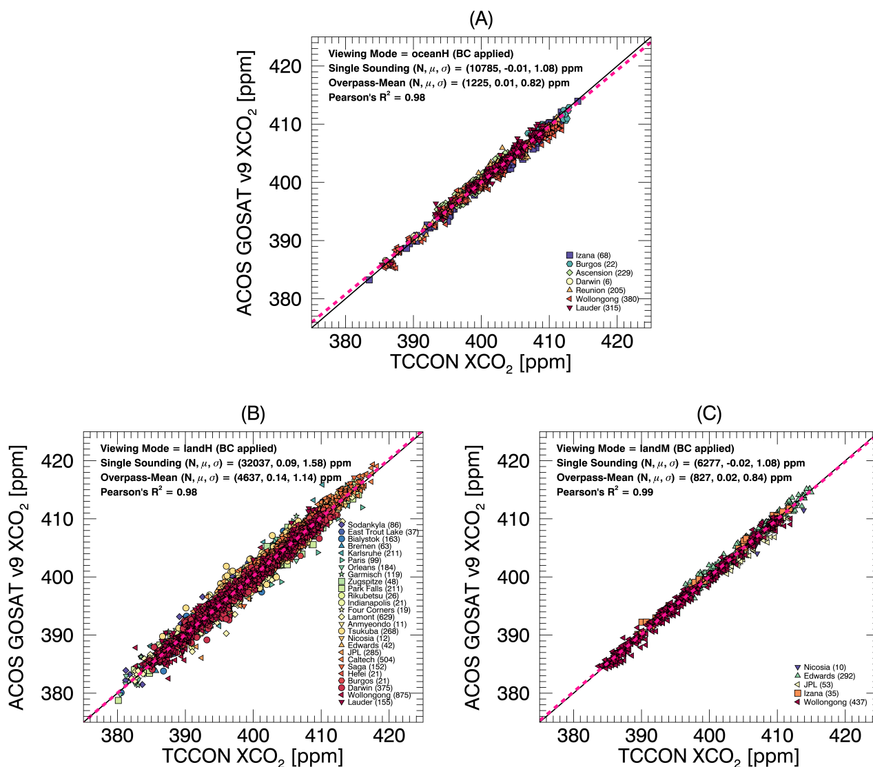
Figure 7. Quality filtered and bias corrected ACOS GOSAT v9 vs collocated TCCON XCO 2 for Ocean-Glint (A), Land H-gain (B), and Land M-gain (C). Each point represents an overpass mean, which typically contain 5-10 GOSAT soundings per overpass. The legend in the lower right indicates the number of collocated overpass means for individual TCCON stations. Summary statistics for all stations combined are reported in the upper left of each panel for both single sounding and overpass means.
