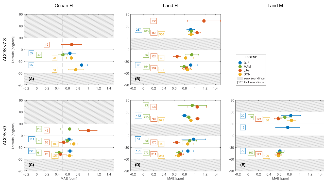
Figure 8. Mean Absolute Error (MAE; ppm) between ACOS GOSAT v9 XCO 2 and collocated TCCON observations for v7.3 (panels A and B) and v9 (panels C, D and E), binned by latitude for: Ocean-Glint (panels A and C), Land H-gain (panels B and D) and Land M-gain (panel E). Recall that there was no Land M-gain data generated for v7.3. The error bars on the MAE represent the standard error of the mean. The calculation of the MAE statistic and error bars follow the procedure reported in Chatterjee et al. (2013) (Equations 3 and 4). The total number of independent observations available within each latitude band and for each season are reported in the colored boxes. Latitude bands that do not have any collocated soundings are shaded in grey.
