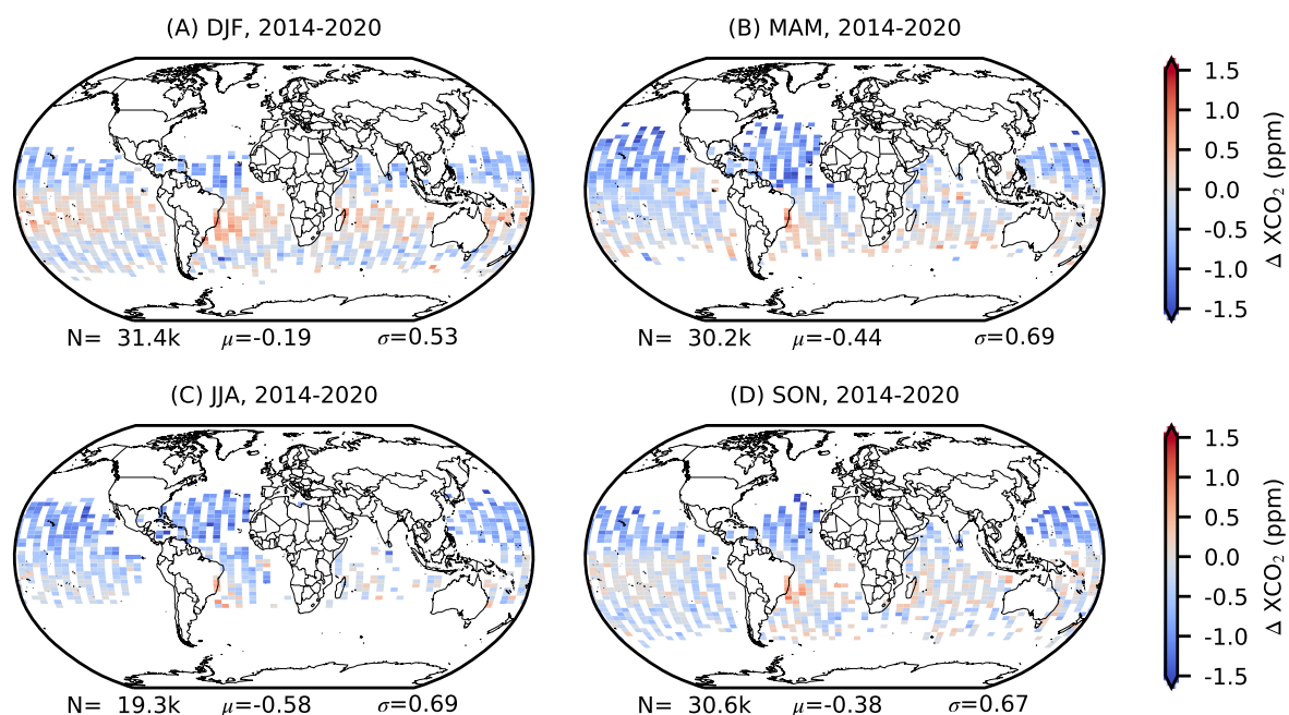
Figure 14. Same as Figure 13, but for Ocean-Glint observations.
