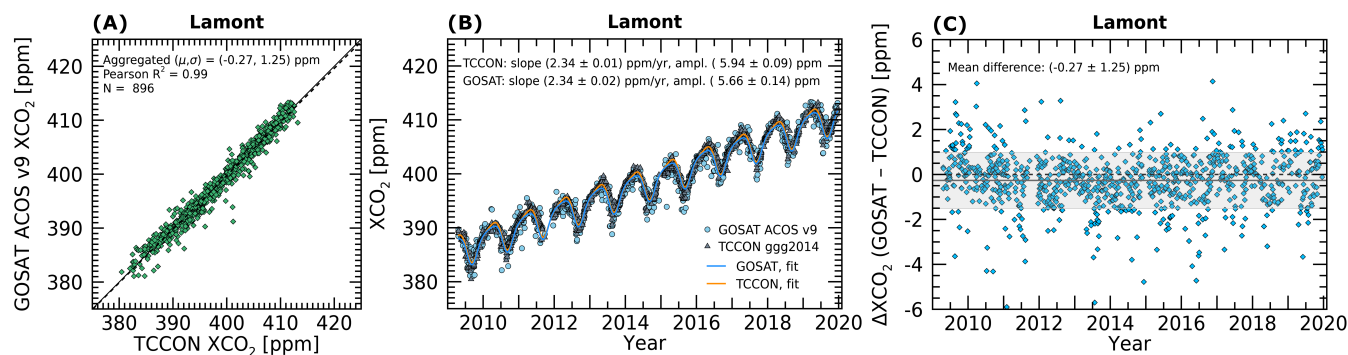
Figure 9. Seasonal cycle analysis of ACOS GOSAT v9 XCO 2 versus collocated TCCON for the Lamont, Oklahoma station, following the methodology of Lindqvist et al. (2015). Panel (A) shows the one-to-one scatter plot of the bias corrected daily mean XCO 2 for GOSAT versus TCCON. Panel (B) shows the time series of GOSAT XCO 2 (blue circles) with fit (blue line) and the TCCON XCO 2 (grey triangles) with fit (orange line) over the eleven year data record. Panel (C) shows the time series of calculated \Delta XCO_2^{TCCON} (GOSAT - TCCON), with the mean difference (horizontal solid black line) and \pm 1 standard deviation (gray shading). The three GOSAT observation modes have been combined into daily mean averages to provide the maximum number of collocations possible for the seasonal fits.
