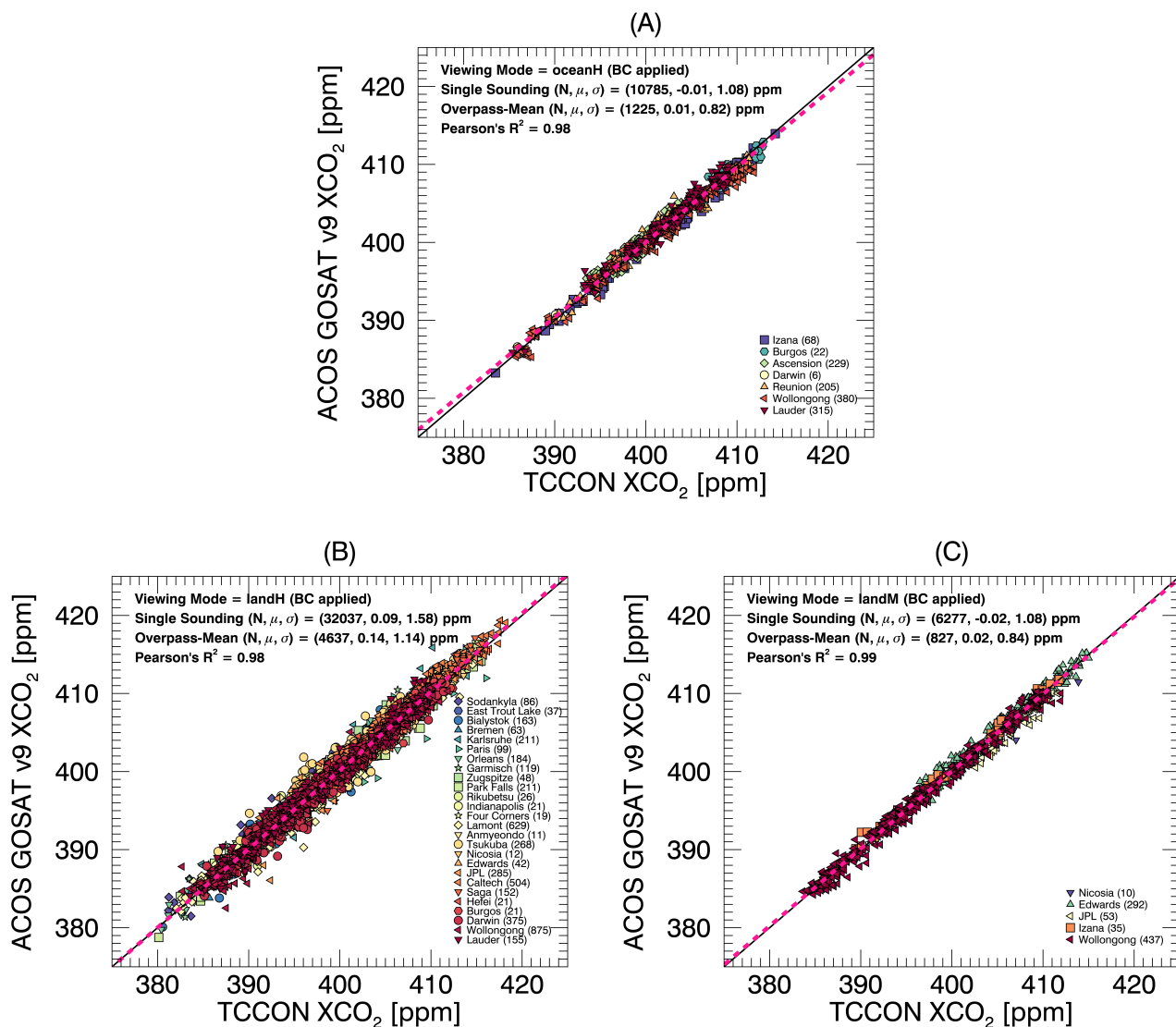
Figure 8. Quality filtered and bias corrected ACOS GOSAT v9 vs colocated TCCON XCO_2 for Ocean-Glint (A), Land H-gain (B), and Land M-gain (C). Each point represents an overpass mean, which typically contain 5-10 GOSAT soundings per overpass. The legend in the lower right indicates the number of colocated overpass means for individual TCCON stations. Summary statistics for all stations combined are reported in the upper left of each panel for both single sounding and overpass means.
