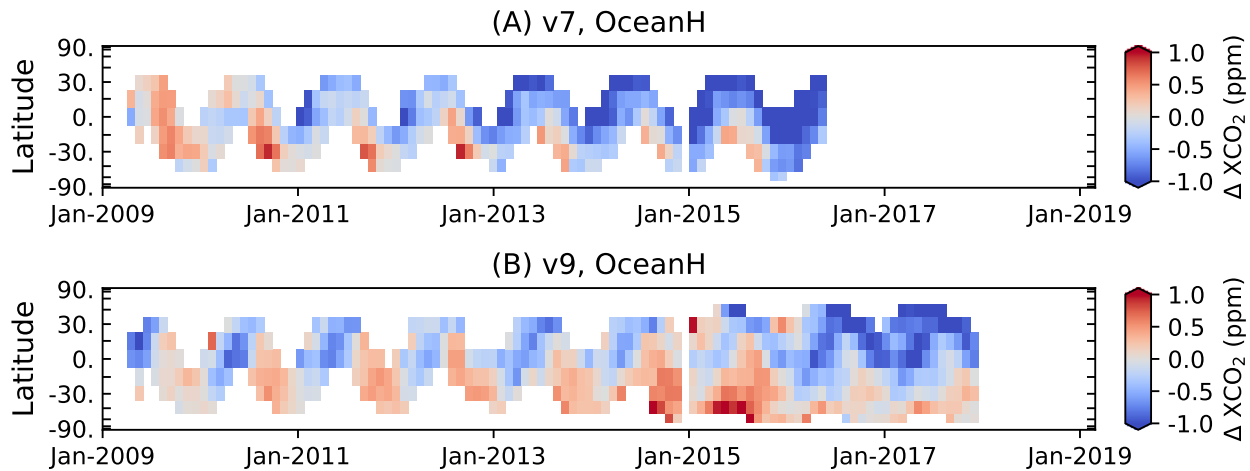
Figure 12. Time series of \Delta\text{XCO}_2^{\text{MMM}} (ACOS GOSAT v9 - MMM) versus latitude at 30 day by 15^\circ resolution for Ocean-Glint observations for v7.3 (A) and v9 (B). Grid cells containing less than 10 collocations are colored white.
