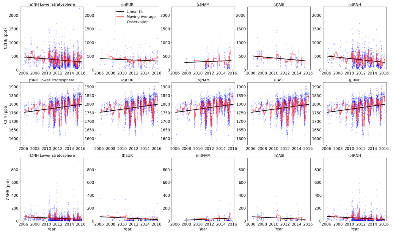
Figure 5. Lower stratospheric ethane, methane and propane mole fractions from observations and linear trends over five regions (whole NH lower stratosphere, EUR, NAM, ASI, and ROW RNH ).
