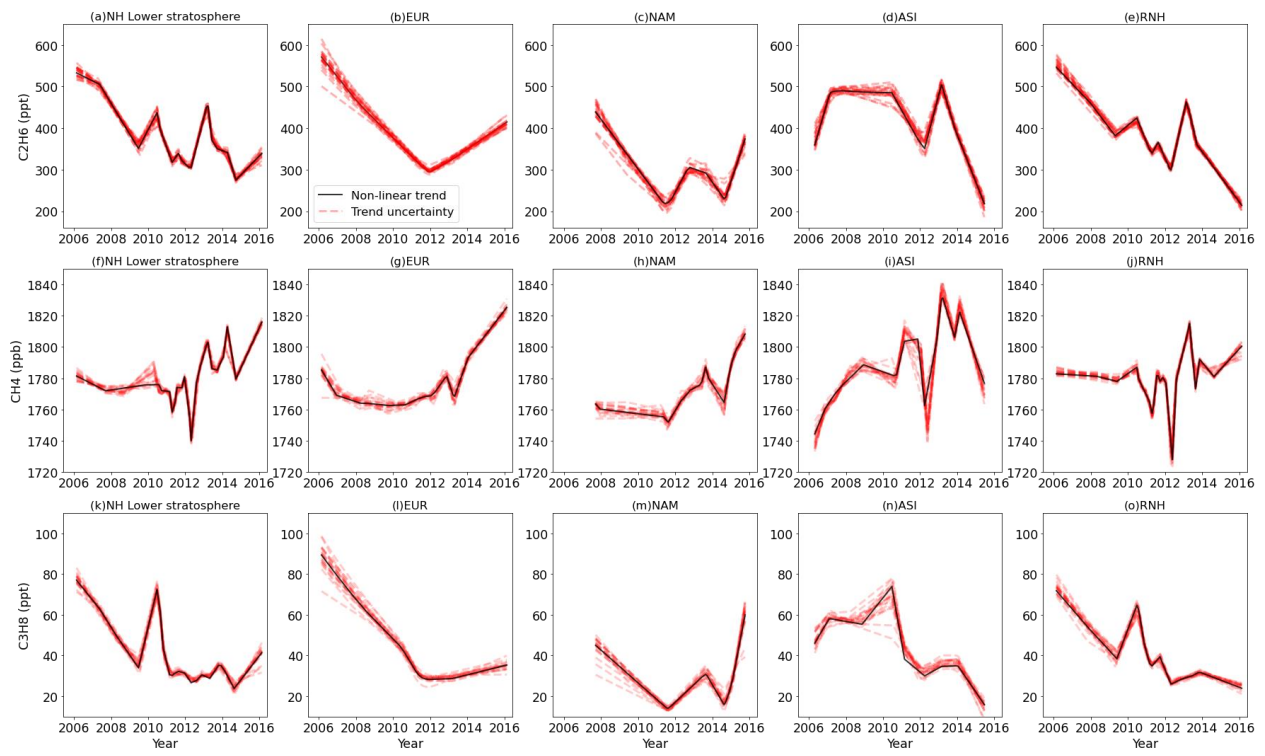
Figure 6. Non-linear trends of the lower stratospheric ethane, methane and propane over five regions (whole NH lower stratosphere, EUR, NAM, ASI, and ROW RNH ).
