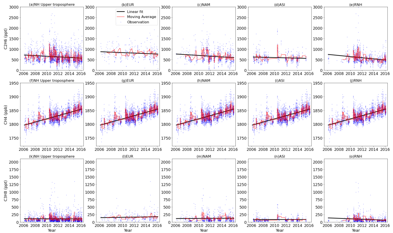
Figure 2. The upper tropospheric ethane, methane and propane mole fractions from observations and linear trends over five regions (whole NH upper troposphere, EUR, NAM, ASI, and
