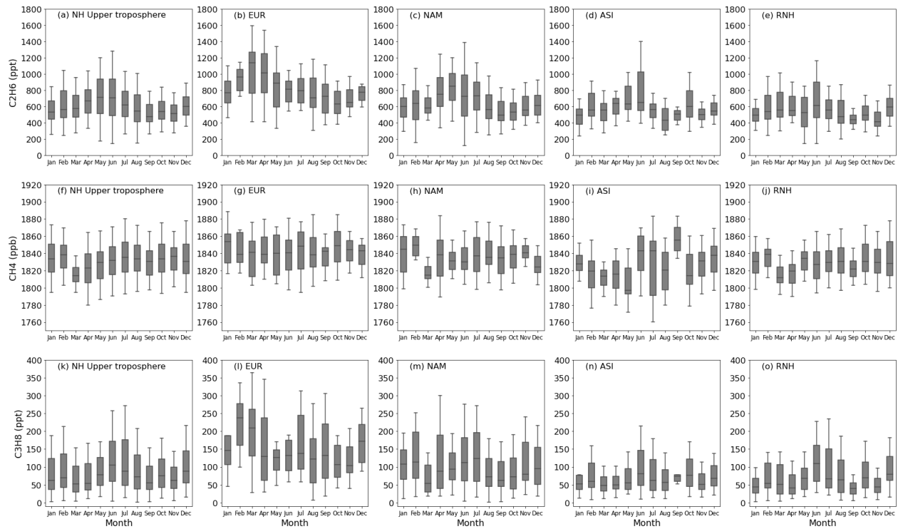
Figure 4. Monthly variations of the upper tropospheric ethane, methane and propane (2006-2016) over five regions (whole NH, EUR, NAM, ASI and ROW / RNH ). The boxes represent 25%-75% of all observed mole fractions, the horizontal lines in the boxes indicate the medians. The whiskers represent the 10%-90% range of all the observed mole fractions.
