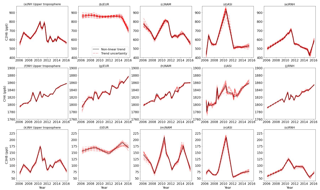
Figure 3. Non-linear trends of the upper tropospheric ethane, methane and propane over five regions (whole NH upper troposphere, EUR, NAM, ASI, and ROW RNH ).
